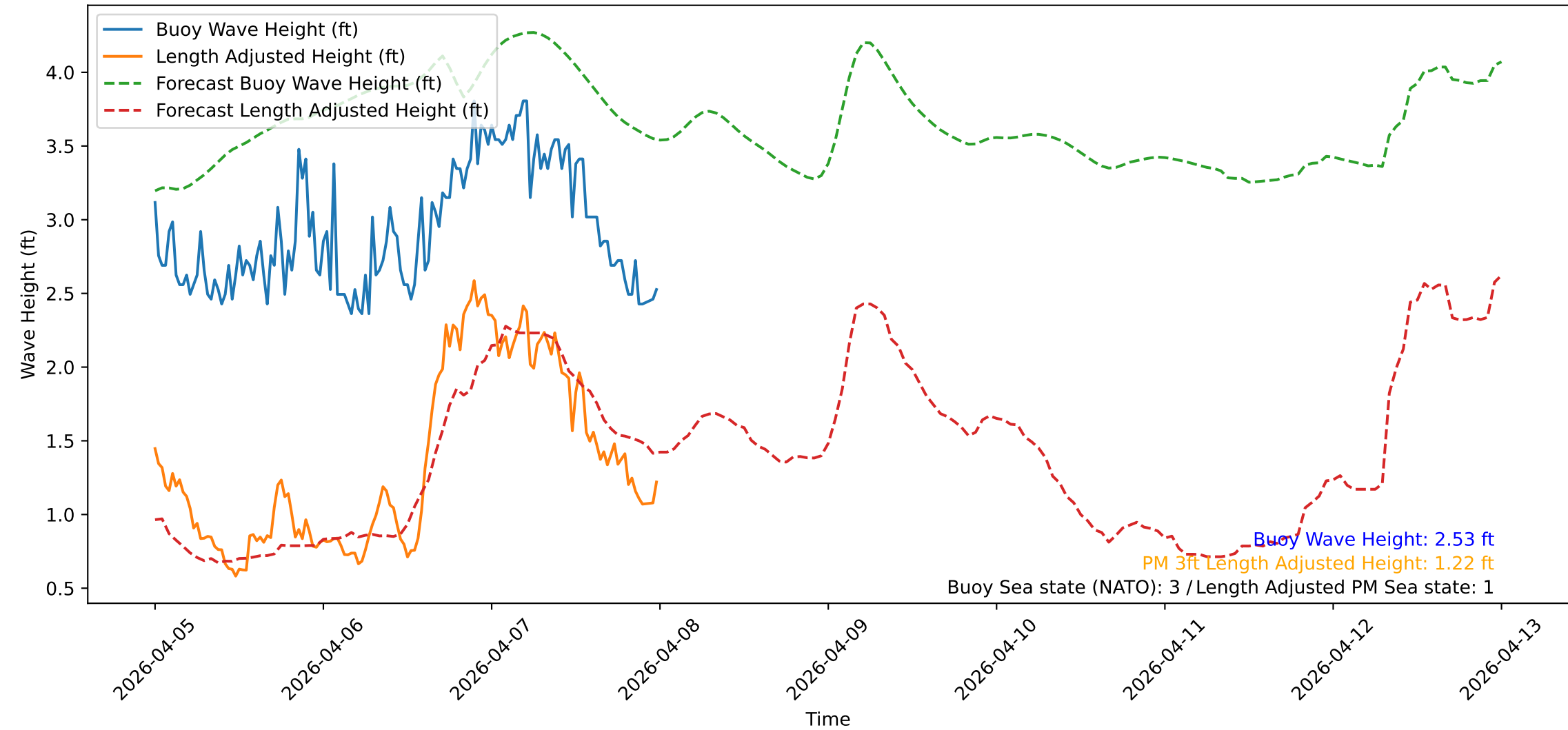
Wave Heights over Time for Green Beach at 2026-04-08 00:11:09
