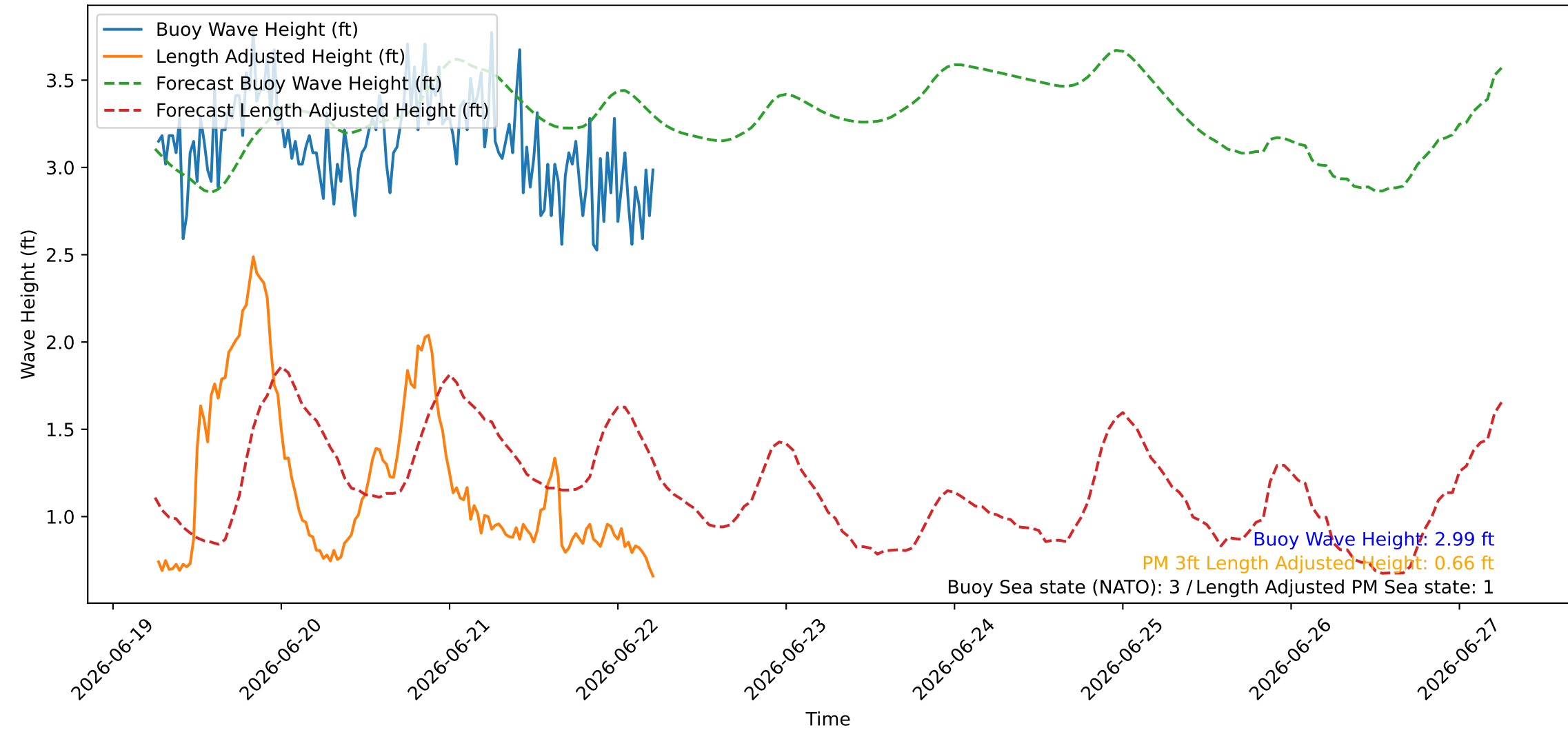
Wave Heights over Time for Red Beach at 2026-06-22 06:10:45
