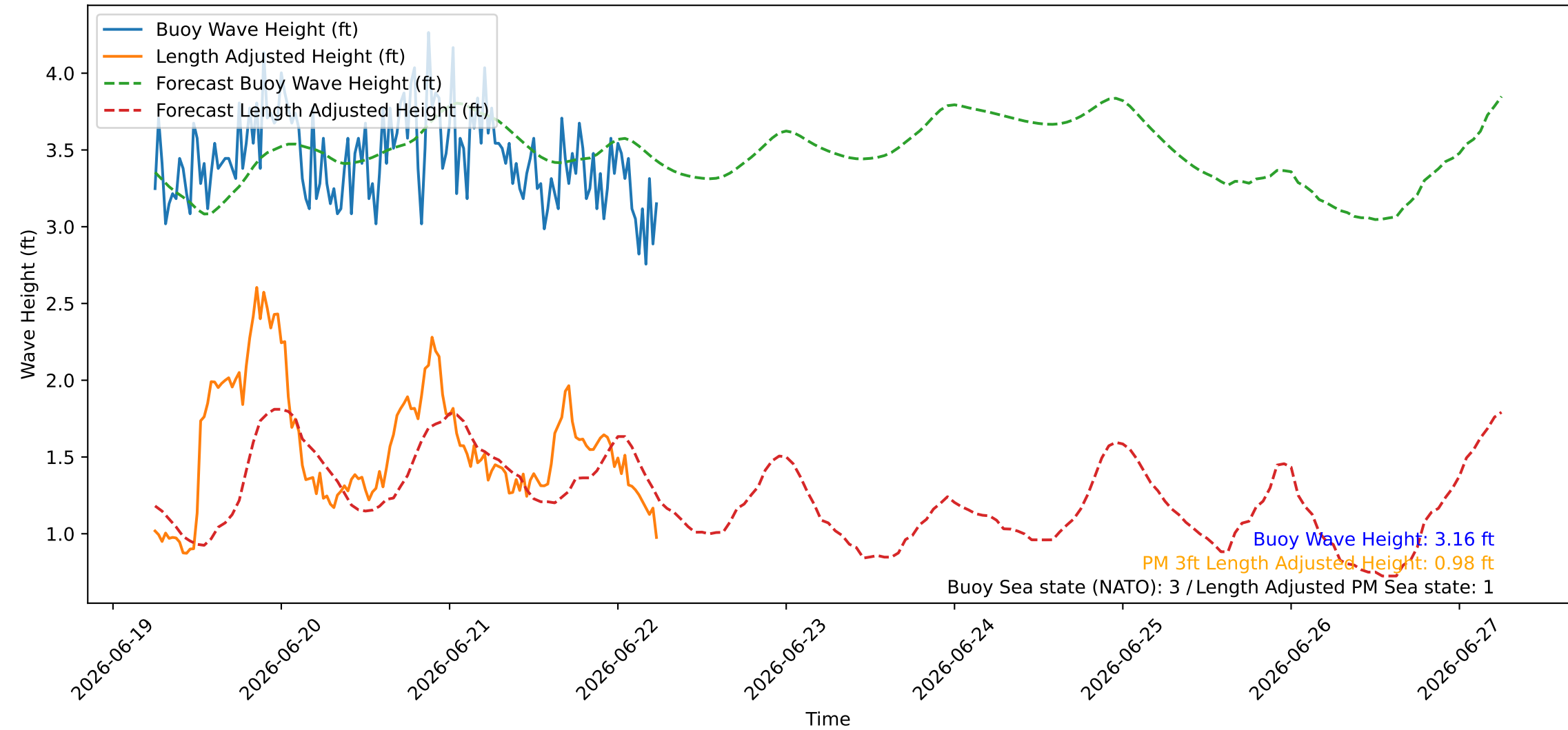
Wave Heights over Time for Oceanside Harbor at 2026-06-22 06:10:26
