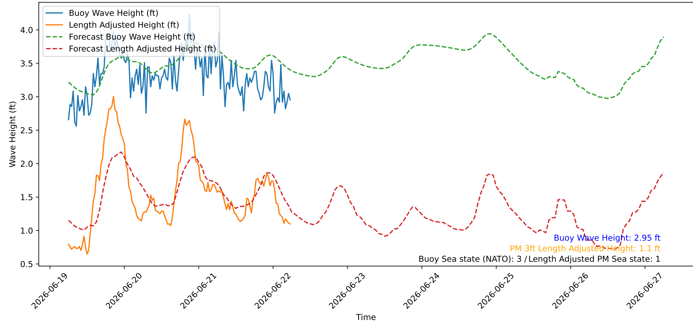
Wave Heights over Time for Green Beach at 2026-06-22 06:11:08
