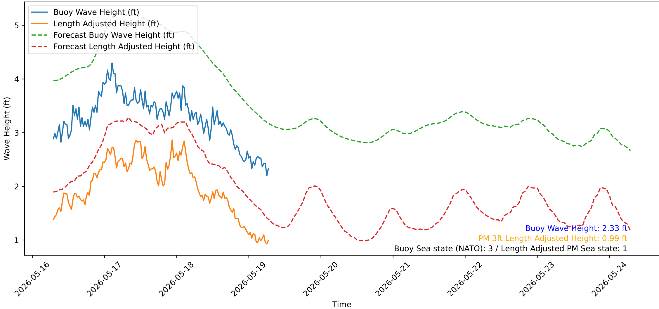
Wave Heights over Time for Oceanside Harbor at 2026-05-19 07:10:31
