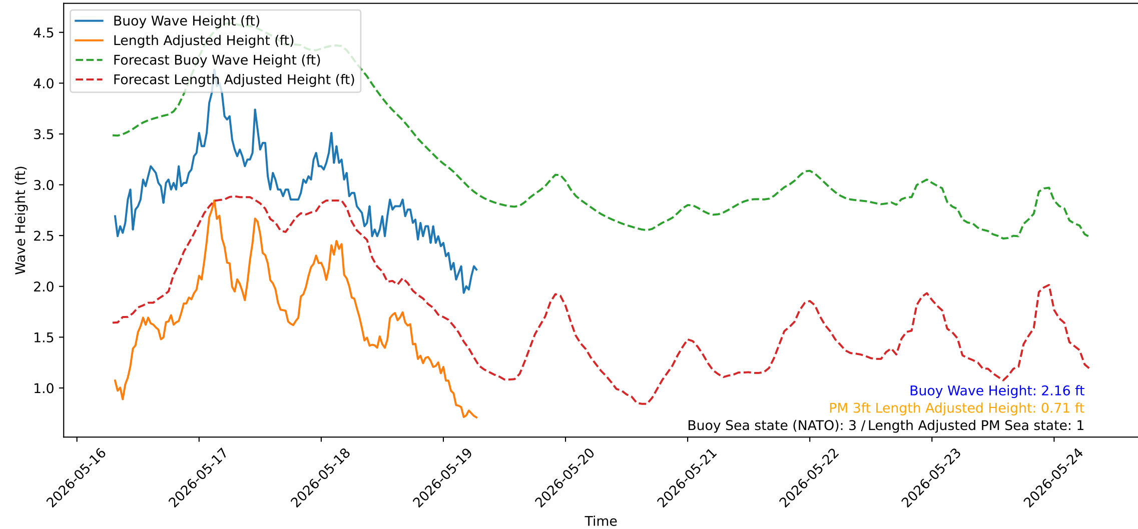
Wave Heights over Time for Red Beach at 2026-05-19 07:10:50
