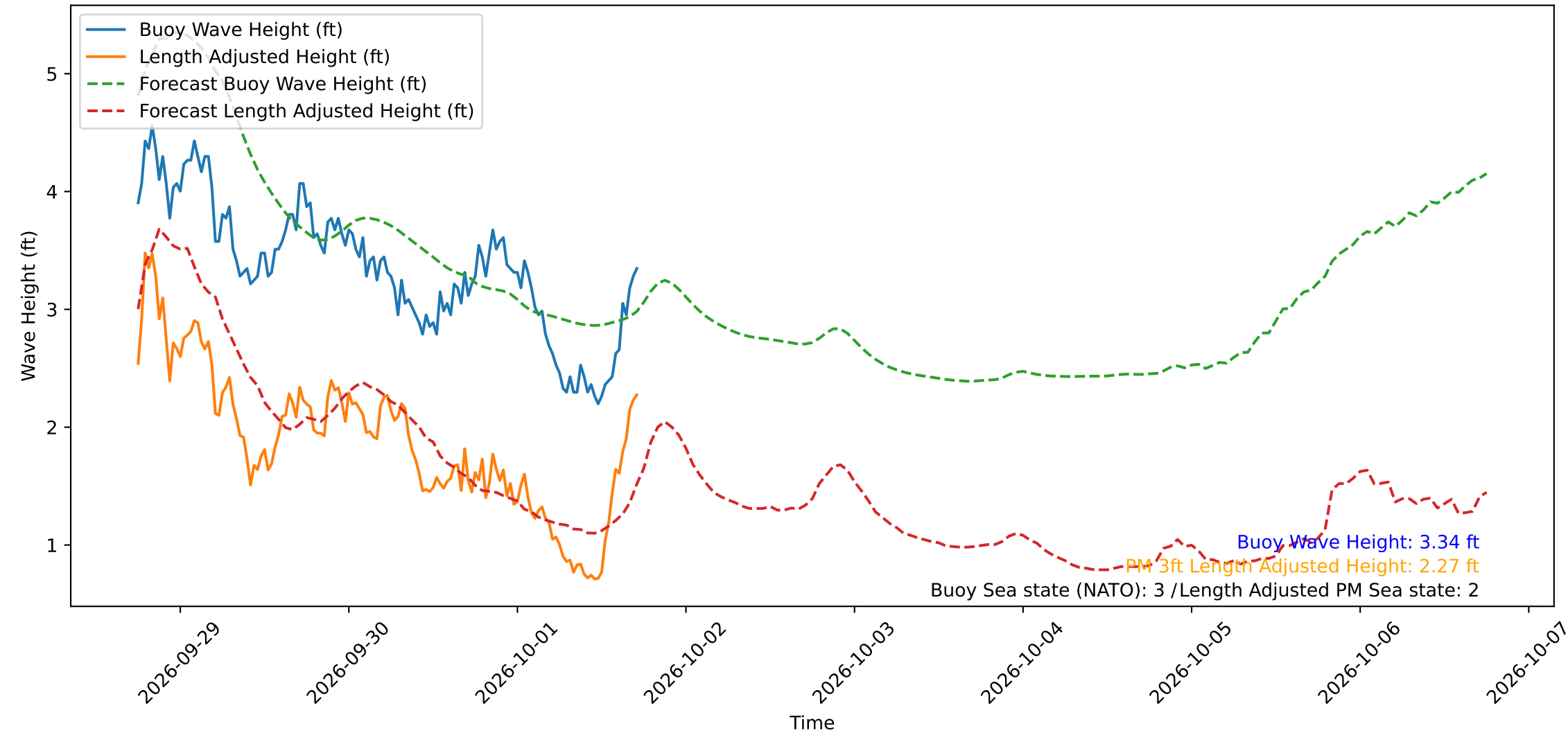
Wave Heights over Time for Green Beach at 2026-10-01 17:41:12
