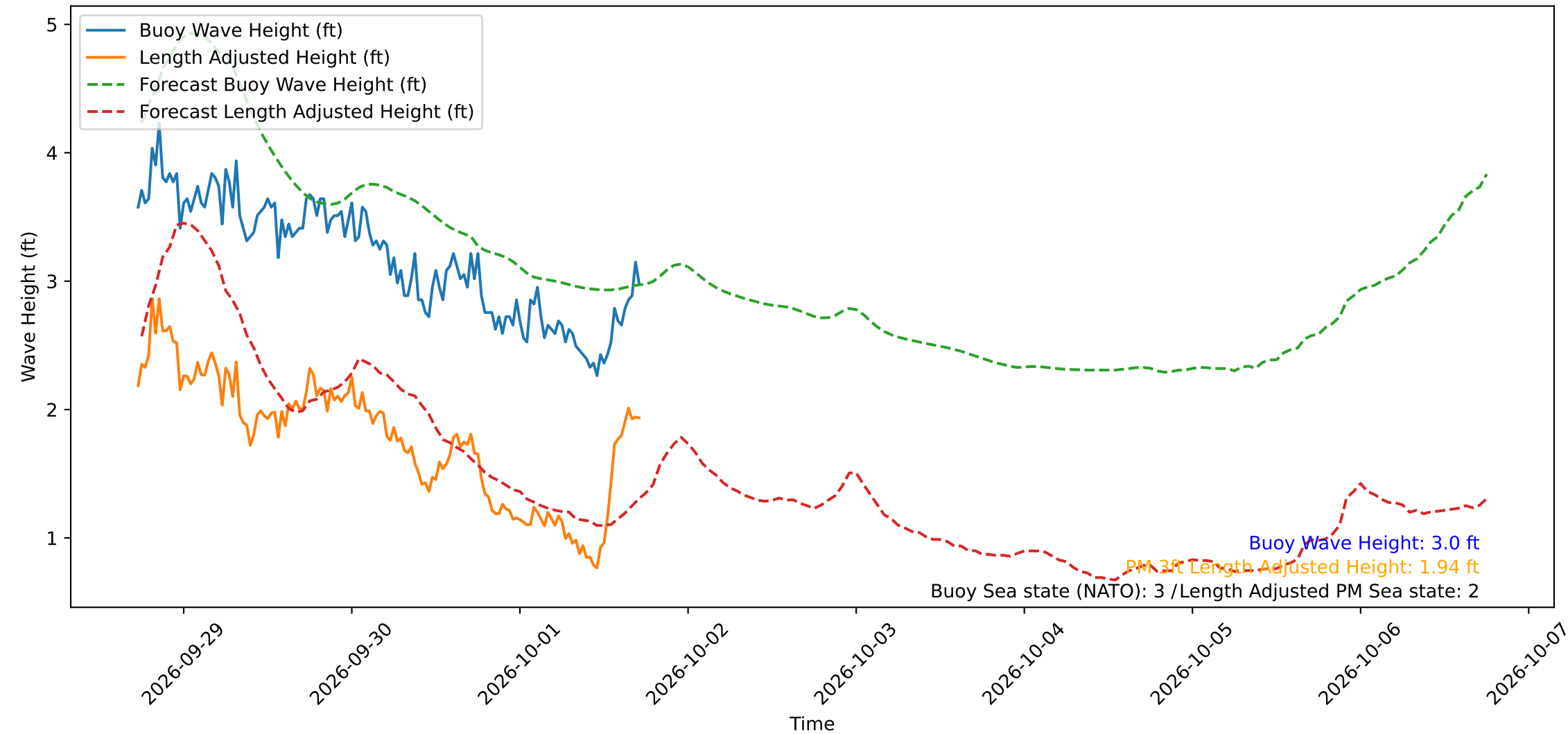
Wave Heights over Time for Oceanside Harbor at 2026-10-01 17:40:29
