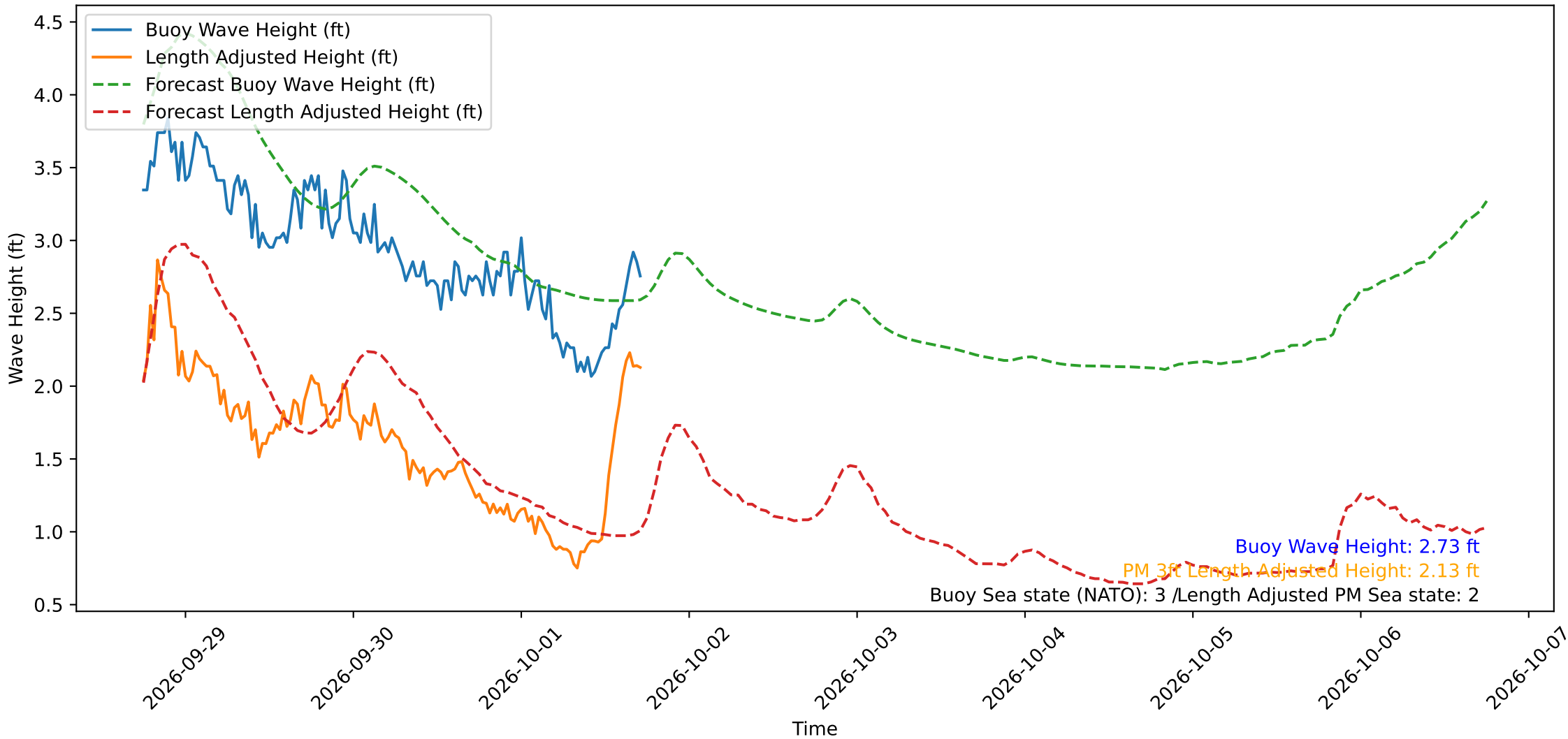
Wave Heights over Time for Red Beach at 2026-10-01 17:40:49
