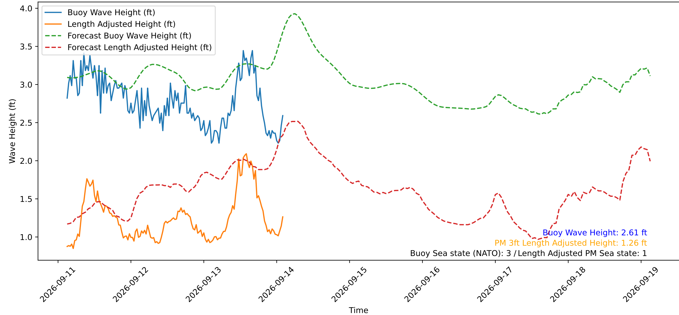
Wave Heights over Time for Red Beach at 2026-09-14 02:50:49
