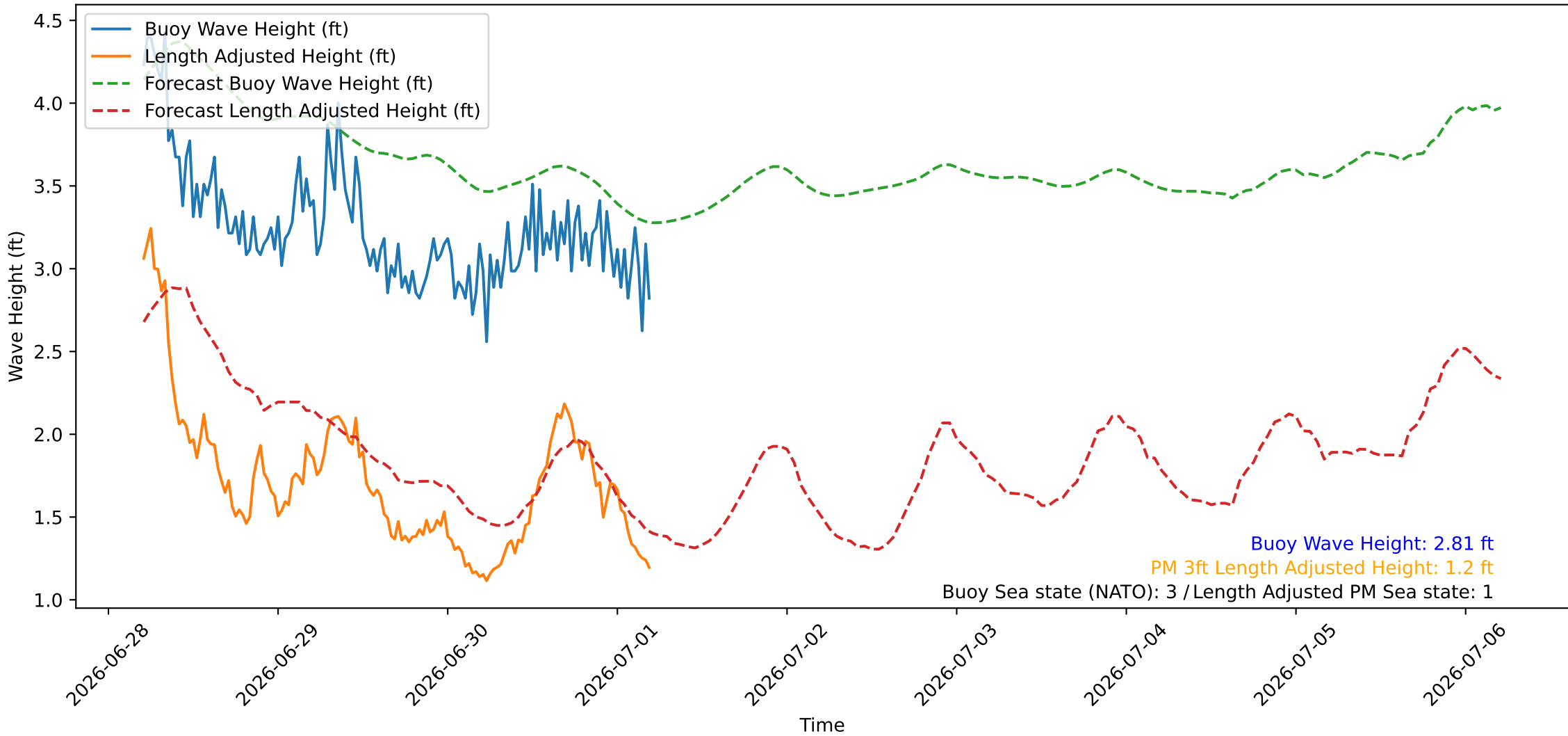
Wave Heights over Time for Oceanside Harbor at 2026-07-01 05:10:26
