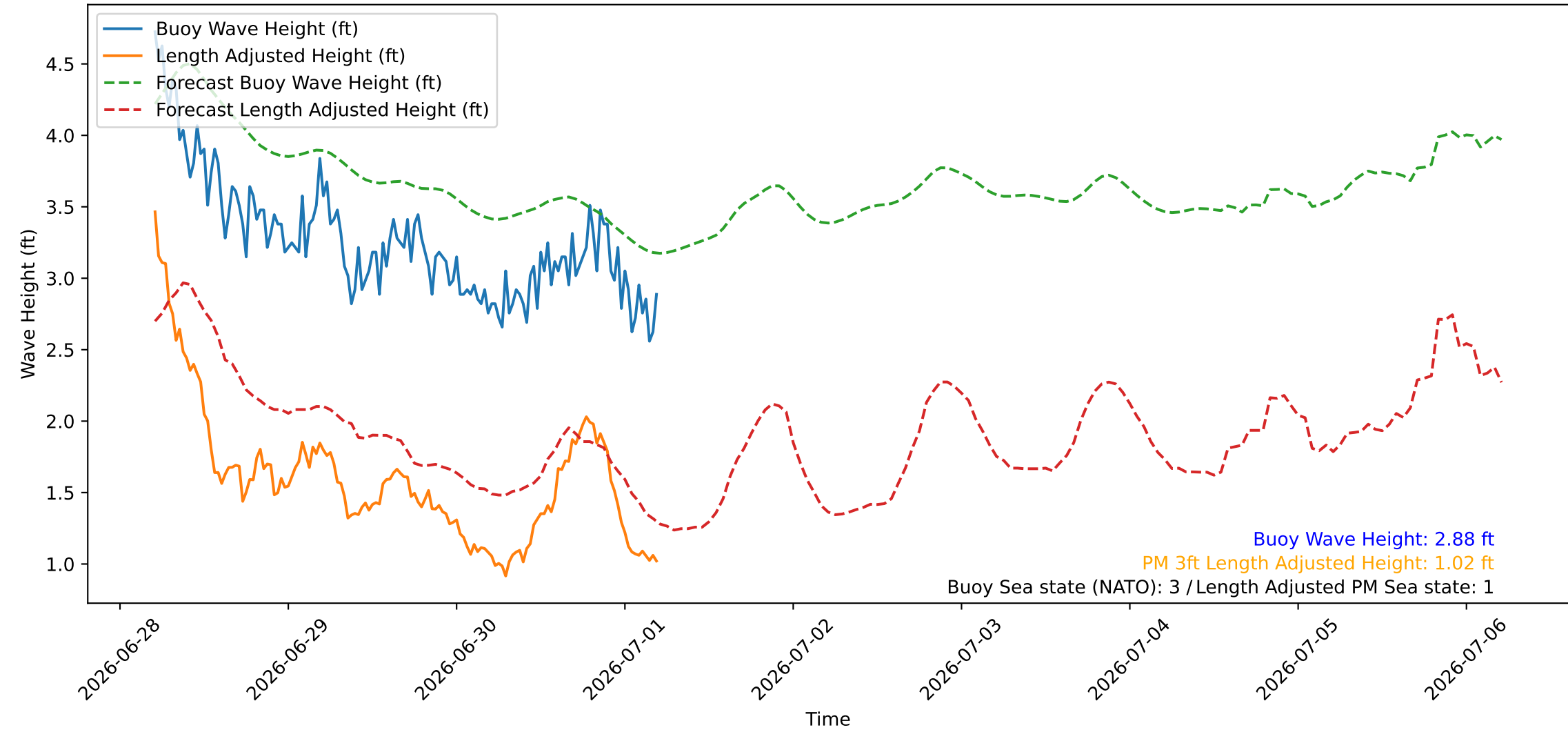
Wave Heights over Time for Green Beach at 2026-07-01 05:11:07
