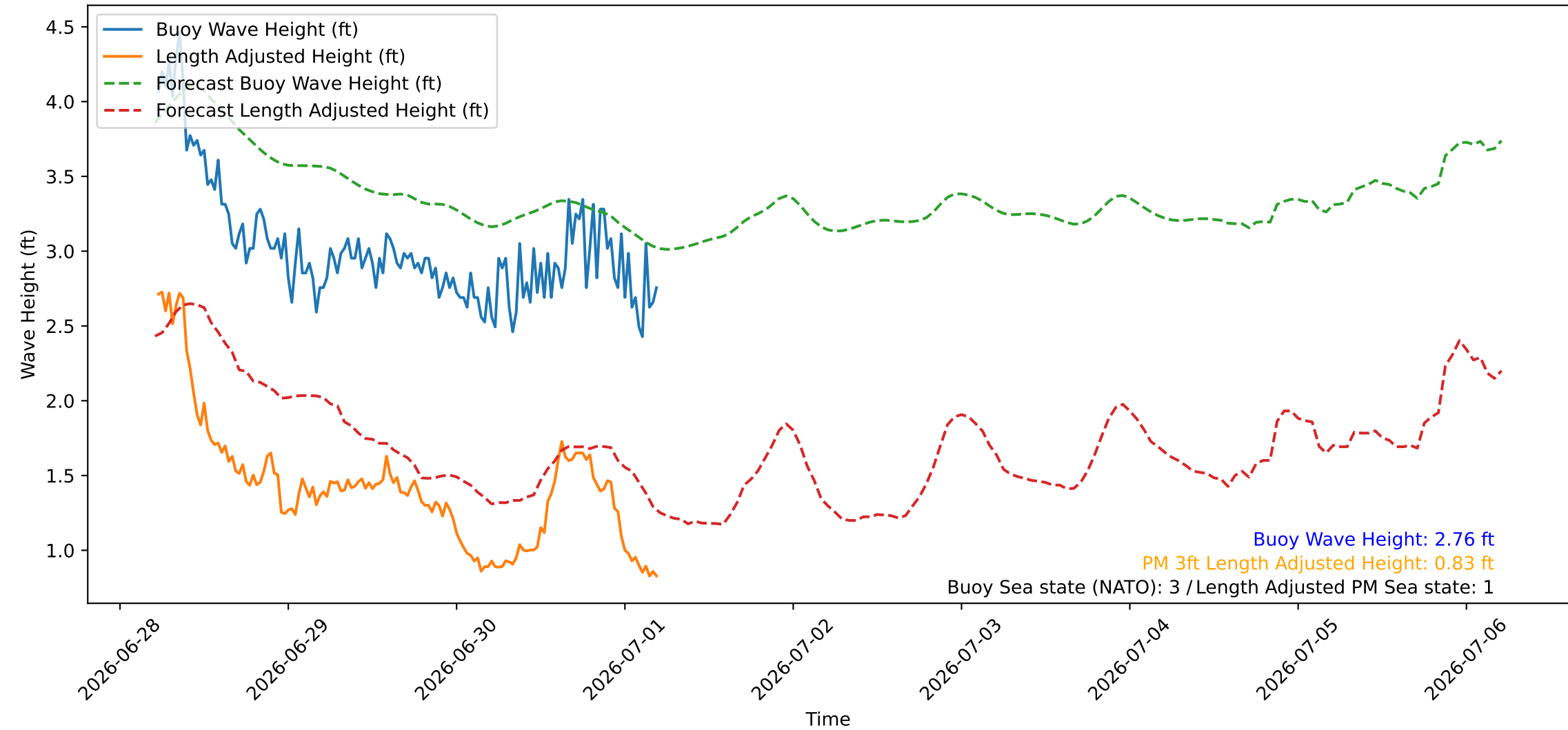
Wave Heights over Time for Red Beach at 2026-07-01 05:10:45
