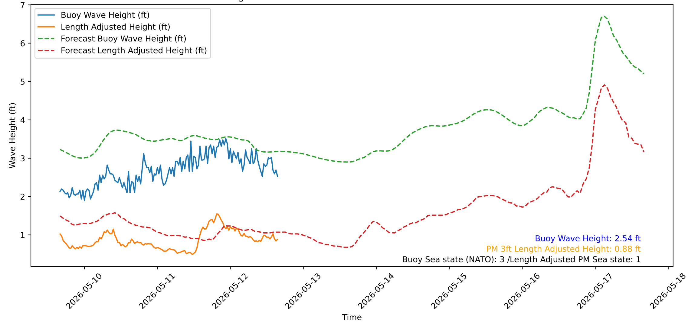
Wave Heights over Time for Green Beach at 2026-05-12 16:11:13
