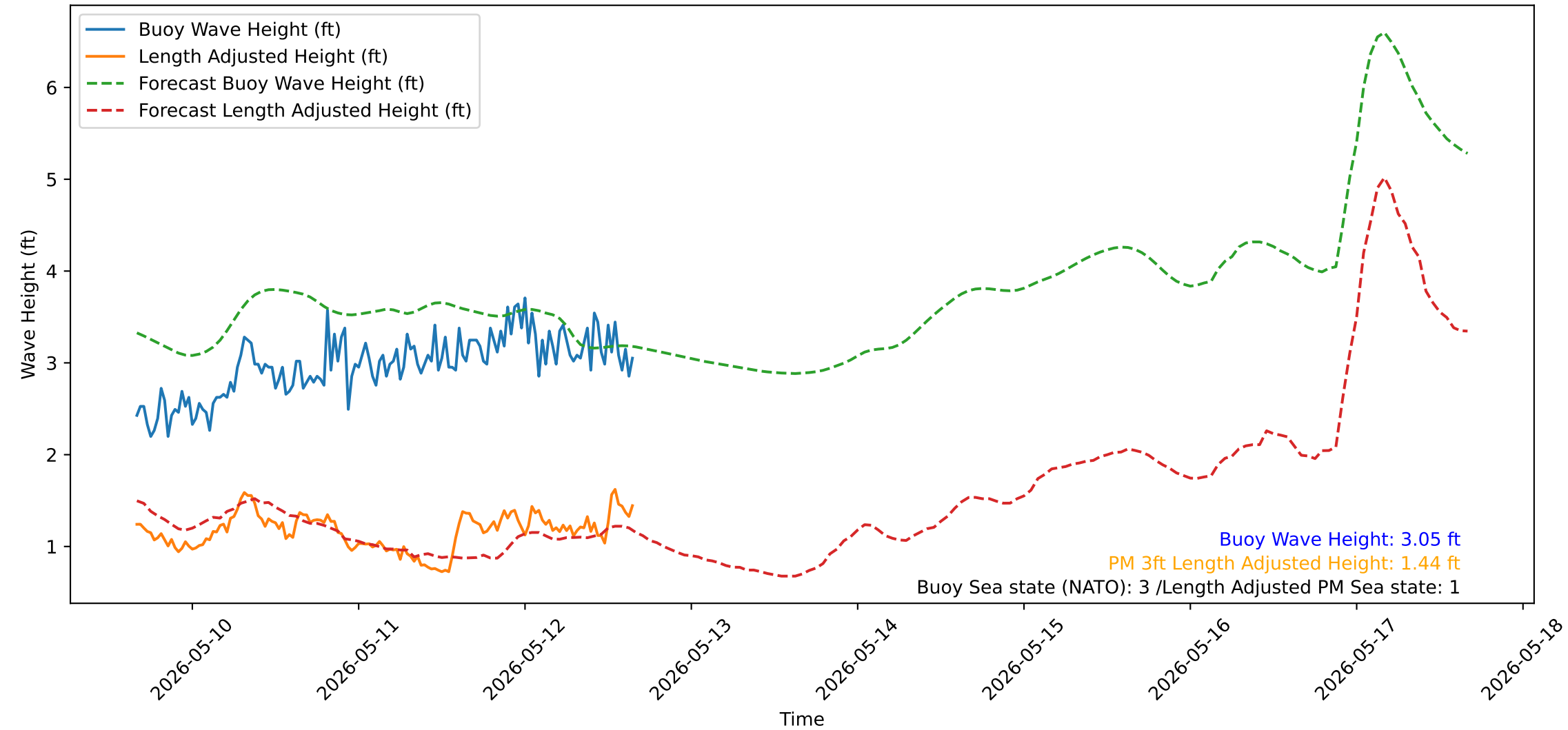
Wave Heights over Time for Oceanside Harbor at 2026-05-12 16:10:31
