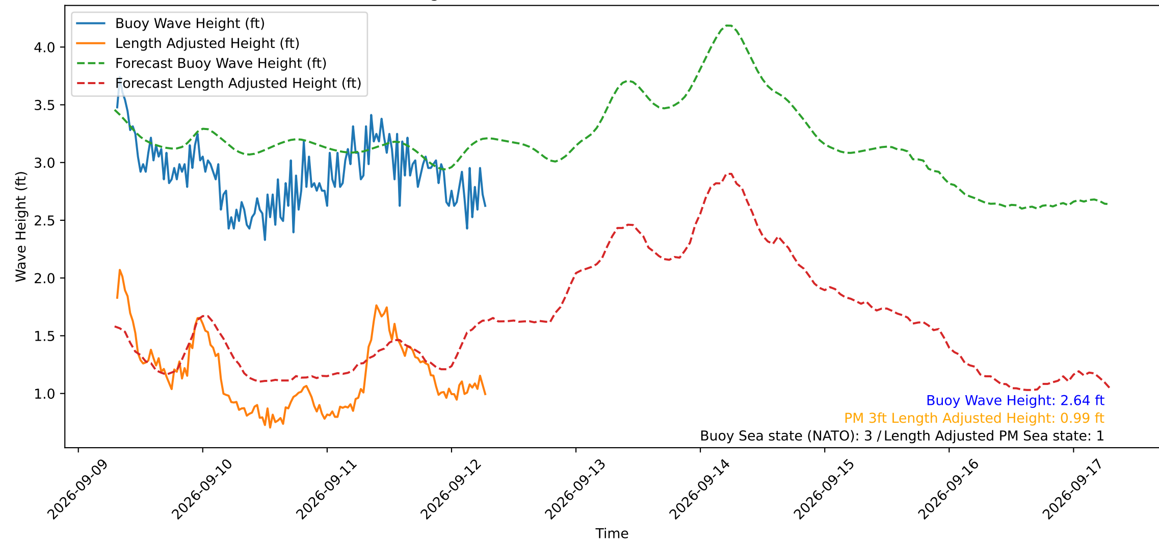
Wave Heights over Time for Red Beach at 2026-09-12 07:20:50
