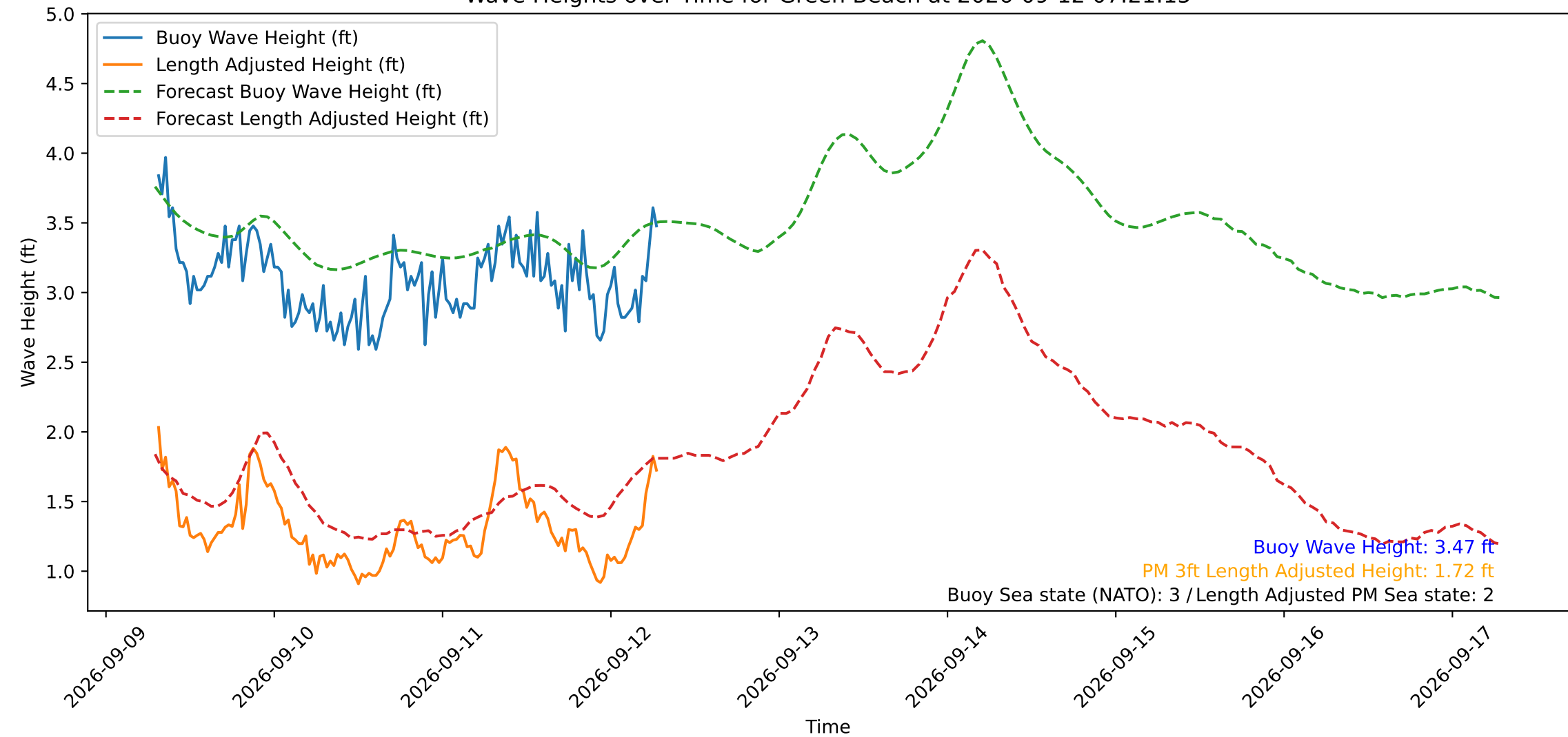
Wave Heights over Time for Green Beach at 2026-09-12 07:21:15
