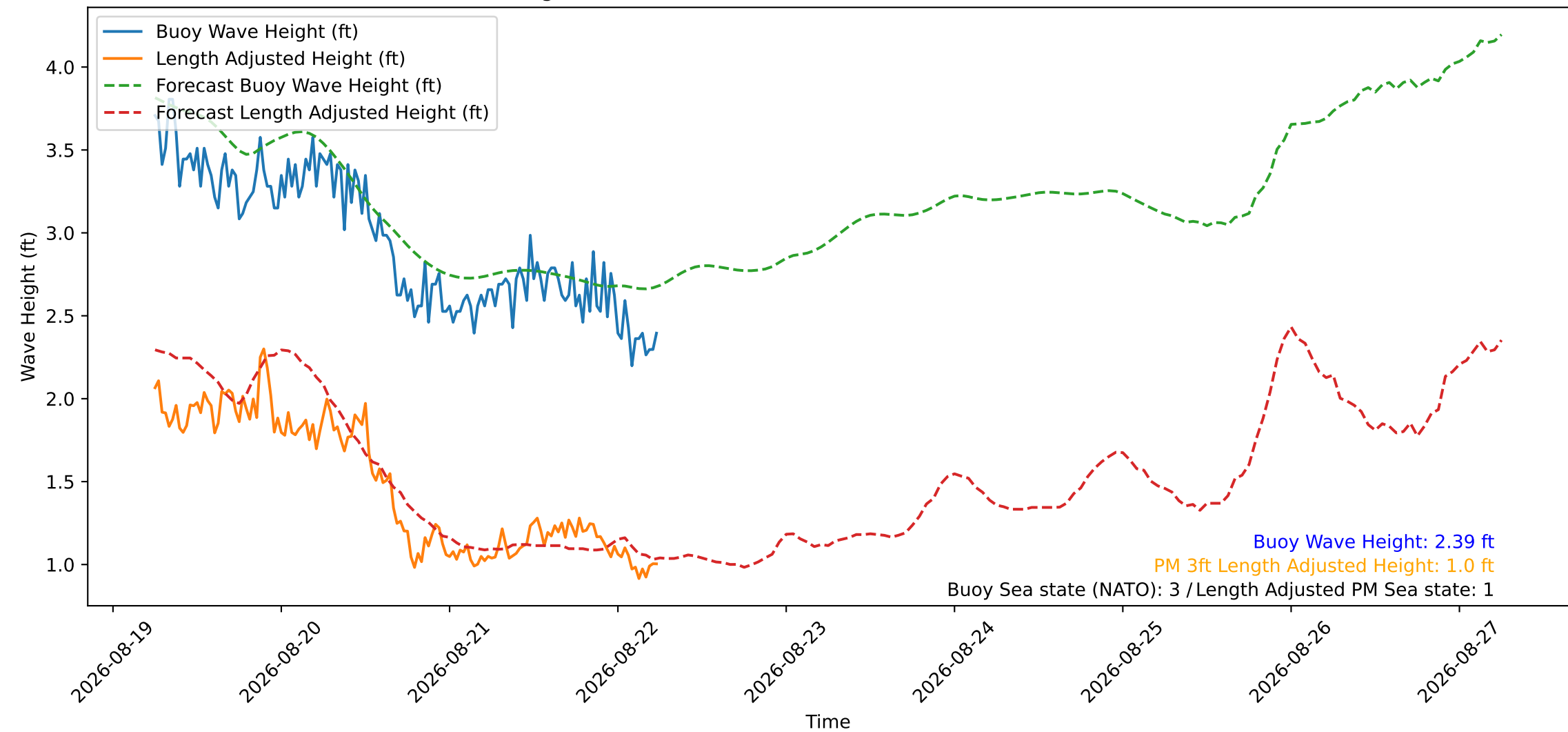
Wave Heights over Time for Oceanside Harbor at 2026-08-22 06:10:29
