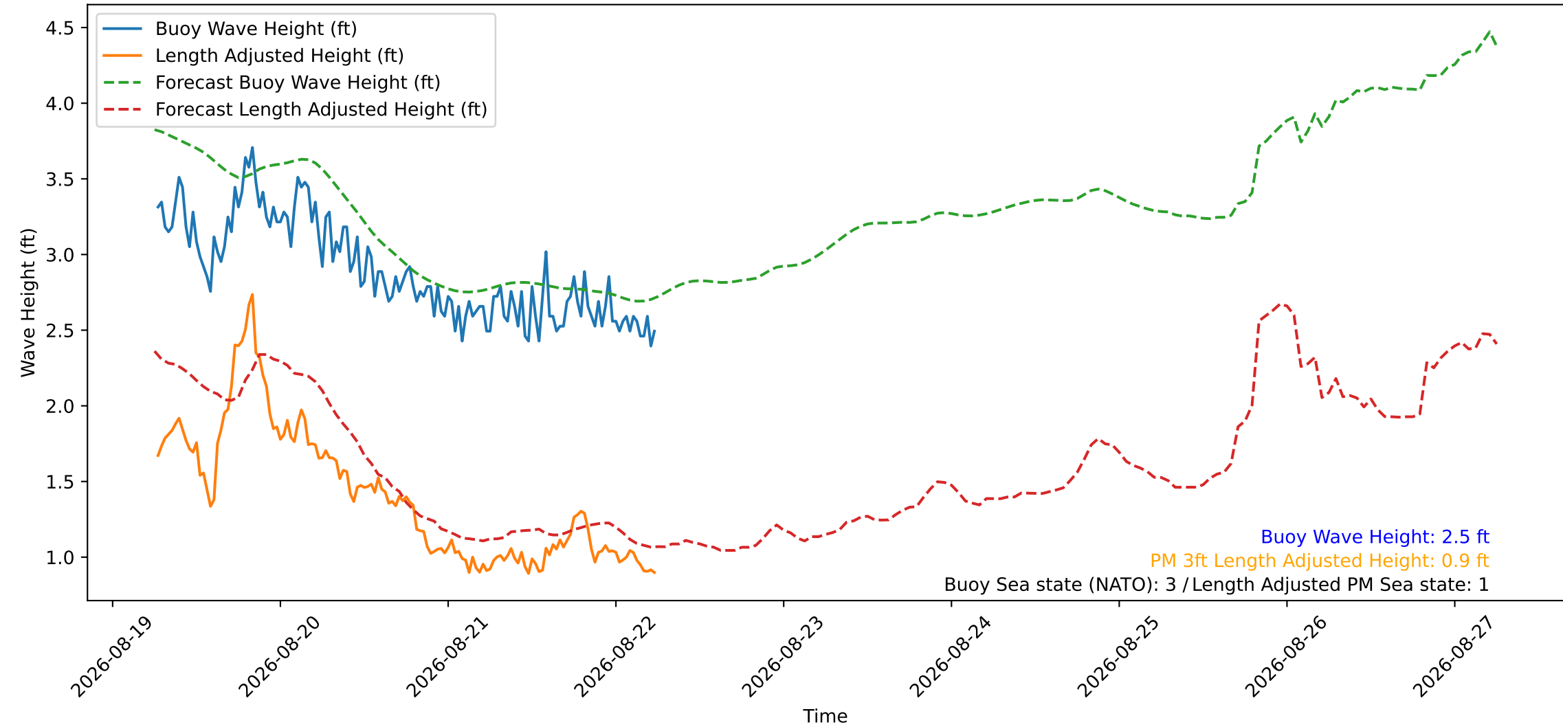
Wave Heights over Time for Green Beach at 2026-08-22 06:11:11
