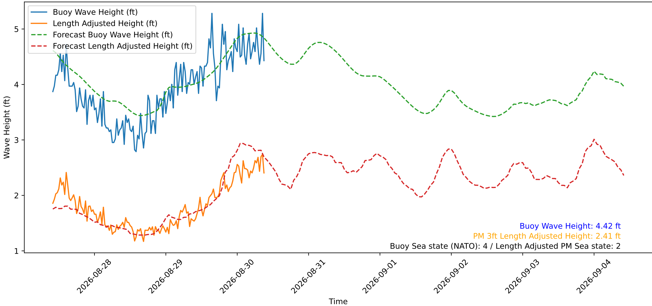
Wave Heights over Time for Oceanside Harbor at 2026-08-30 10:00:29
