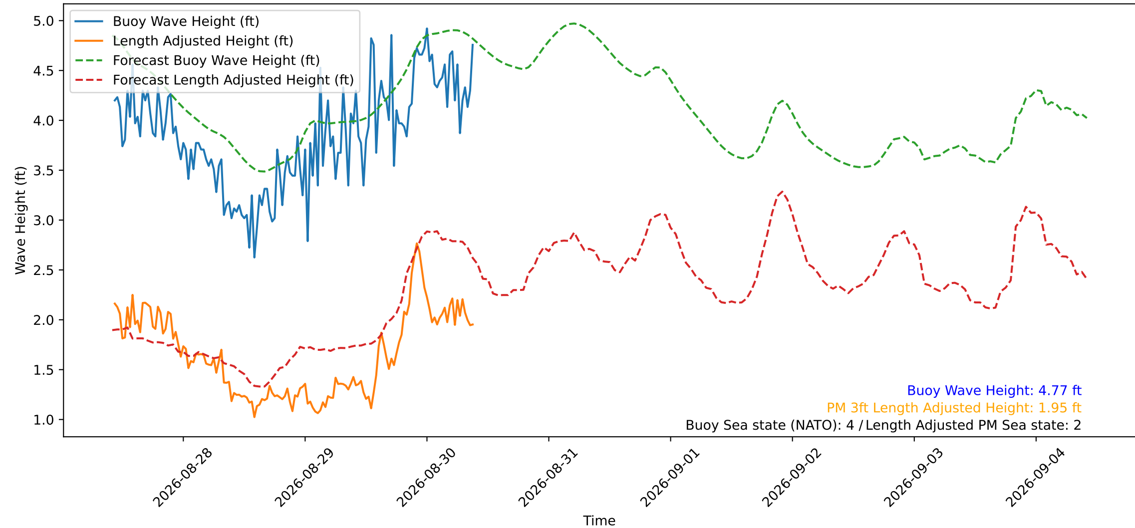
Wave Heights over Time for Green Beach at 2026-08-30 10:01:11
