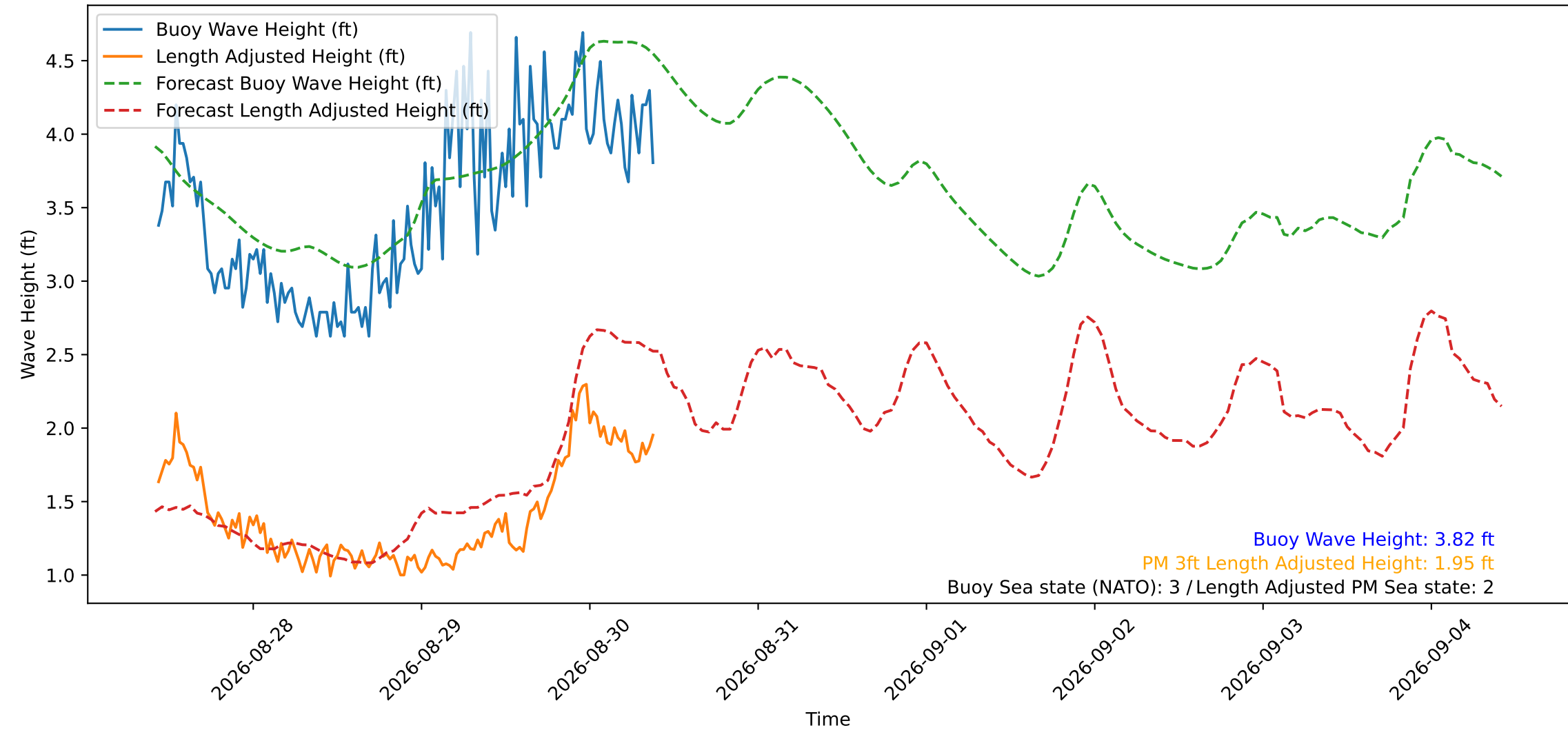
Wave Heights over Time for Red Beach at 2026-08-30 10:00:49
