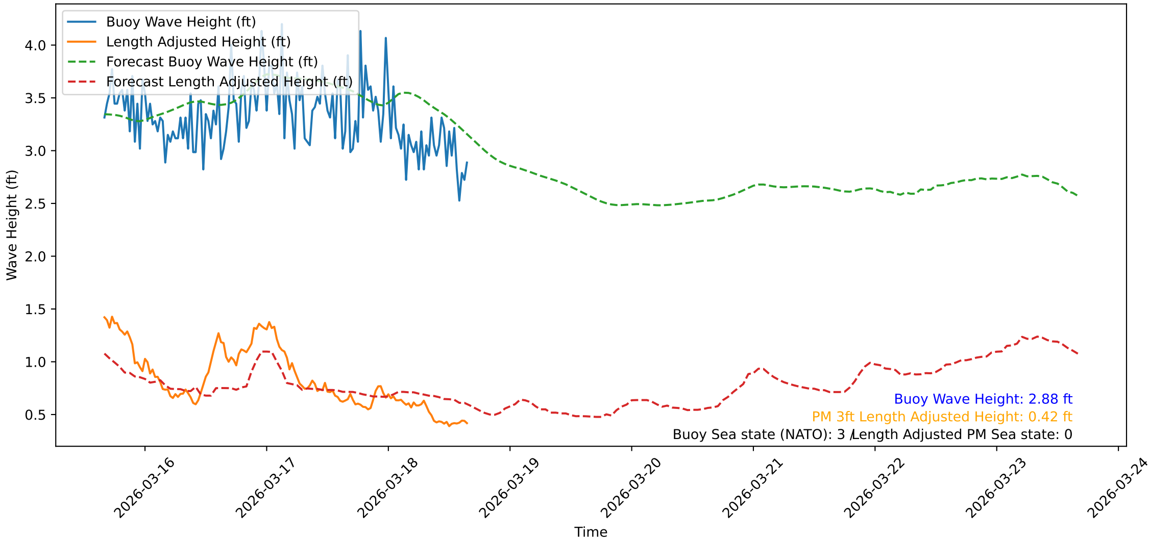
Wave Heights over Time for Green Beach at 2026-03-18 16:11:10
