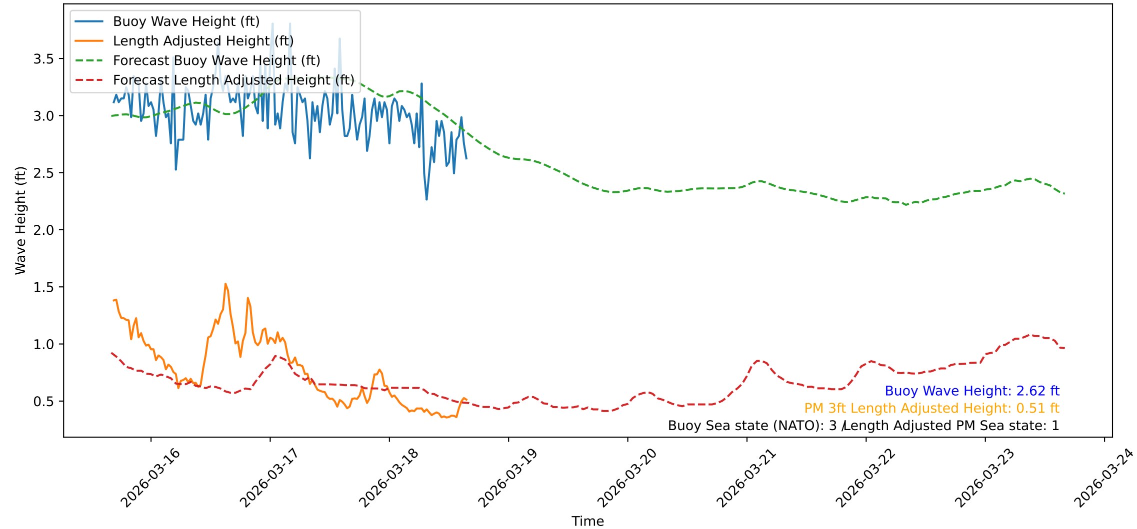
Wave Heights over Time for Red Beach at 2026-03-18 16:10:47
