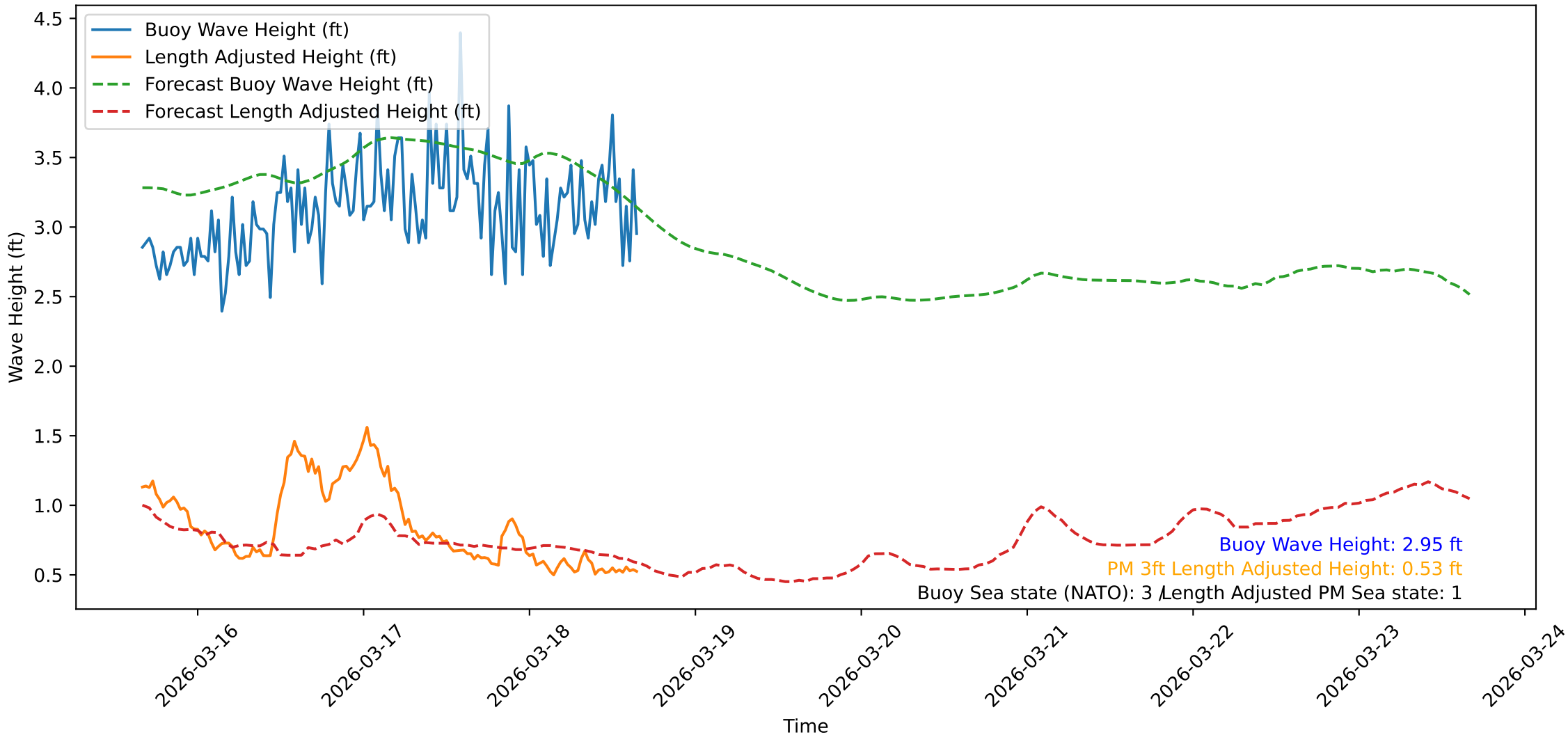
Wave Heights over Time for Oceanside Harbor at 2026-03-18 16:10:31
