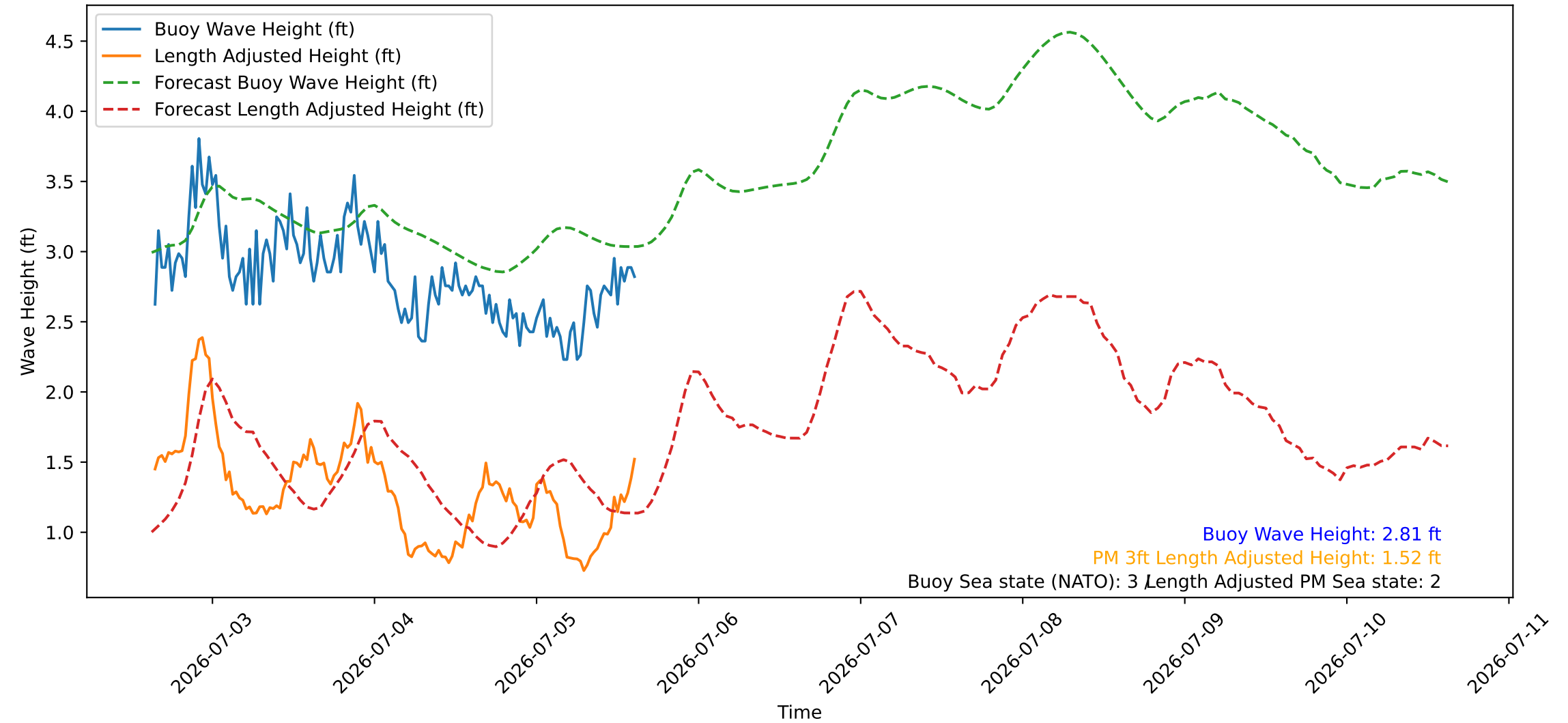
Wave Heights over Time for Red Beach at 2026-07-05 15:10:47
