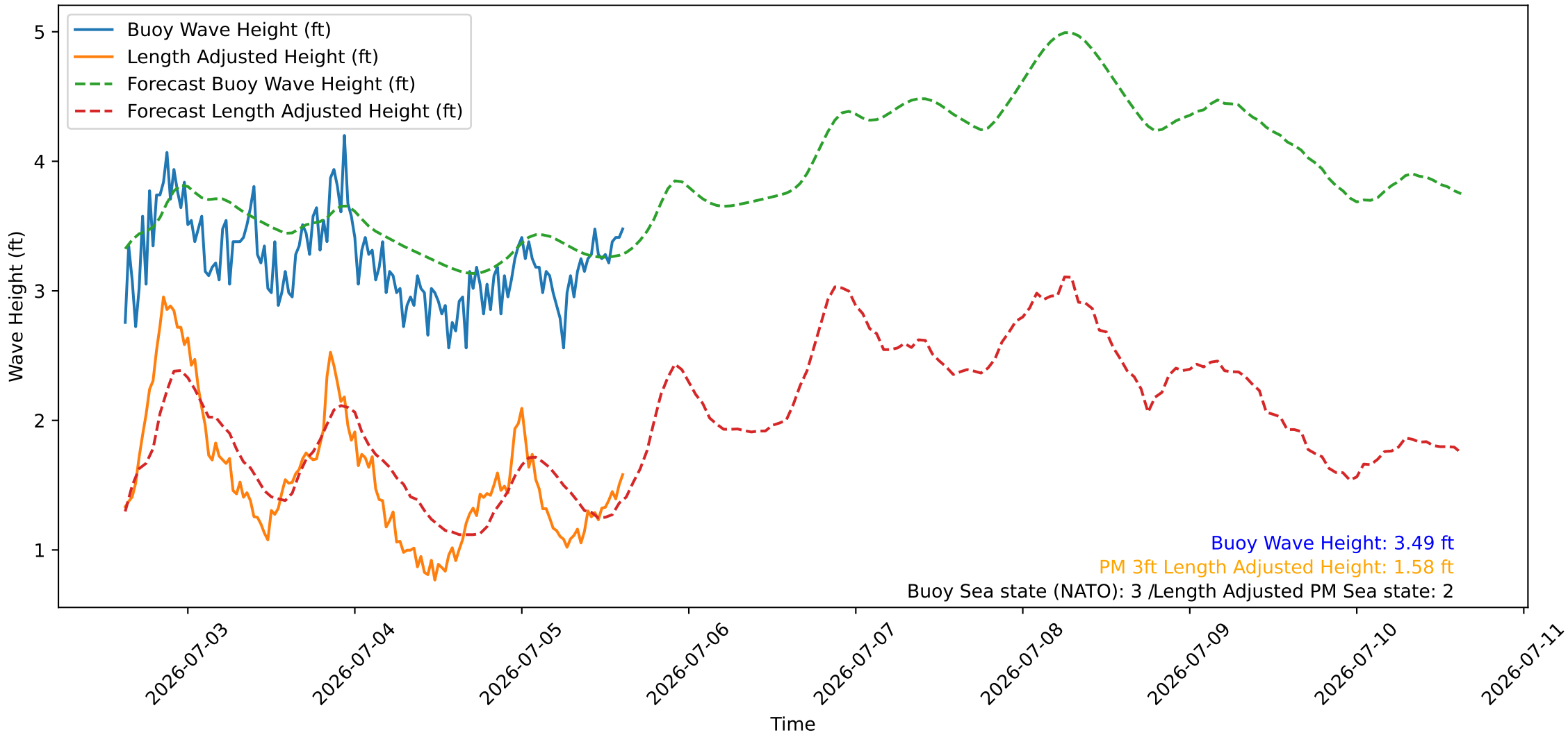
Wave Heights over Time for Green Beach at 2026-07-05 15:11:09
