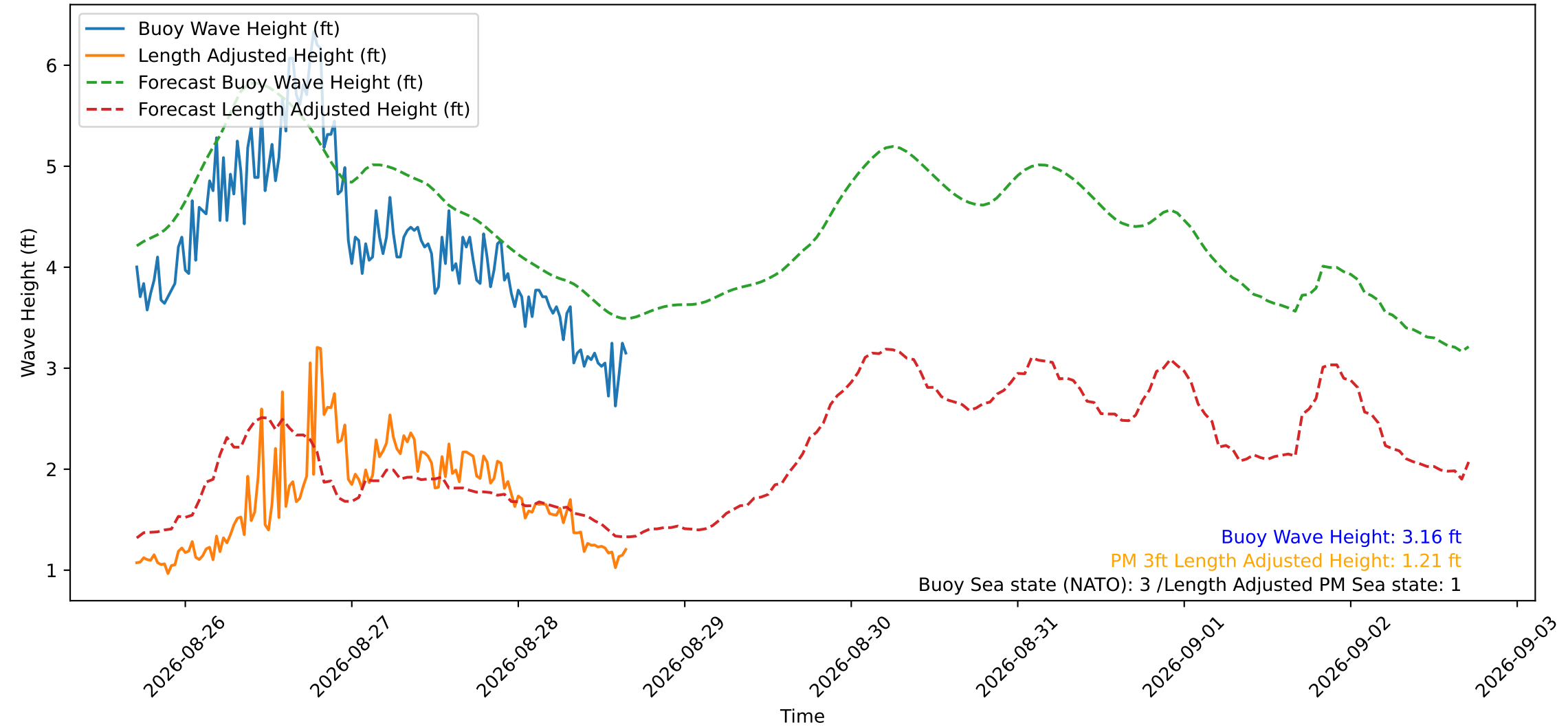
Wave Heights over Time for Green Beach at 2026-08-28 16:31:12
