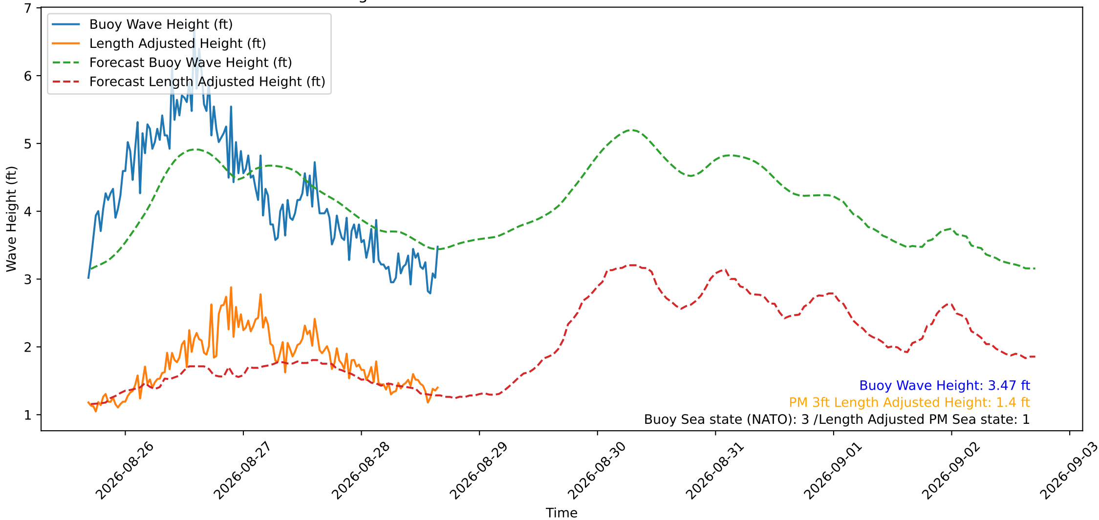
Wave Heights over Time for Oceanside Harbor at 2026-08-28 16:30:30
