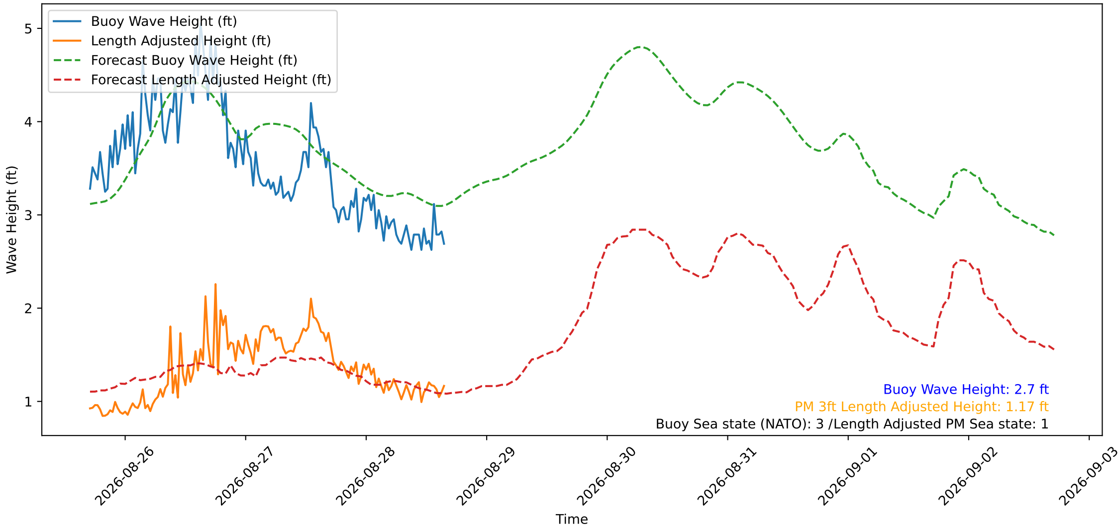
Wave Heights over Time for Red Beach at 2026-08-28 16:30:49
