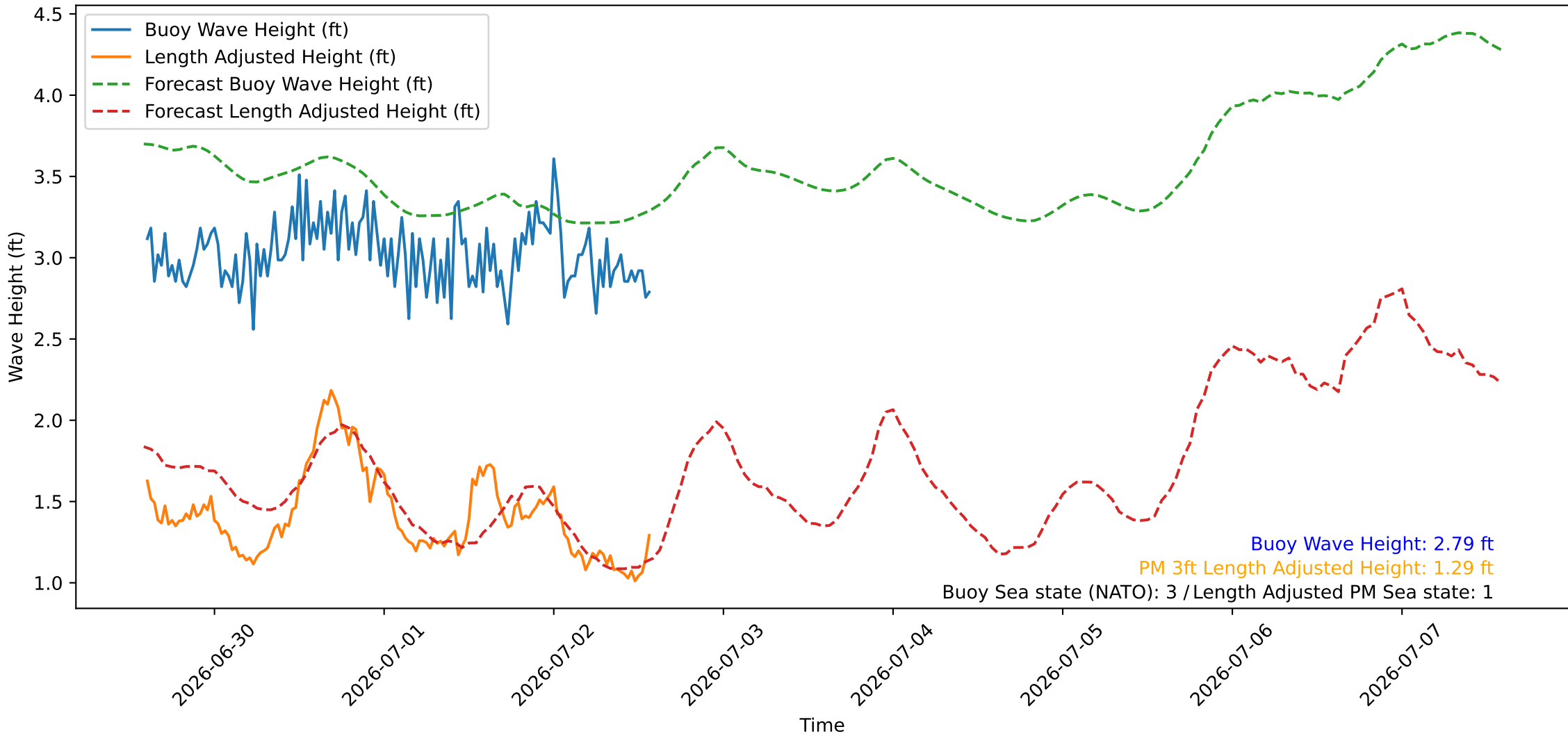
Wave Heights over Time for Oceanside Harbor at 2026-07-02 14:20:26
