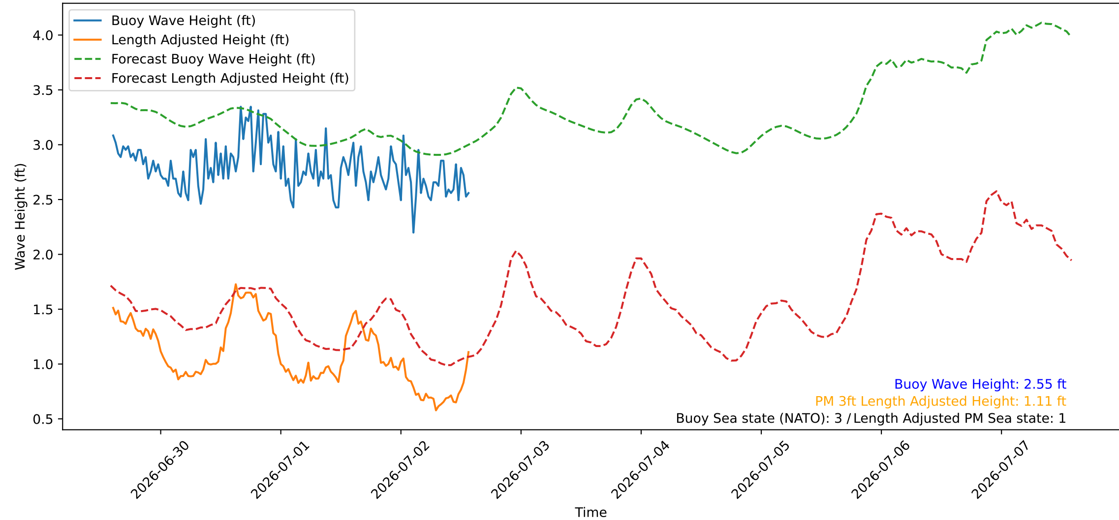
Wave Heights over Time for Red Beach at 2026-07-02 14:20:47
