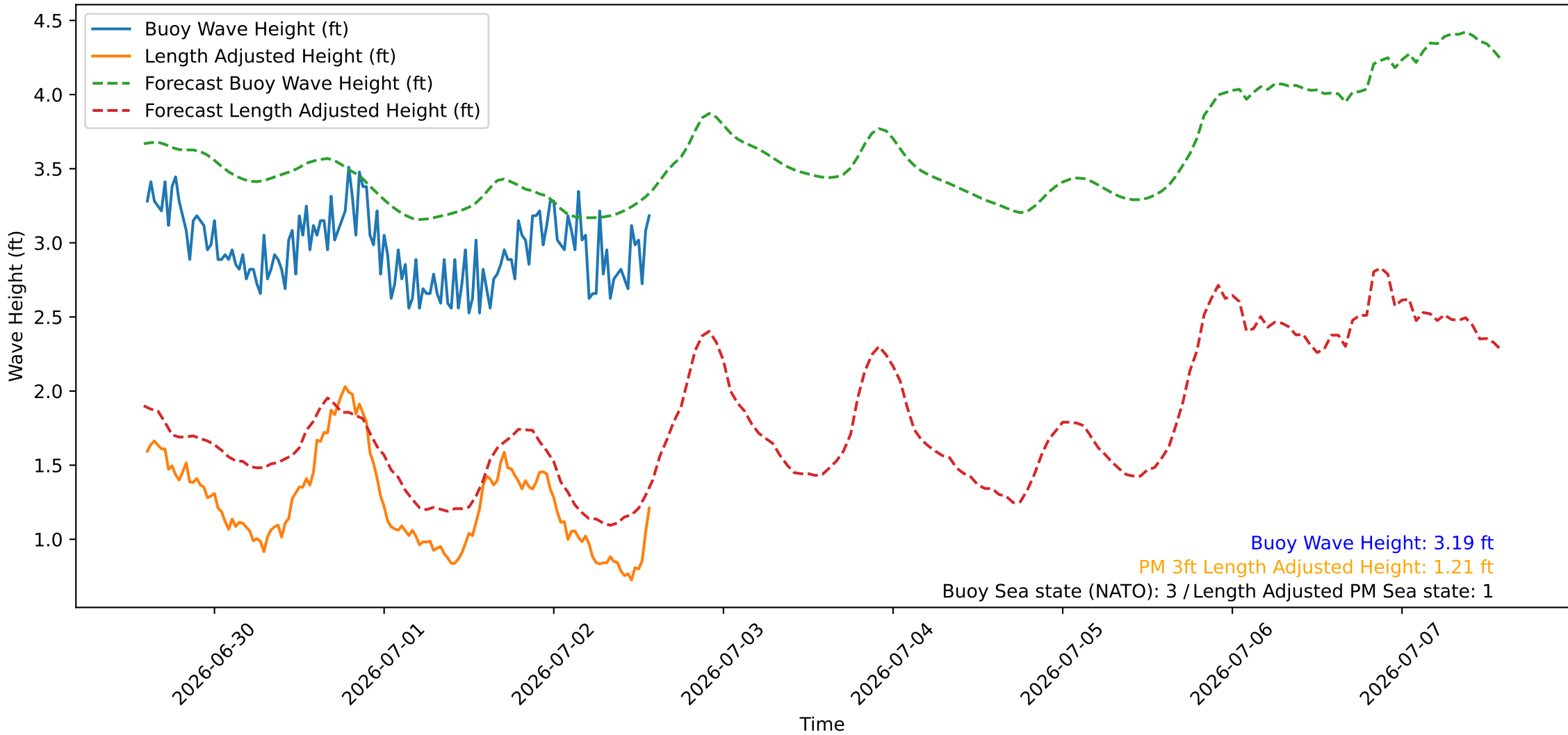
Wave Heights over Time for Green Beach at 2026-07-02 14:21:09
