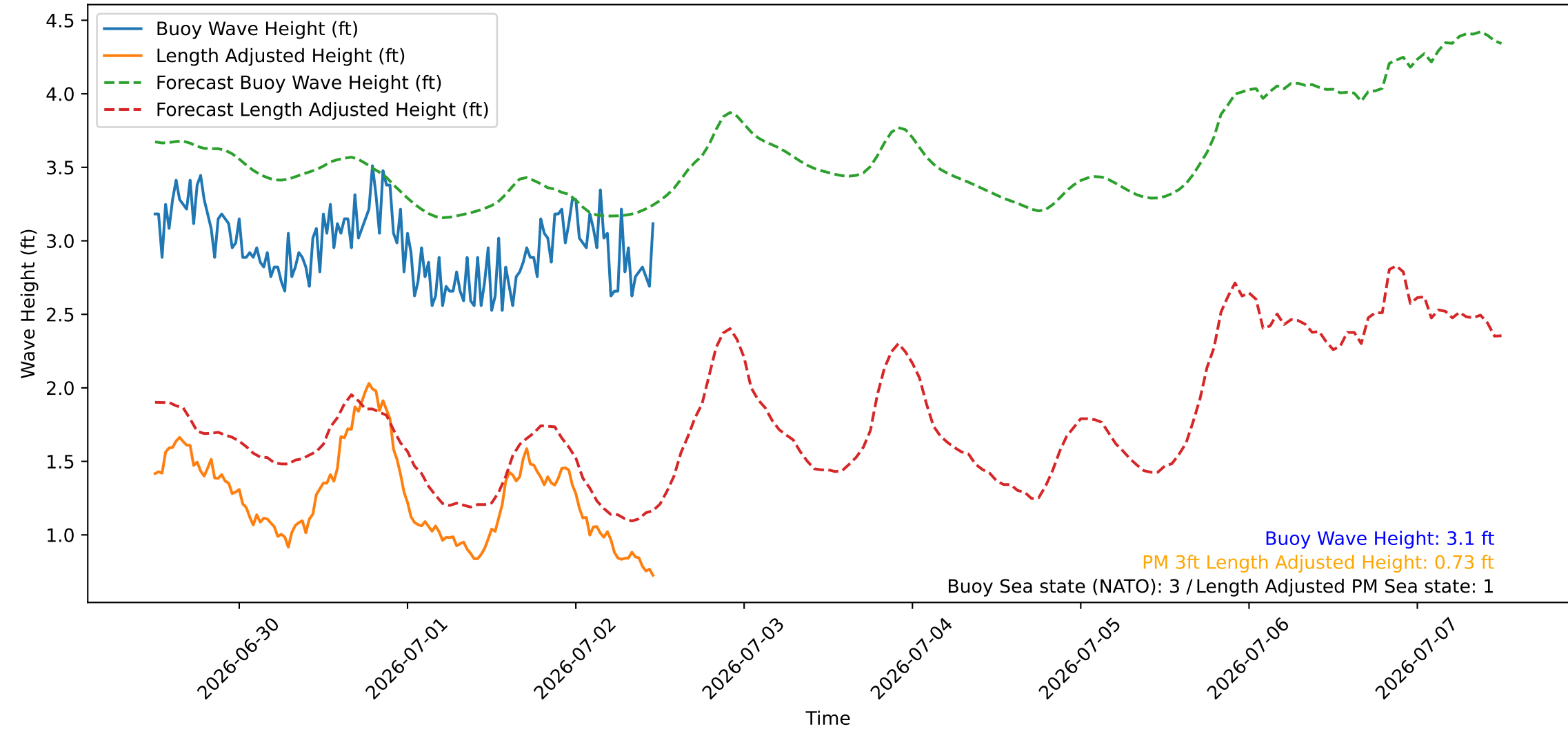
Wave Heights over Time for Green Beach at 2026-07-02 11:51:09
