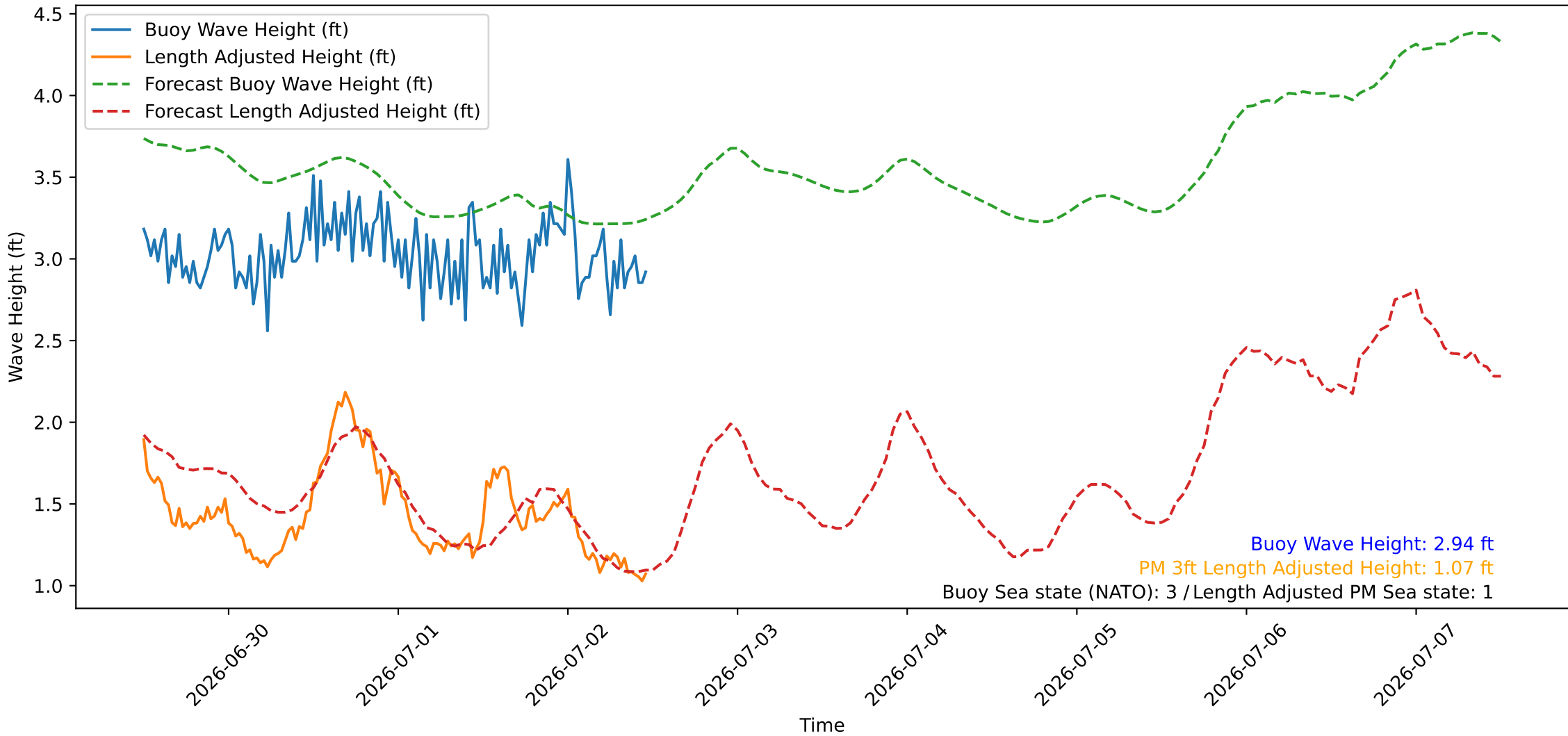
Wave Heights over Time for Oceanside Harbor at 2026-07-02 11:50:26
