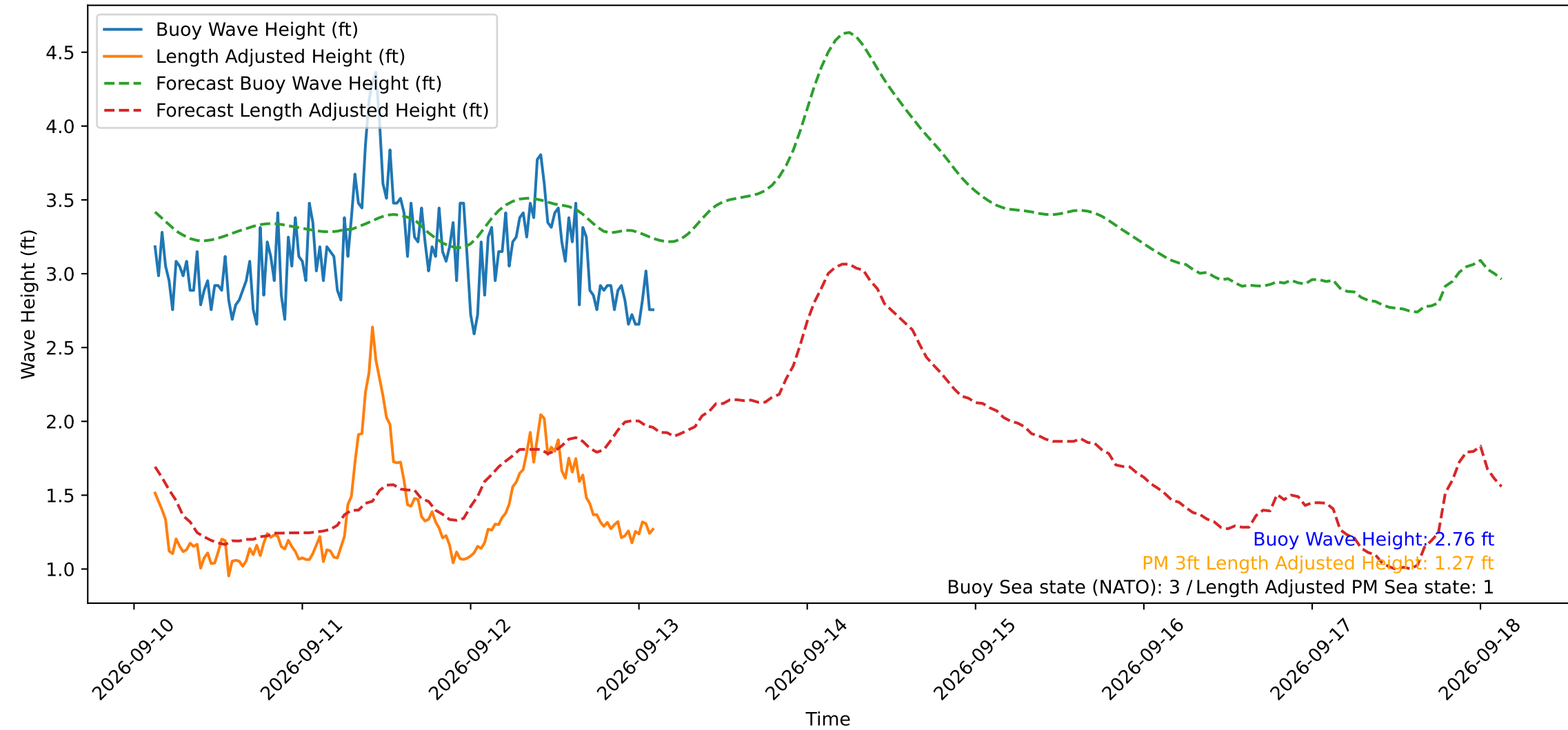
Wave Heights over Time for Oceanside Harbor at 2026-09-13 03:00:29
