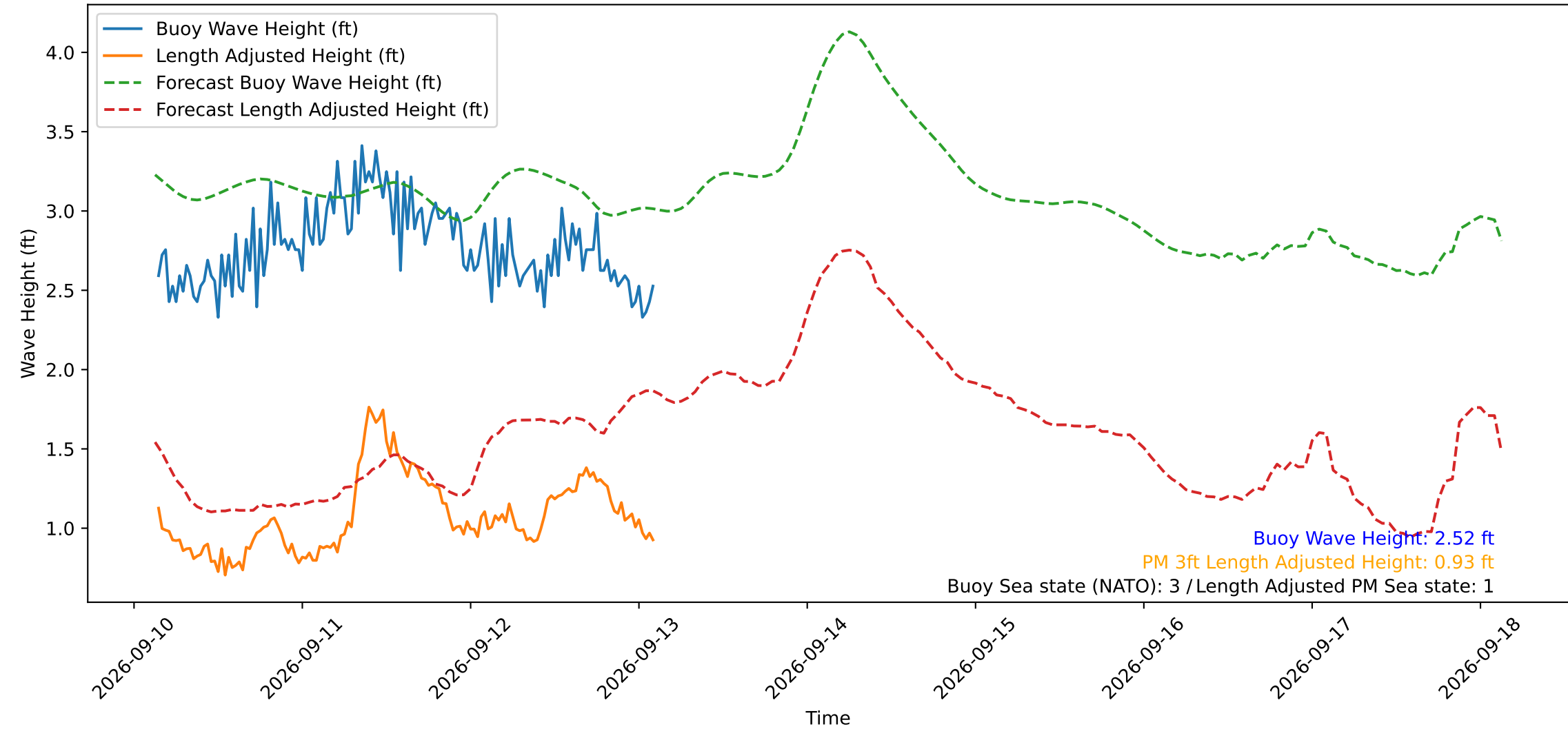
Wave Heights over Time for Red Beach at 2026-09-13 03:00:50
