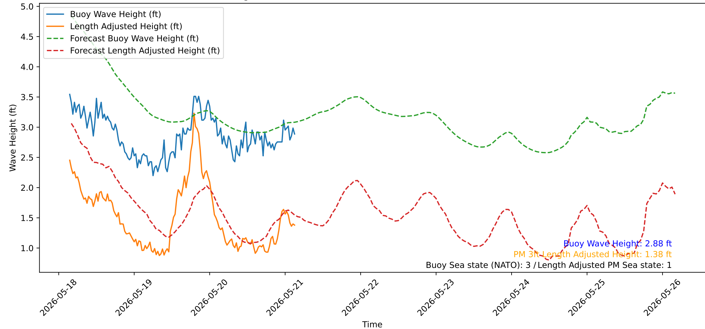
Wave Heights over Time for Oceanside Harbor at 2026-05-21 03:40:32
