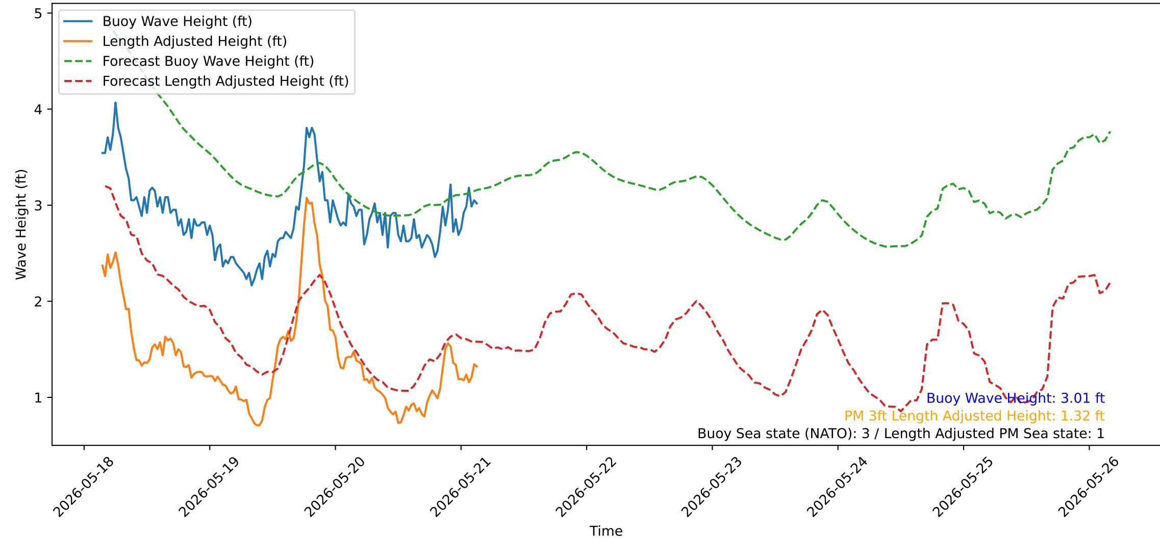
Wave Heights over Time for Green Beach at 2026-05-21 03:41:14
