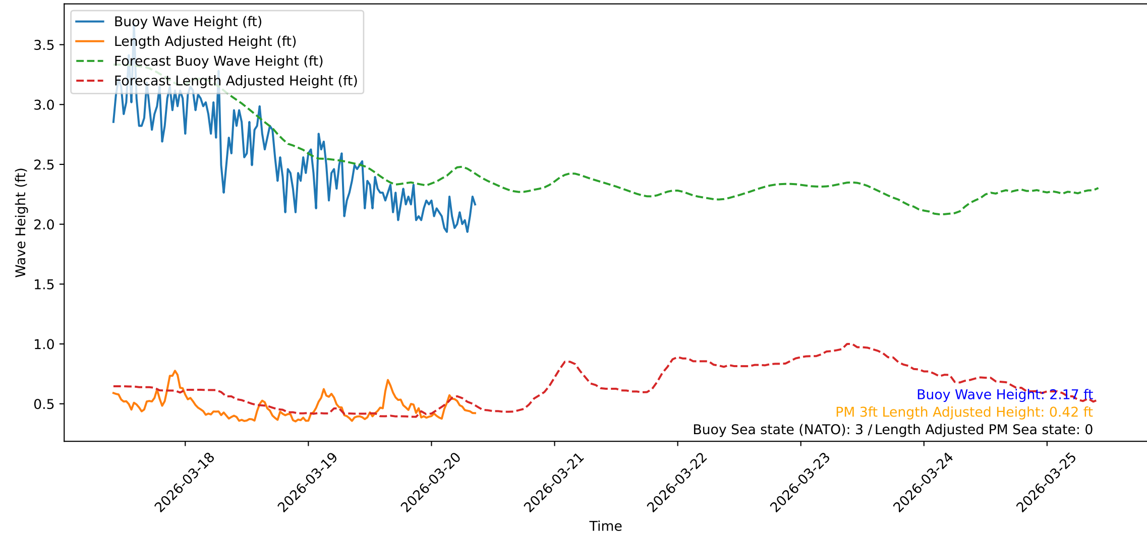
Wave Heights over Time for Red Beach at 2026-03-20 09:30:48
