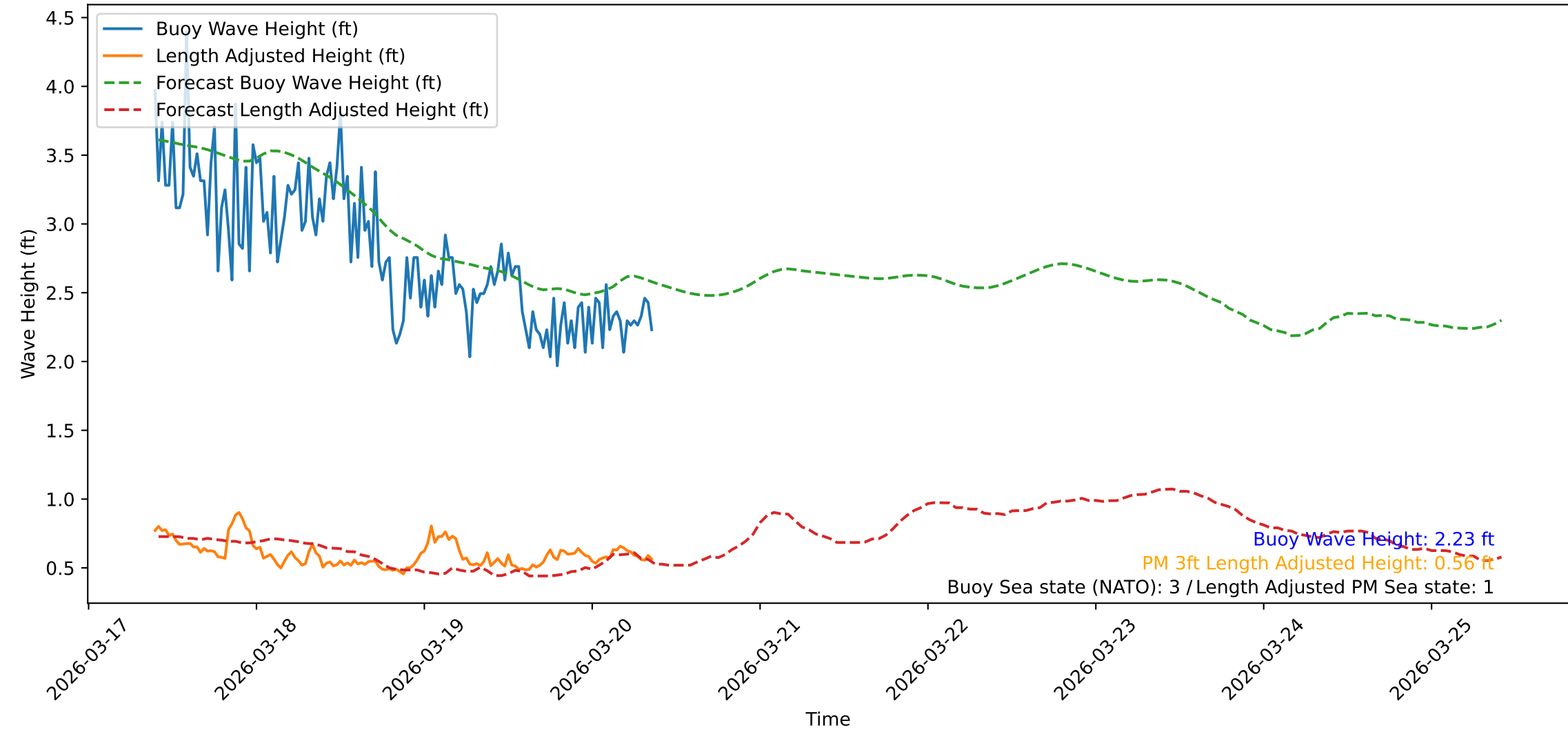
Wave Heights over Time for Oceanside Harbor at 2026-03-20 09:30:32
