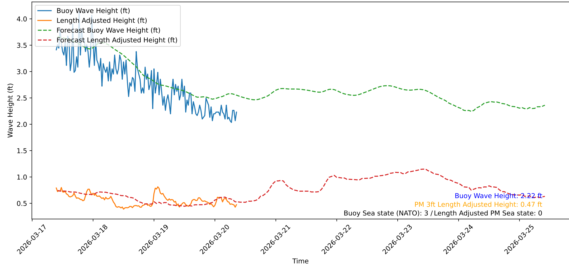
Wave Heights over Time for Green Beach at 2026-03-20 09:31:11
