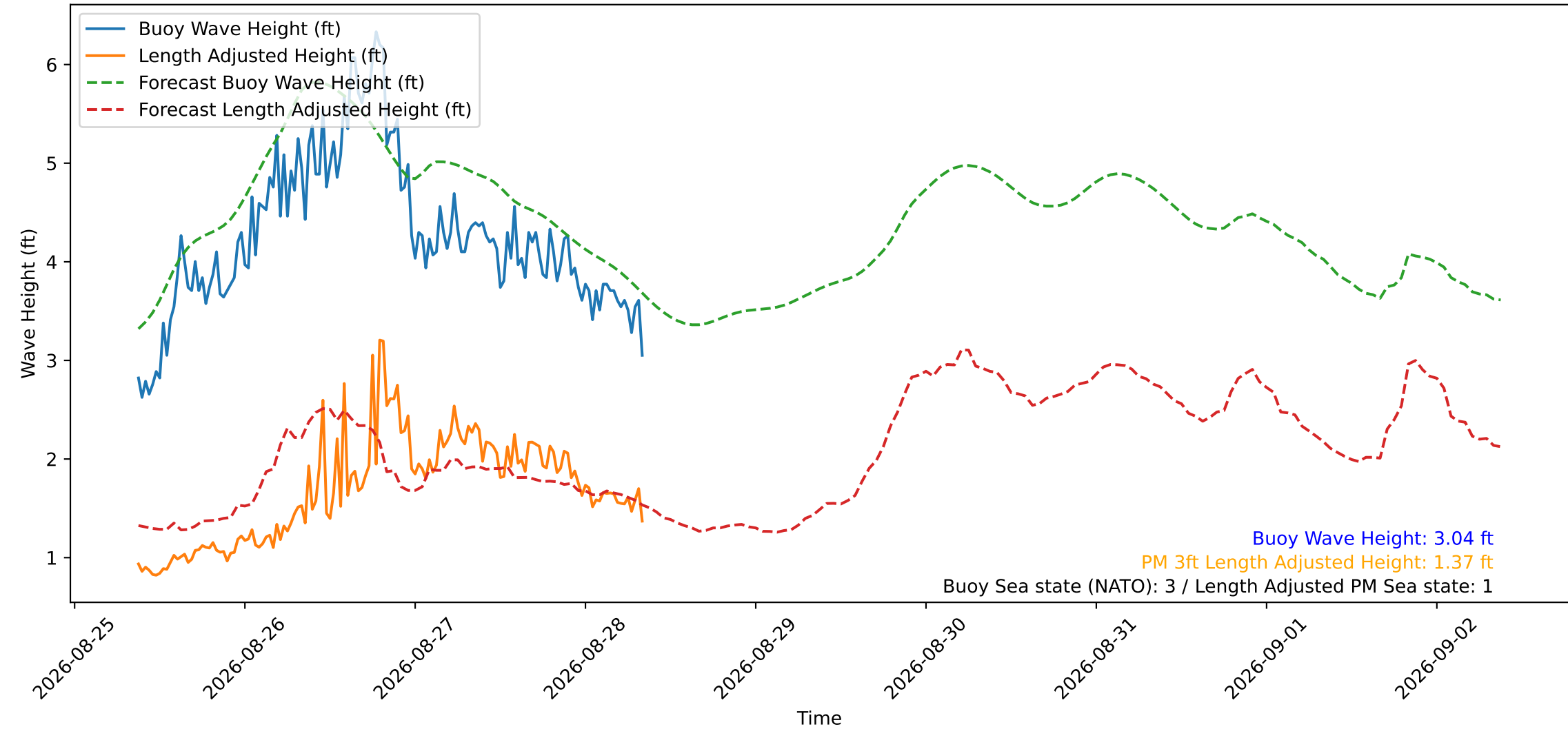
Wave Heights over Time for Green Beach at 2026-08-28 08:41:12
