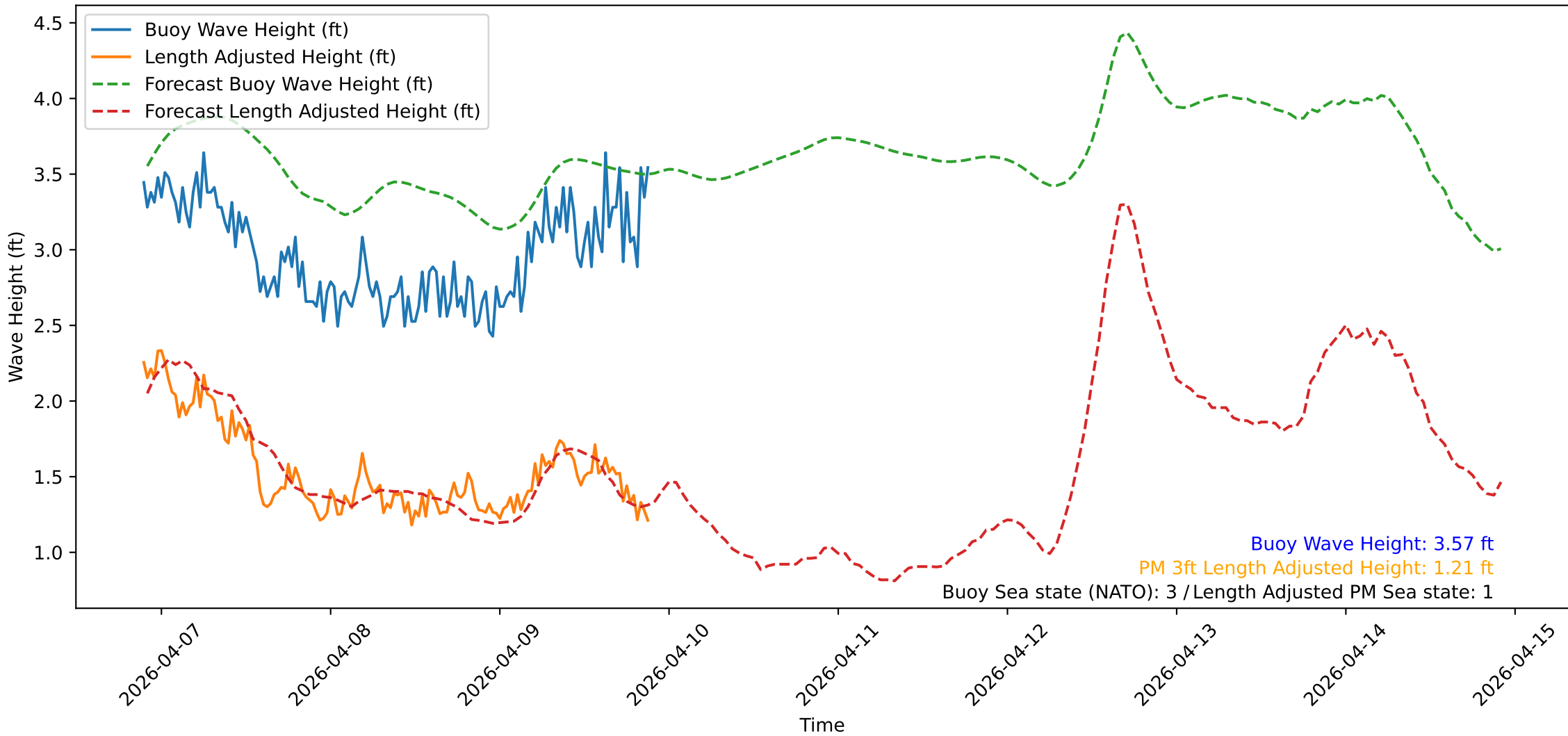
Wave Heights over Time for Oceanside Harbor at 2026-04-09 21:40:31
