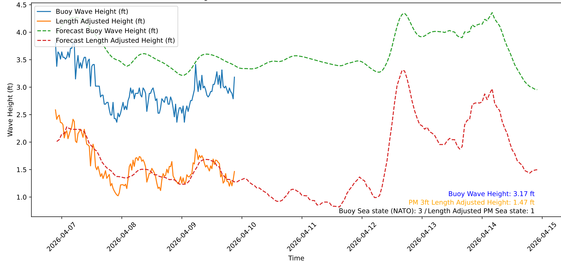
Wave Heights over Time for Green Beach at 2026-04-09 21:41:09
