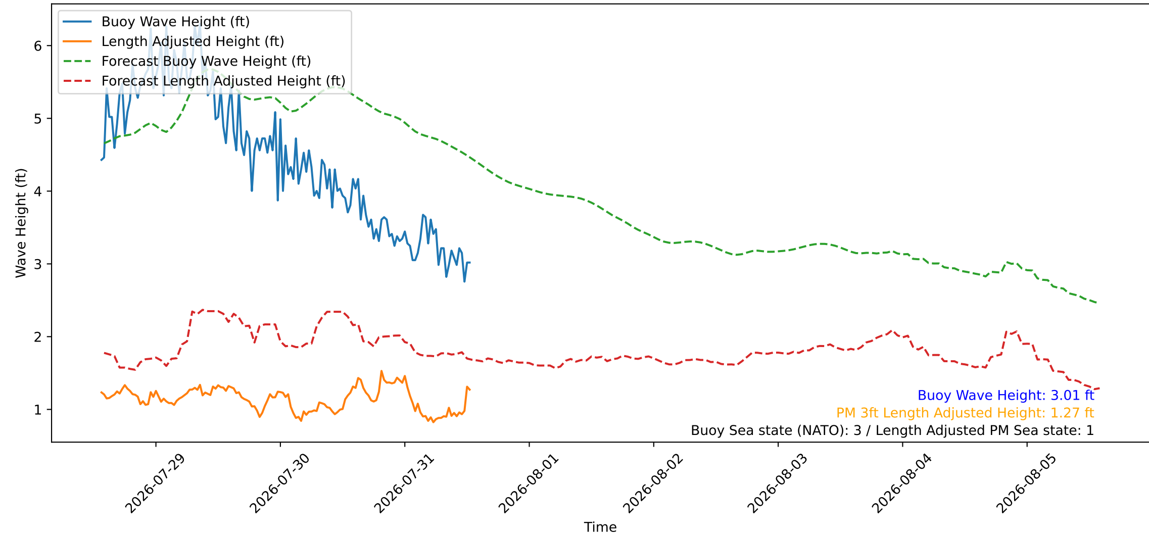
Wave Heights over Time for Green Beach at 2026-07-31 13:41:09
