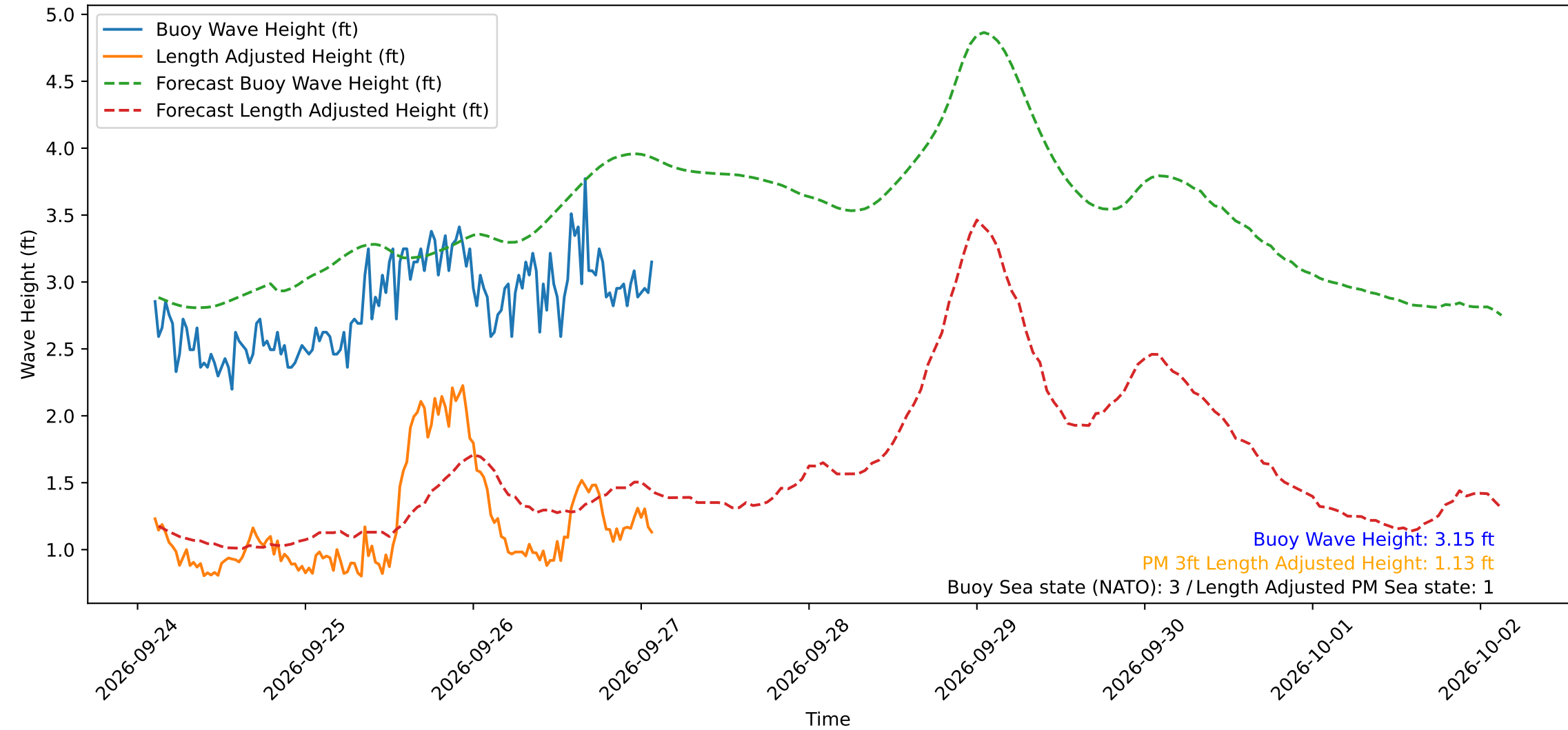
Wave Heights over Time for Oceanside Harbor at 2026-09-27 02:30:30
