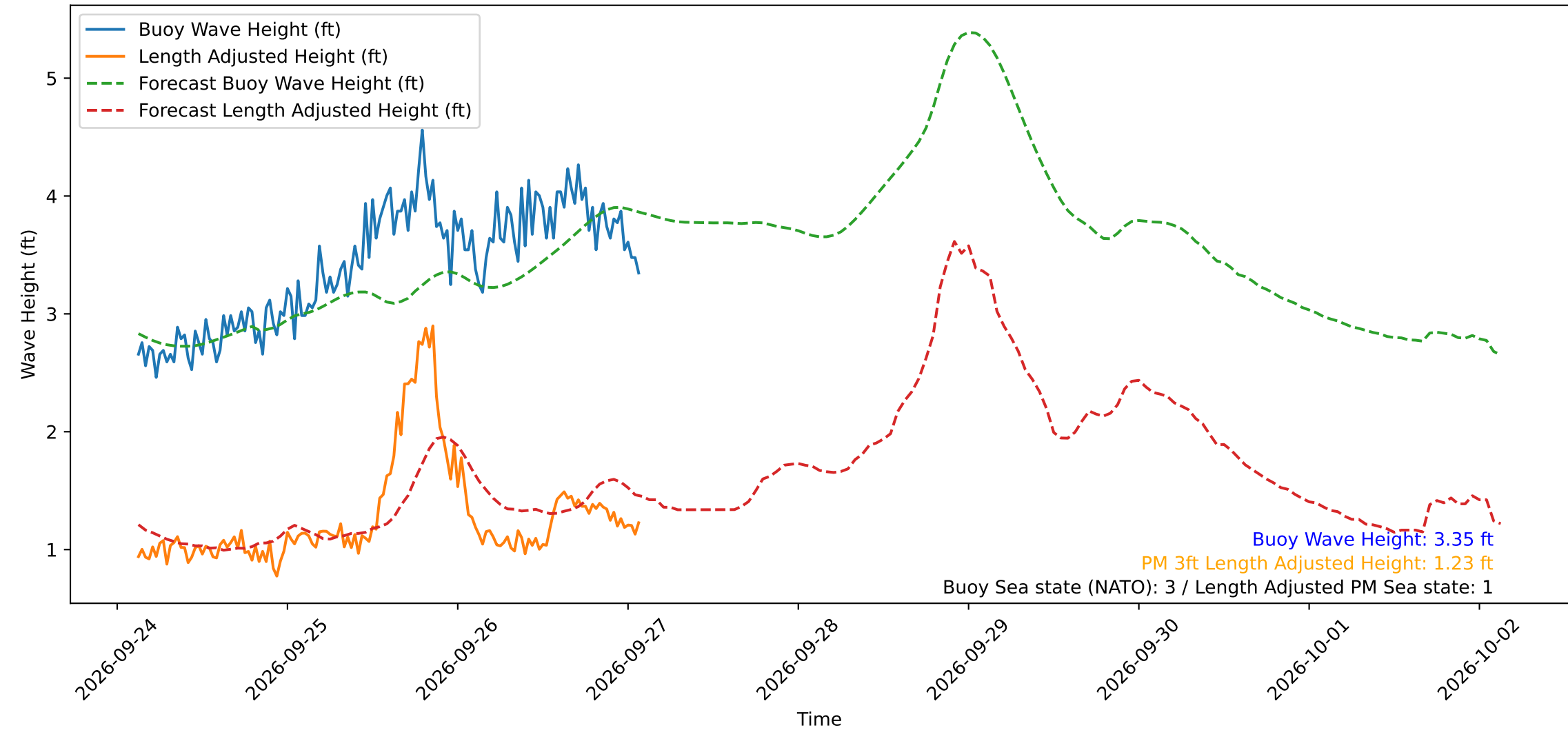
Wave Heights over Time for Green Beach at 2026-09-27 02:31:12
