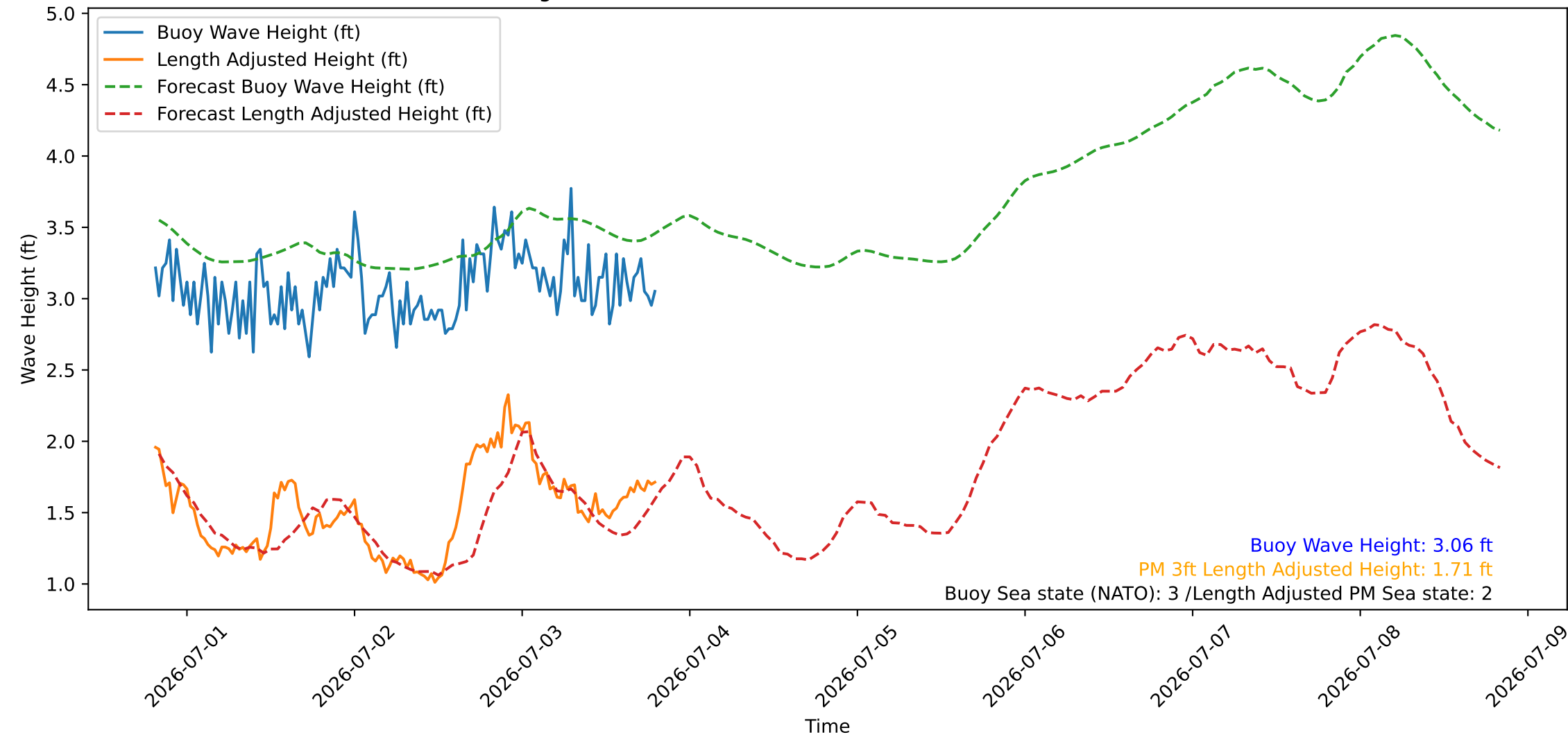
Wave Heights over Time for Oceanside Harbor at 2026-07-03 19:40:26
