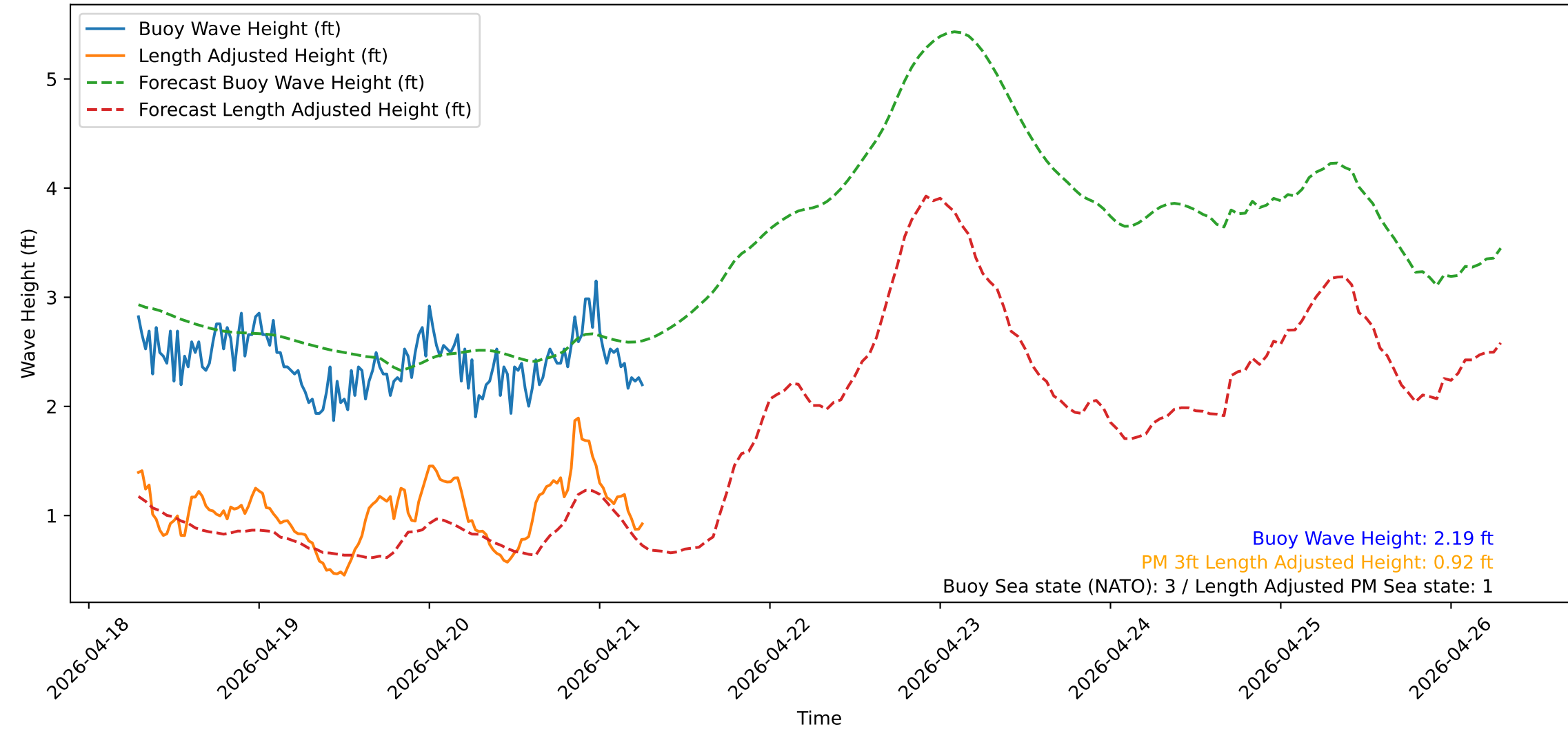
Wave Heights over Time for Green Beach at 2026-04-21 06:51:14
