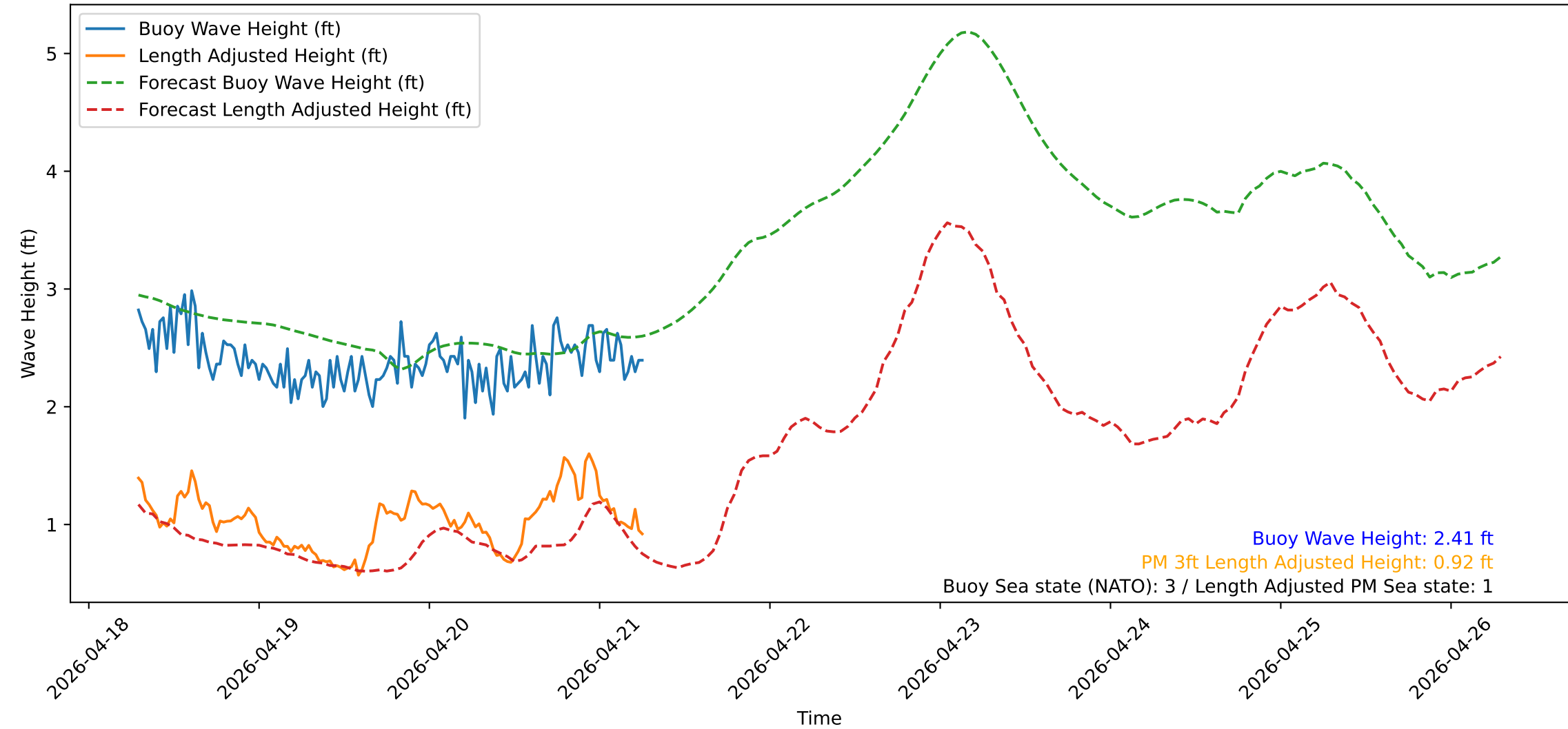
Wave Heights over Time for Oceanside Harbor at 2026-04-21 06:50:31
