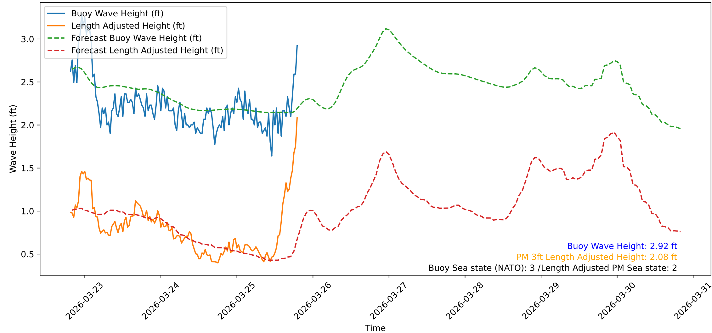
Wave Heights over Time for Green Beach at 2026-03-25 19:41:10
