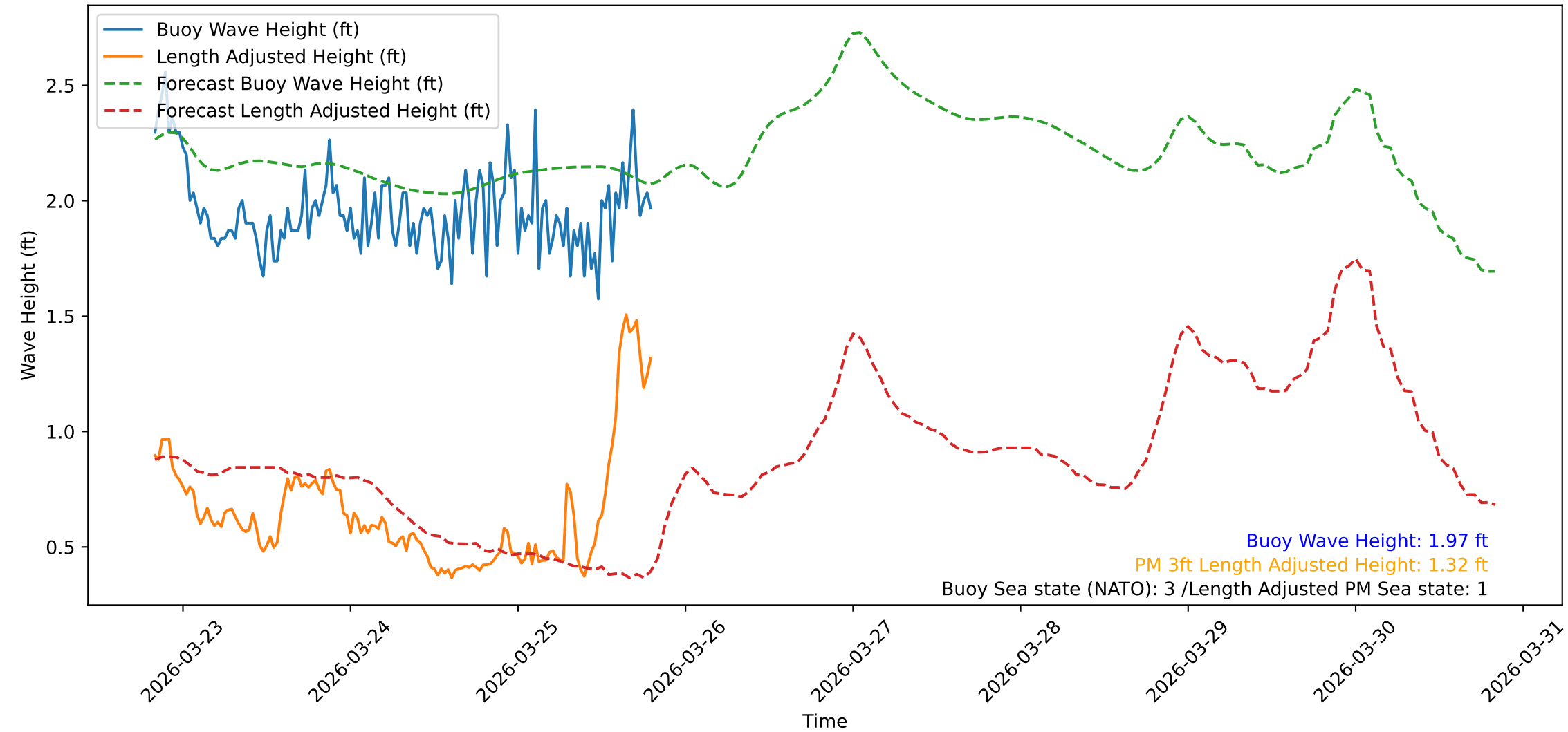
Wave Heights over Time for Red Beach at 2026-03-25 19:40:48
