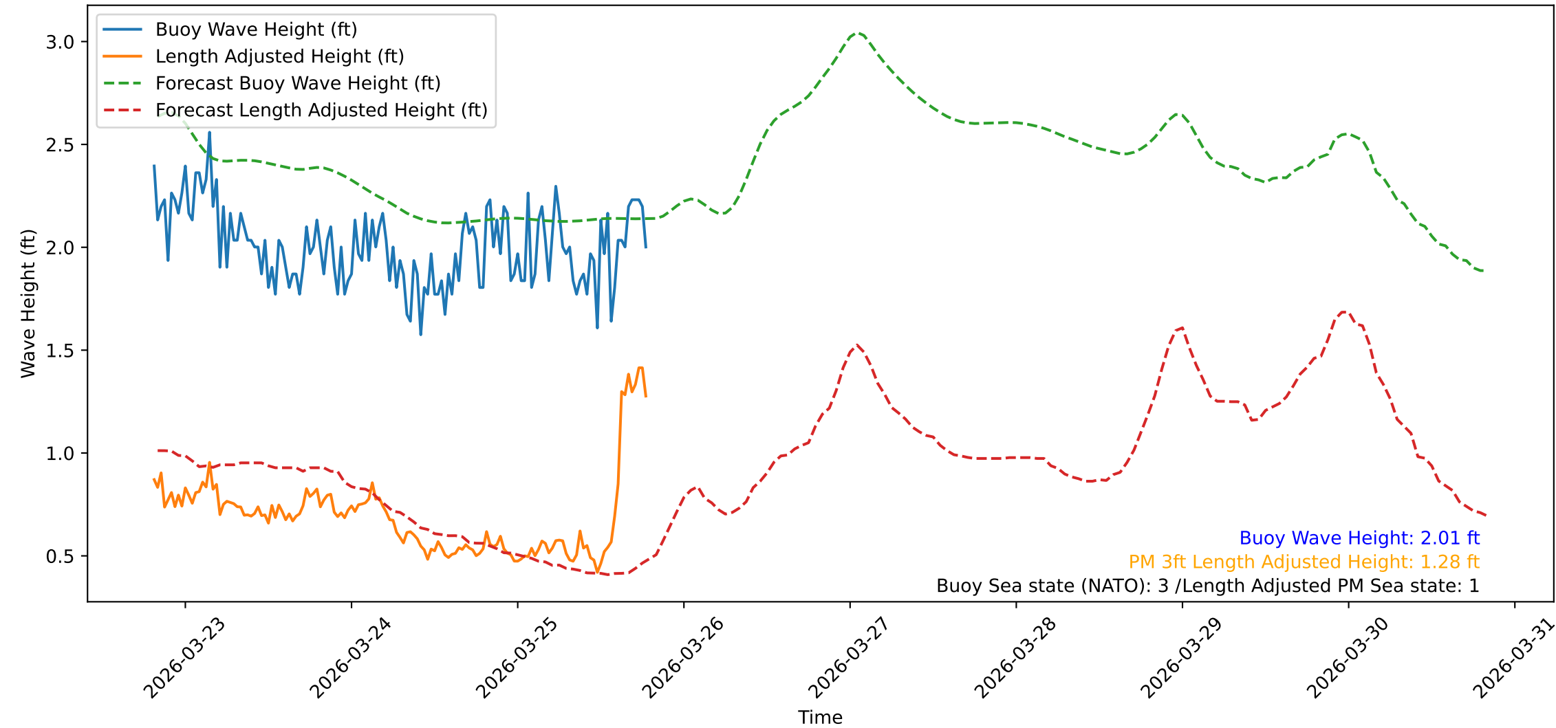
Wave Heights over Time for Oceanside Harbor at 2026-03-25 19:40:32
