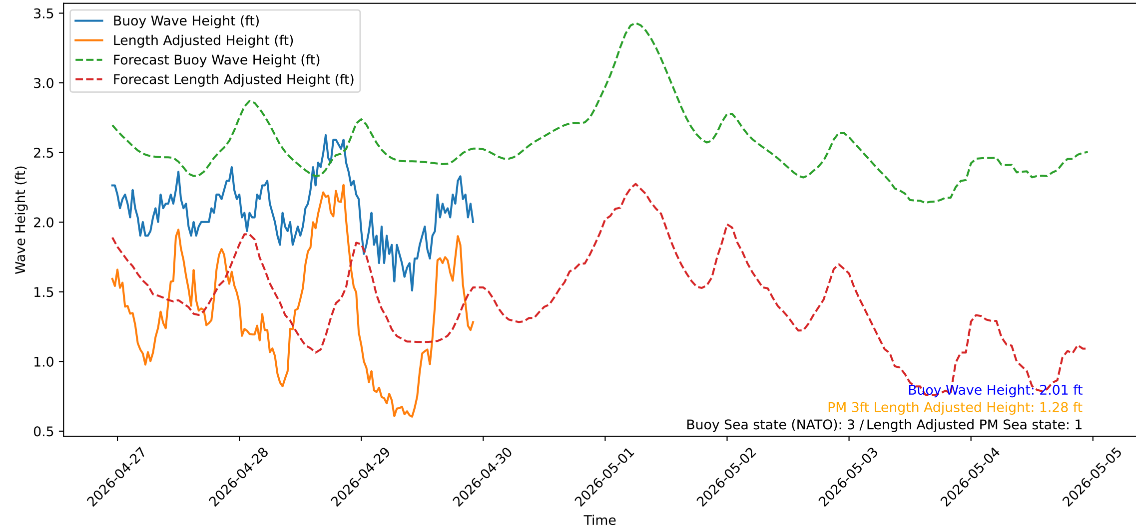
Wave Heights over Time for Red Beach at 2026-04-29 22:50:52
