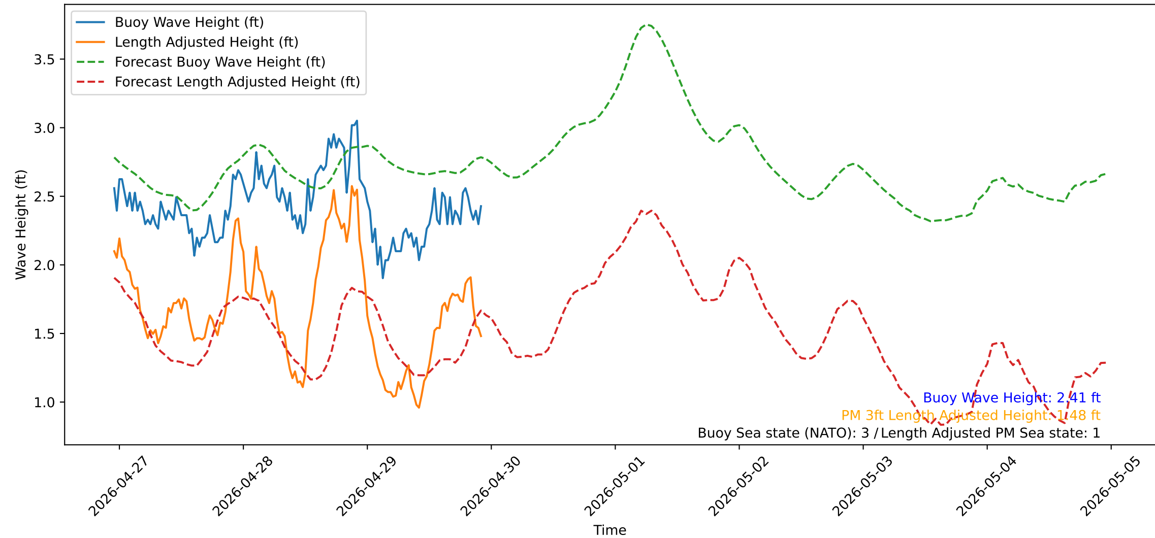
Wave Heights over Time for Oceanside Harbor at 2026-04-29 22:50:31
