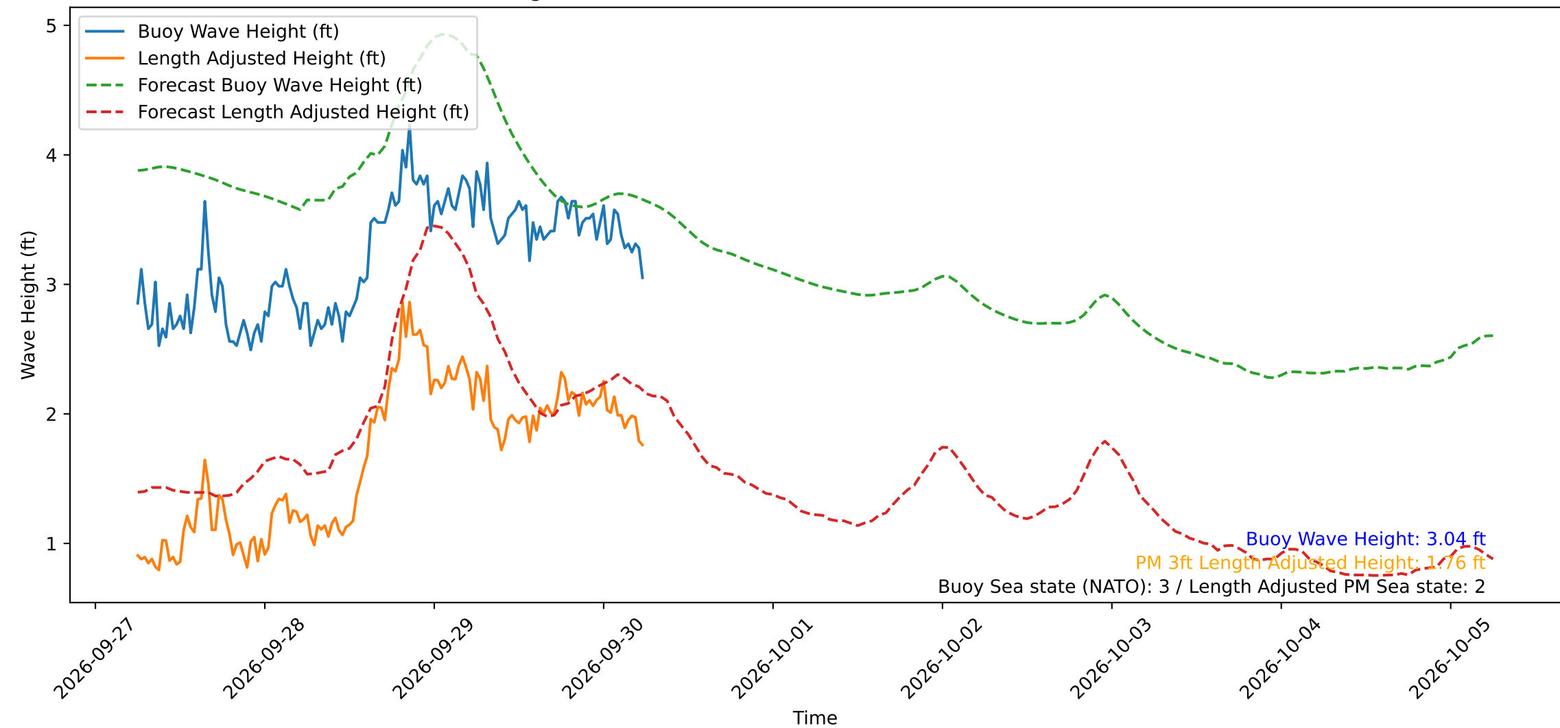
Wave Heights over Time for Oceanside Harbor at 2026-09-30 06:10:30
