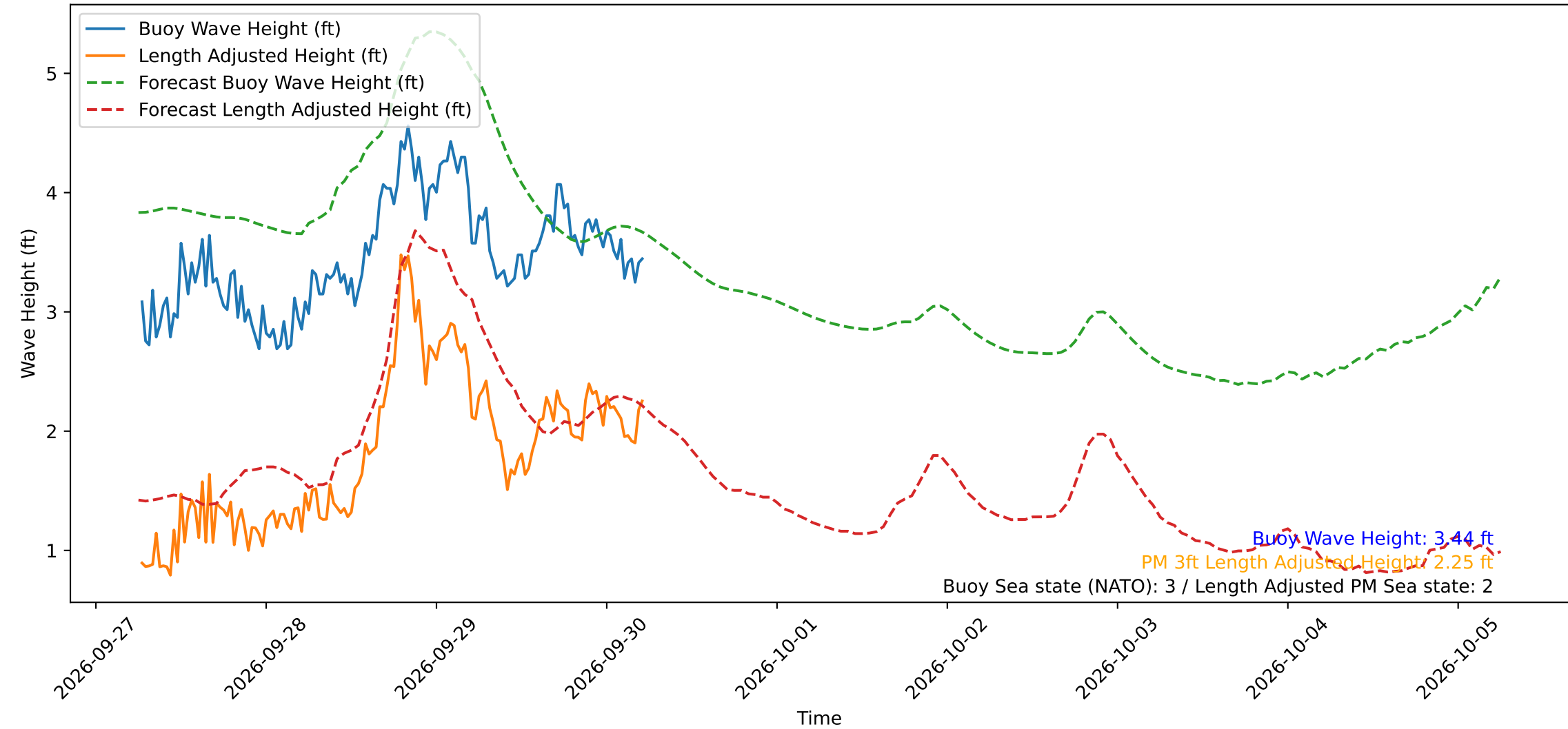
Wave Heights over Time for Green Beach at 2026-09-30 06:11:11
