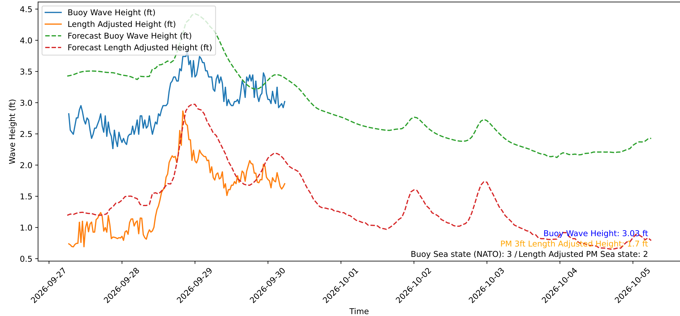
Wave Heights over Time for Red Beach at 2026-09-30 06:10:49
