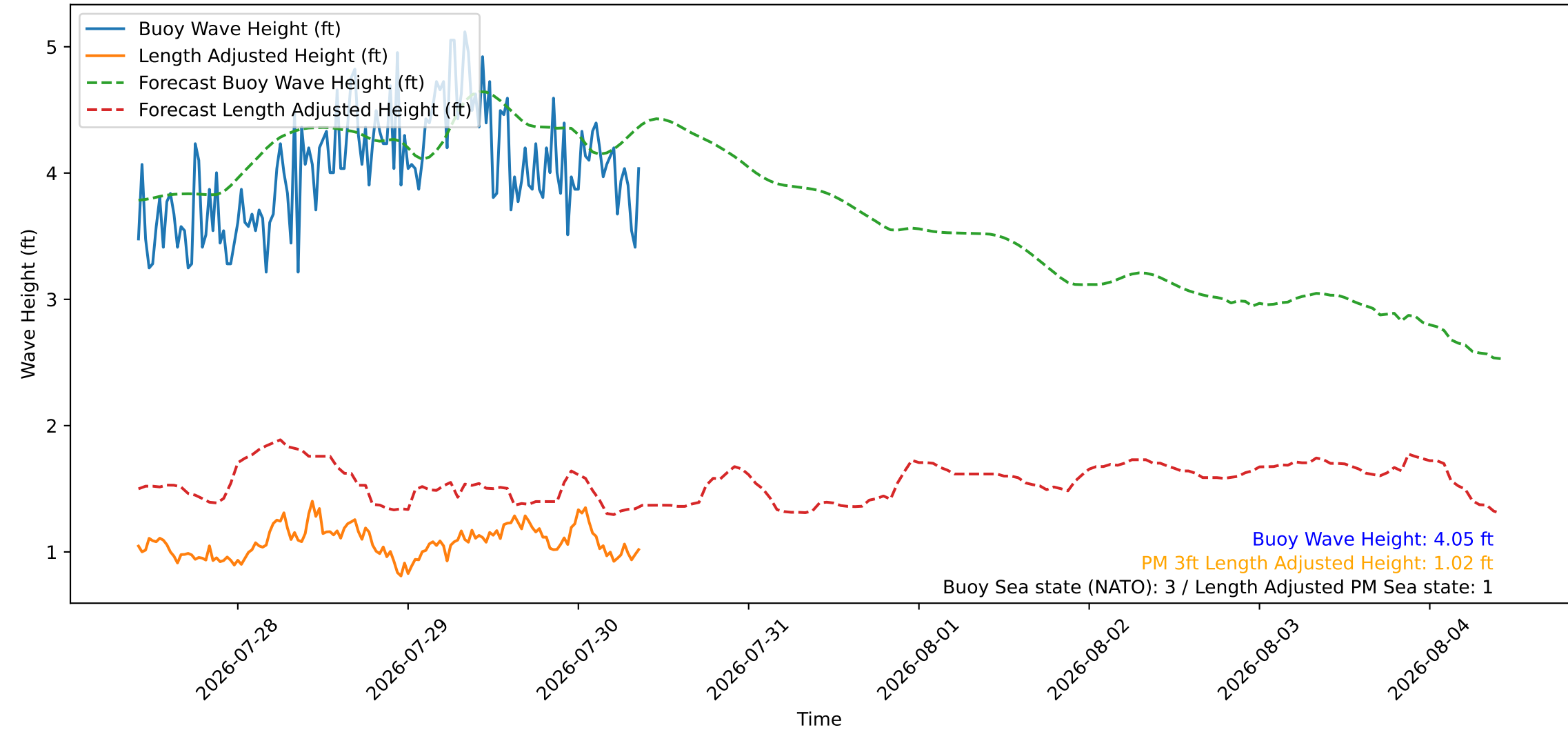
Wave Heights over Time for Red Beach at 2026-07-30 09:40:46
