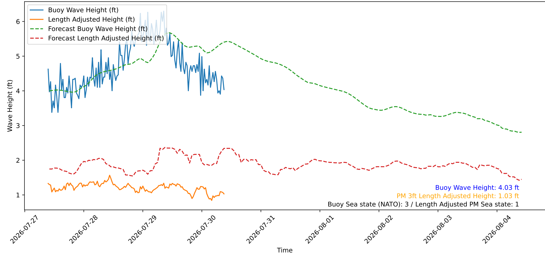
Wave Heights over Time for Green Beach at 2026-07-30 09:41:09
