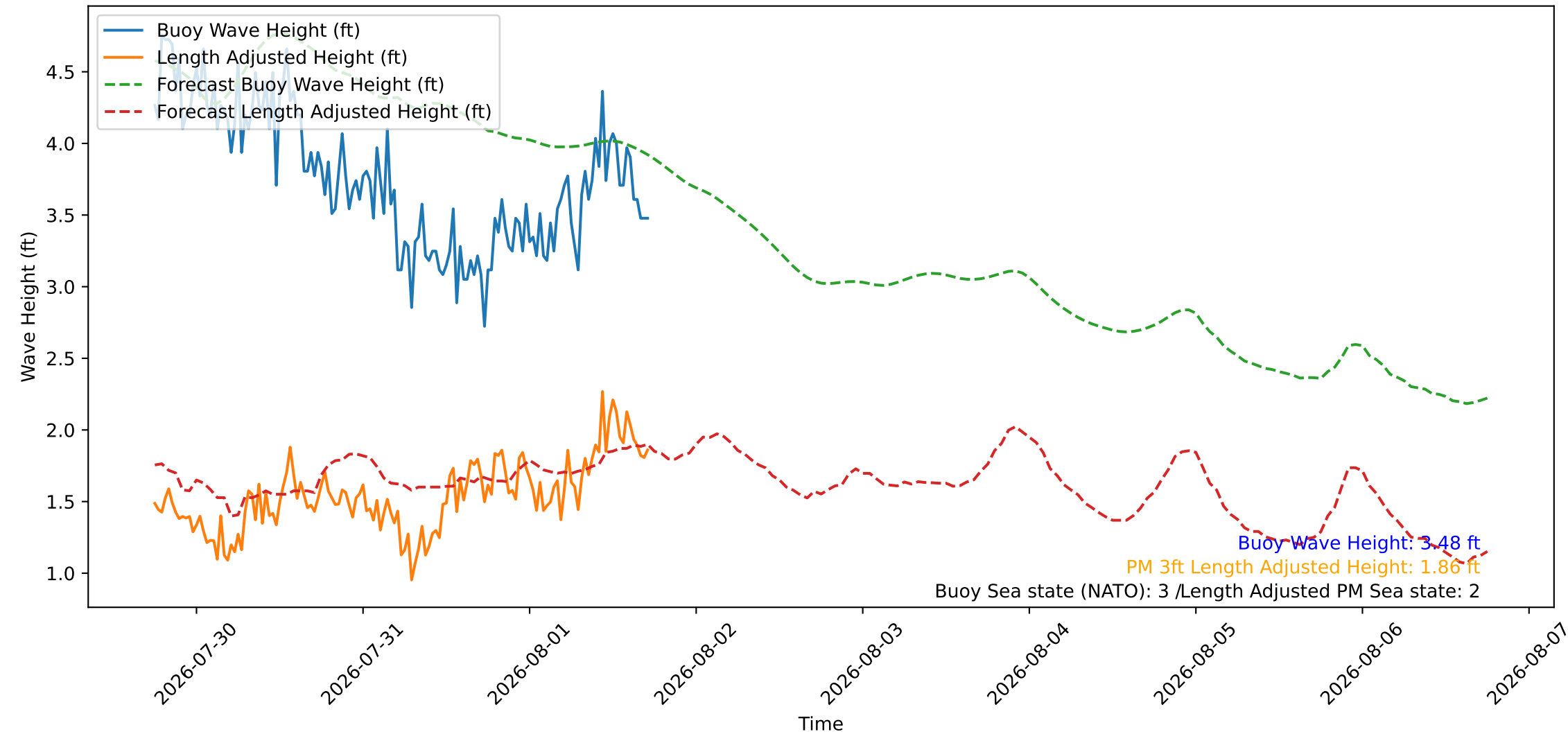
Wave Heights over Time for Oceanside Harbor at 2026-08-01 18:00:26
