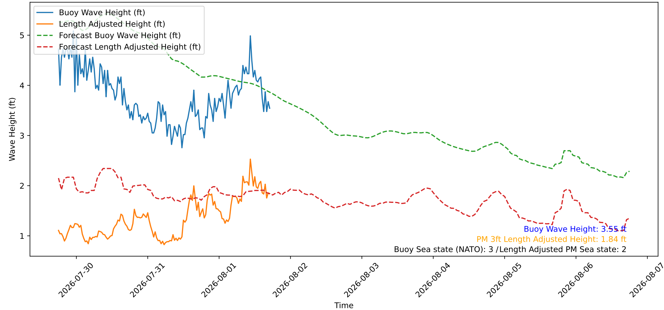
Wave Heights over Time for Green Beach at 2026-08-01 18:01:08
