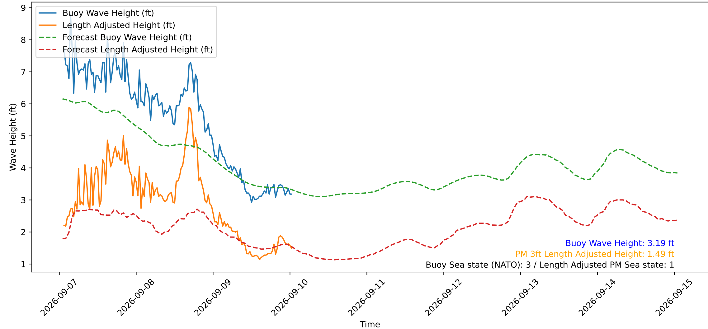
Wave Heights over Time for Green Beach at 2026-09-10 01:21:15
