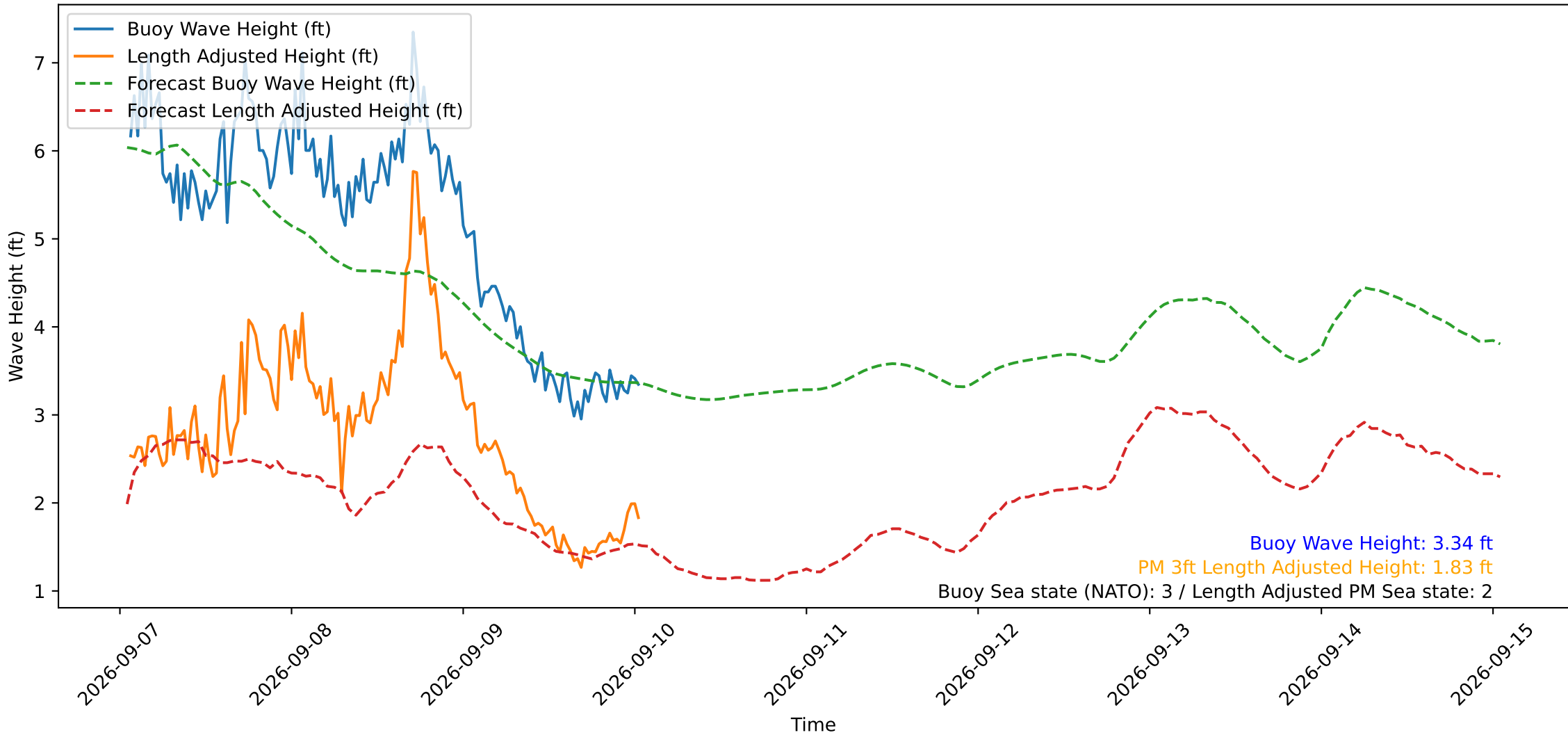
Wave Heights over Time for Oceanside Harbor at 2026-09-10 01:20:30
