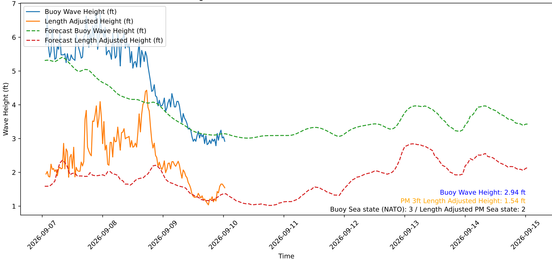
Wave Heights over Time for Red Beach at 2026-09-10 01:20:51
