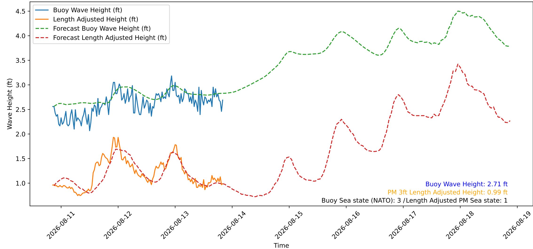
Wave Heights over Time for Oceanside Harbor at 2026-08-13 20:40:27
