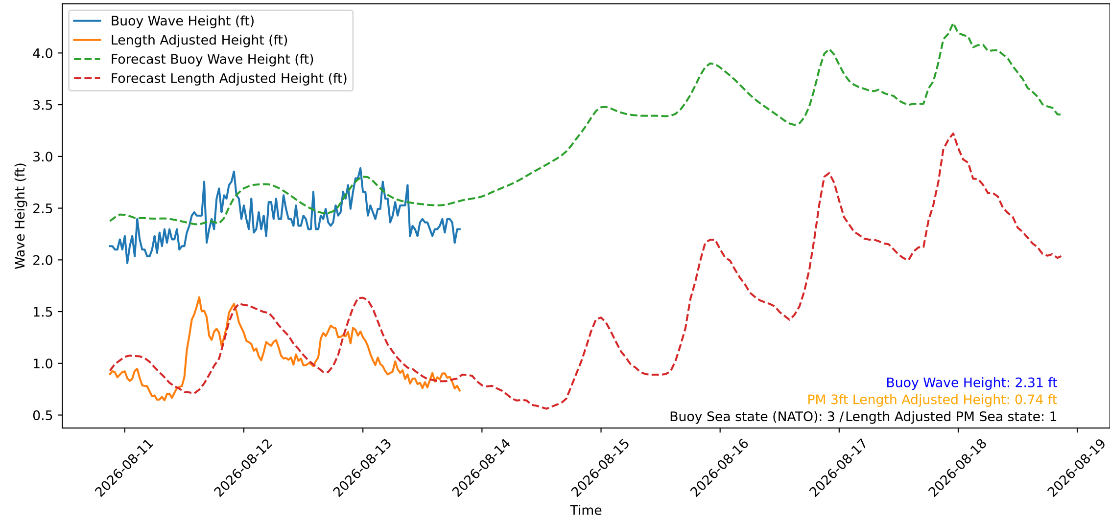
Wave Heights over Time for Red Beach at 2026-08-13 20:40:46
