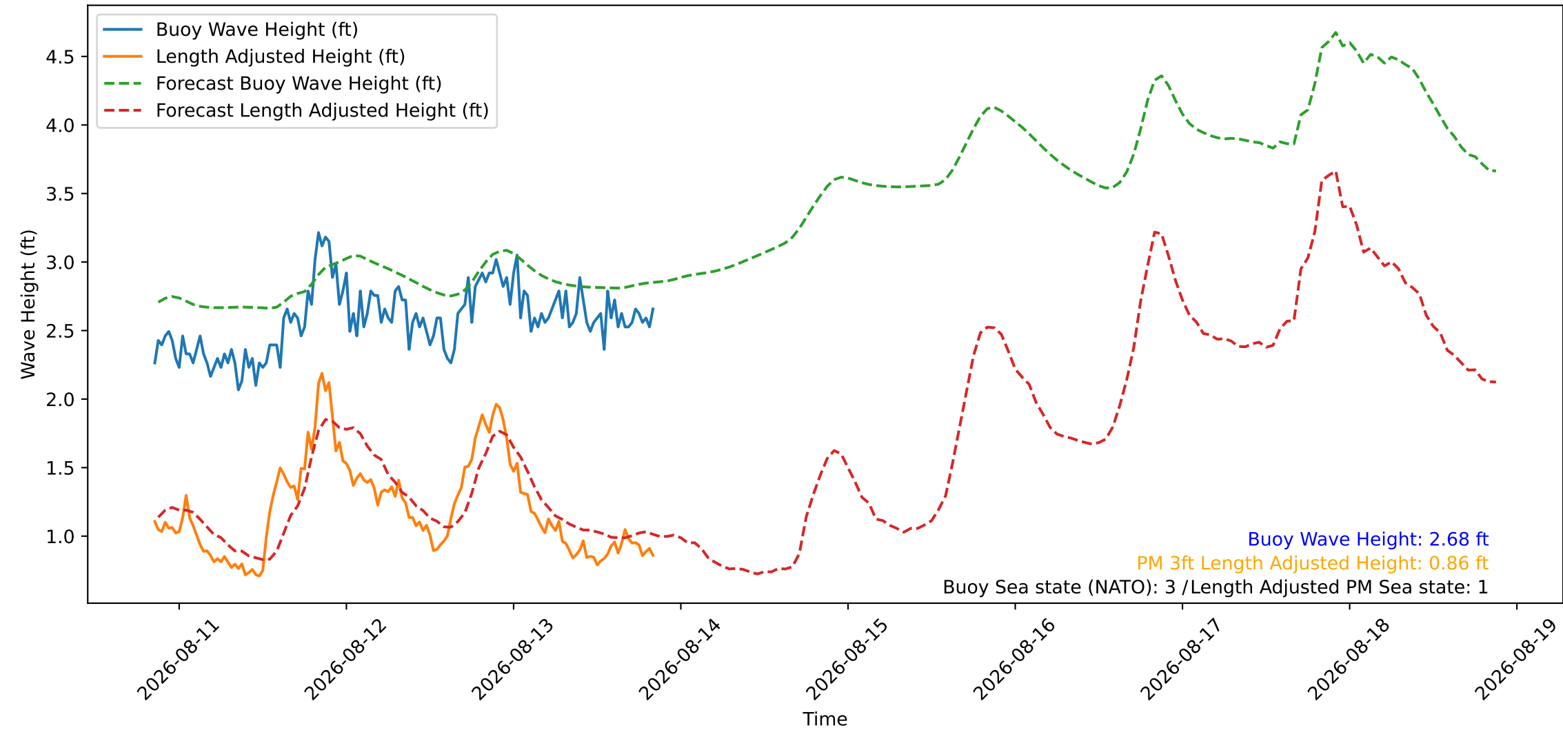
Wave Heights over Time for Green Beach at 2026-08-13 20:41:09
