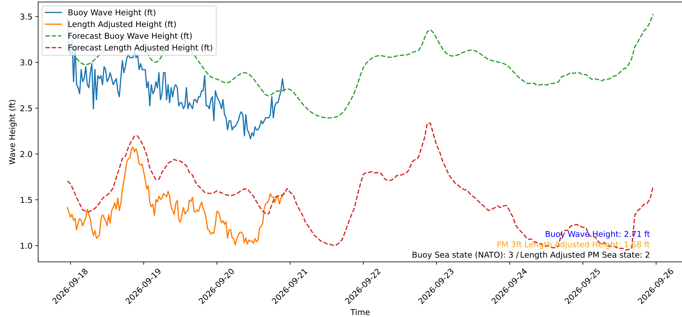
Wave Heights over Time for Green Beach at 2026-09-20 22:51:14
