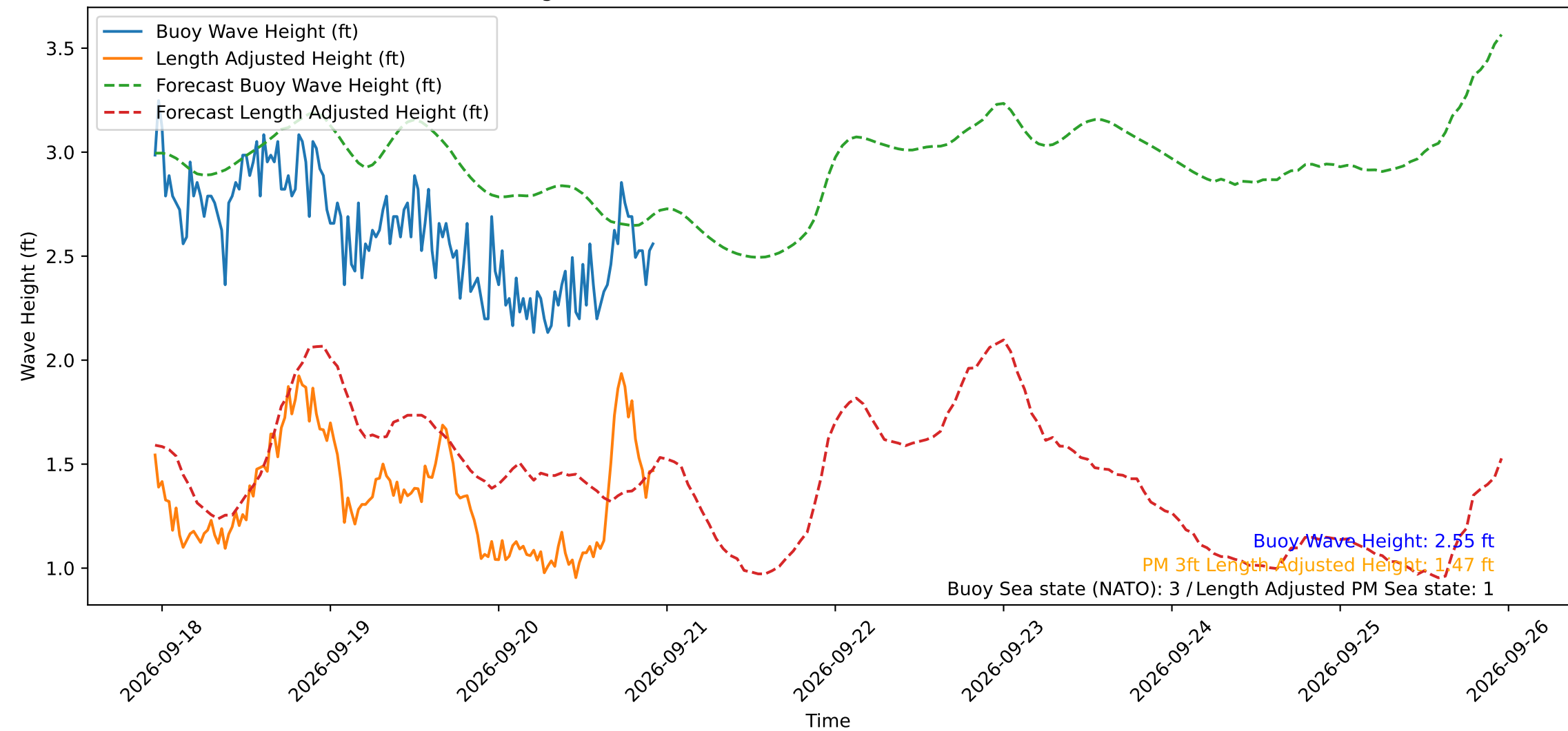
Wave Heights over Time for Oceanside Harbor at 2026-09-20 22:50:29
