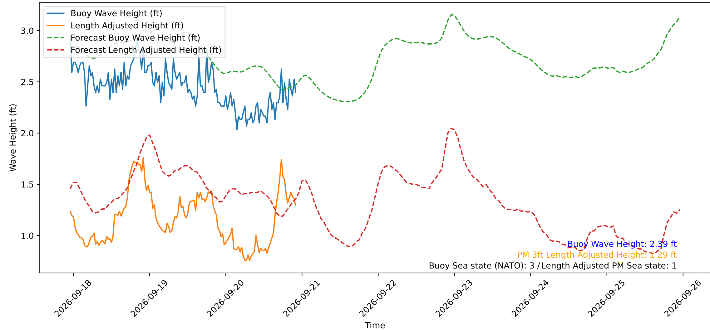
Wave Heights over Time for Red Beach at 2026-09-20 22:50:50
