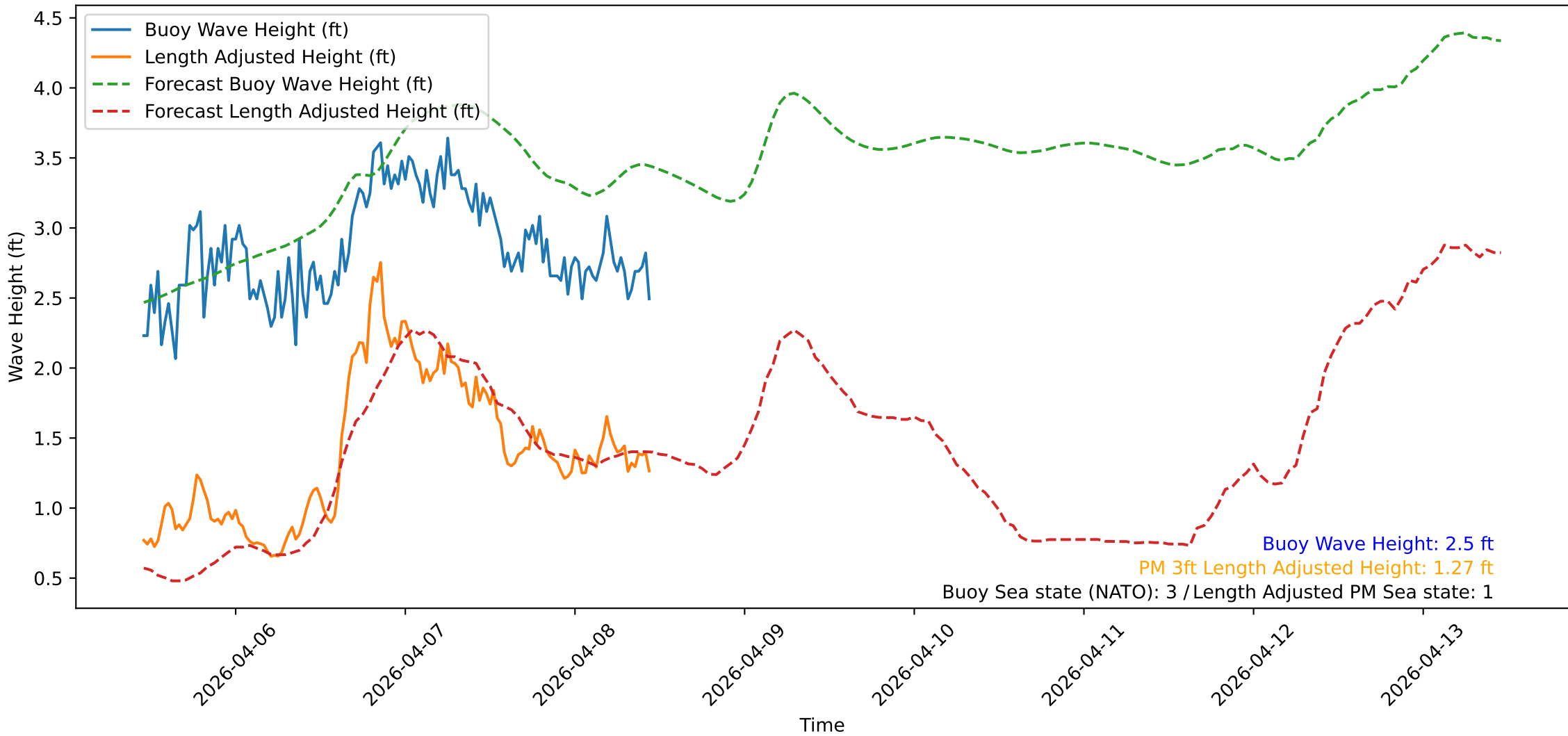
Wave Heights over Time for Oceanside Harbor at 2026-04-08 11:10:31
