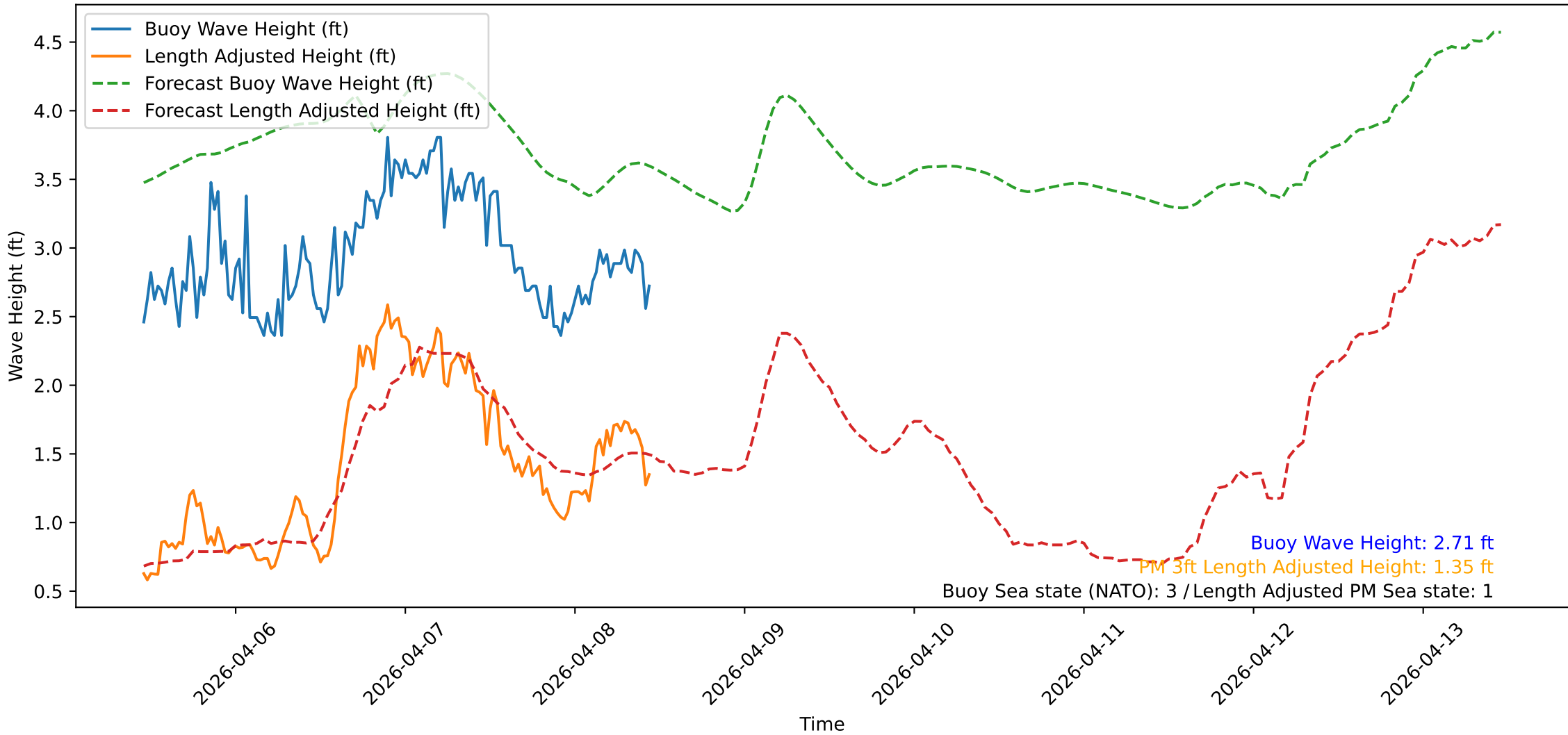
Wave Heights over Time for Green Beach at 2026-04-08 11:11:09
