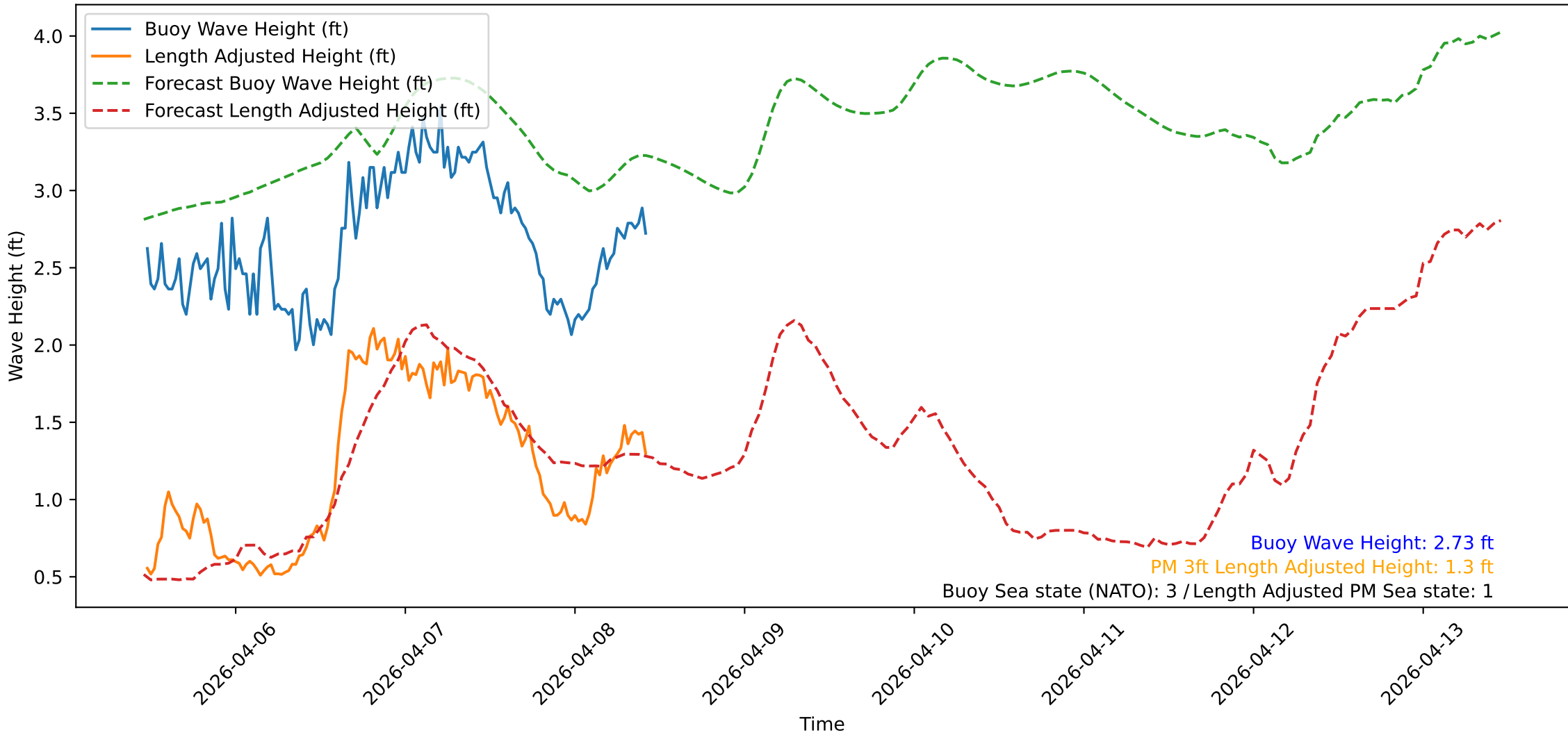
Wave Heights over Time for Red Beach at 2026-04-08 11:10:47
