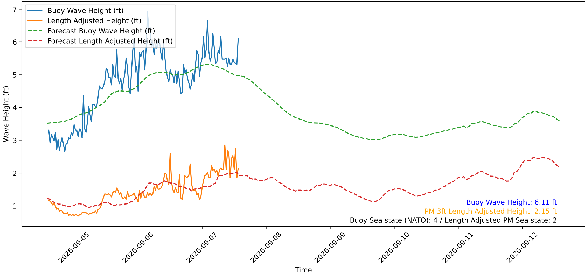
Wave Heights over Time for Red Beach at 2026-09-07 14:20:50
