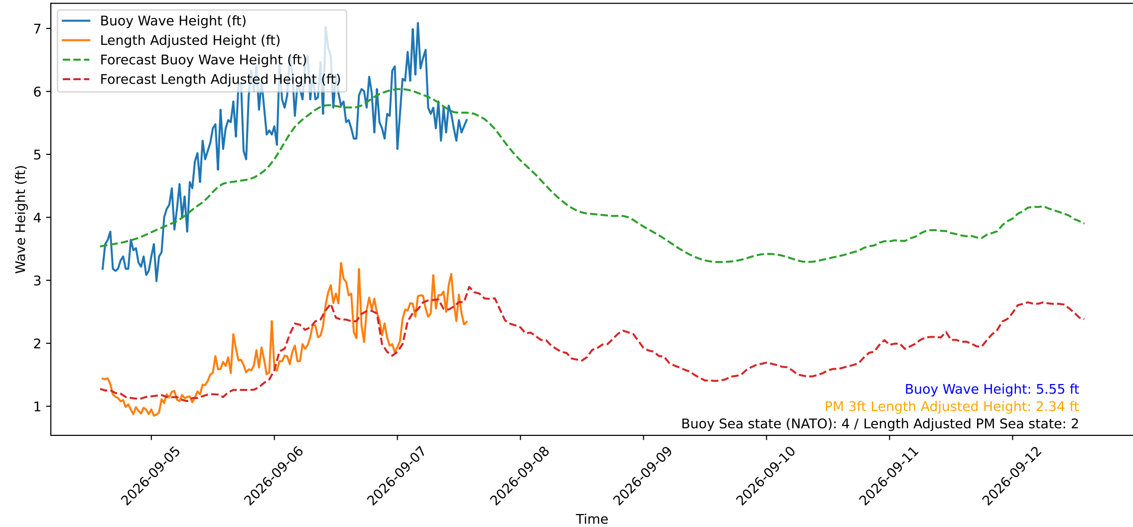
Wave Heights over Time for Oceanside Harbor at 2026-09-07 14:20:29
