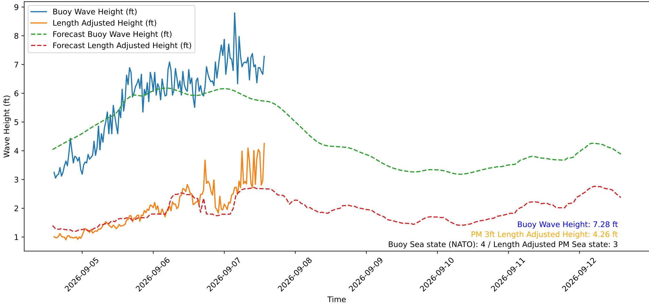
Wave Heights over Time for Green Beach at 2026-09-07 14:21:14
