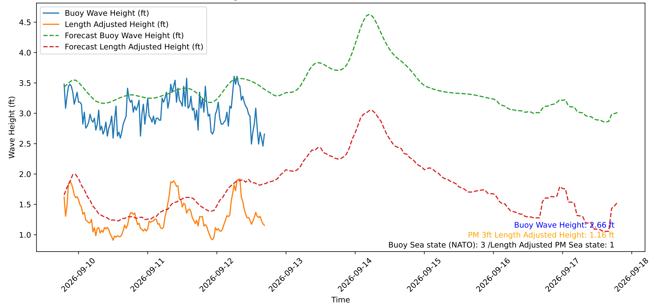
Wave Heights over Time for Green Beach at 2026-09-12 18:31:11
