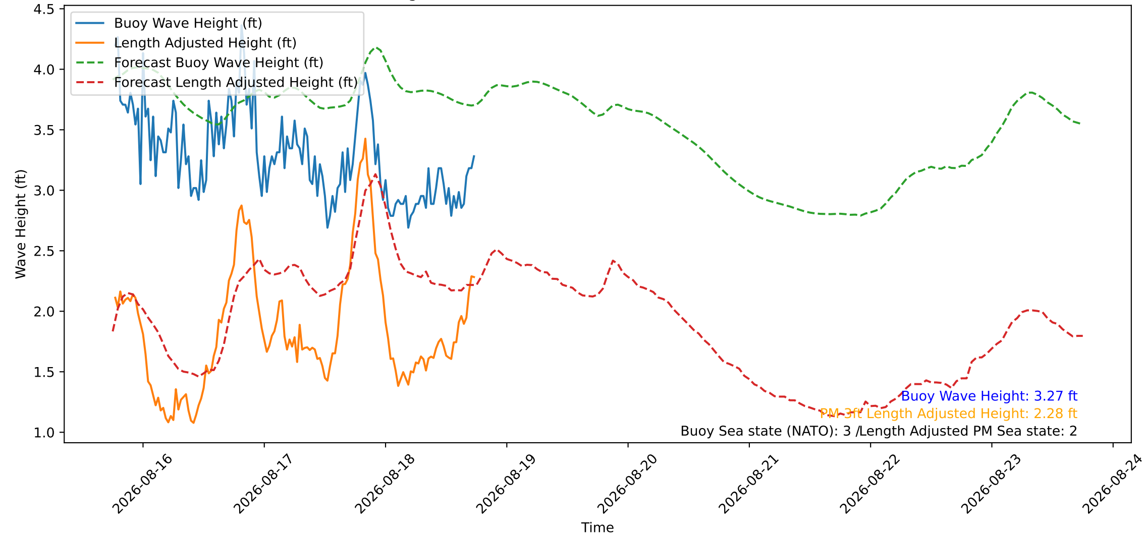
Wave Heights over Time for Green Beach at 2026-08-18 18:21:12
