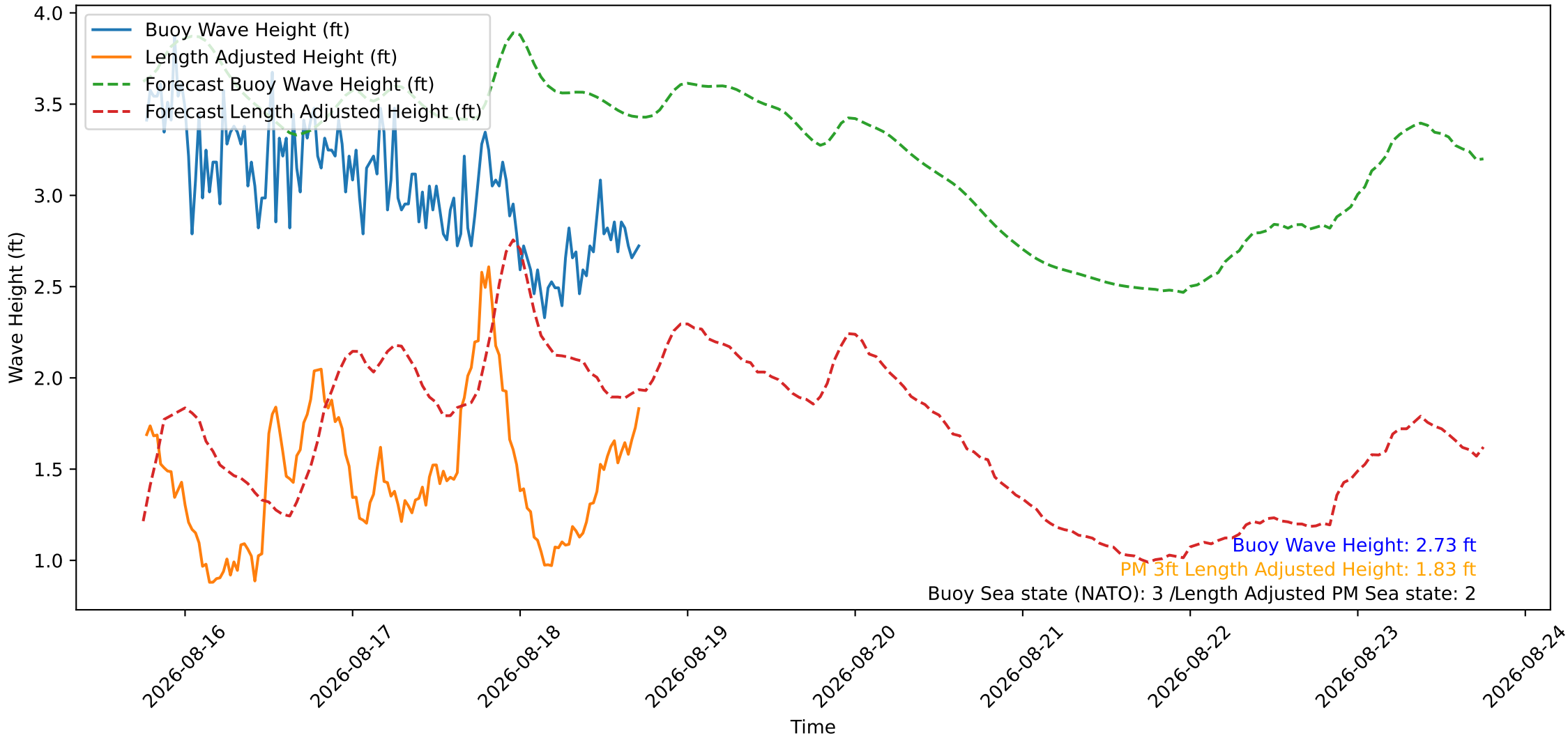
Wave Heights over Time for Red Beach at 2026-08-18 18:20:48
