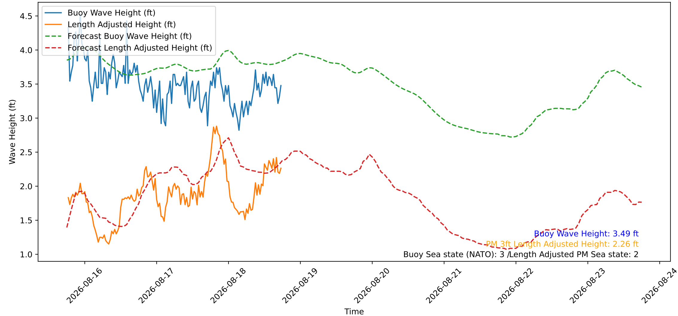
Wave Heights over Time for Oceanside Harbor at 2026-08-18 18:20:27
