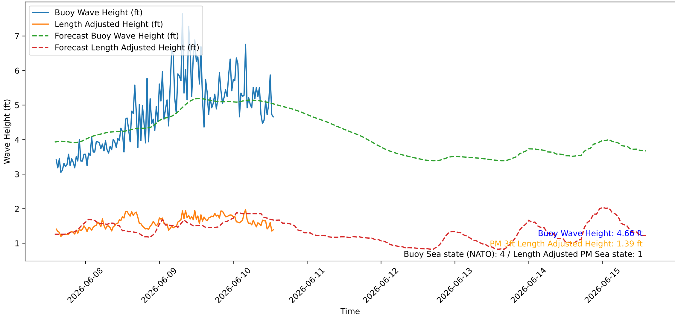
Wave Heights over Time for Red Beach at 2026-06-10 14:00:46
