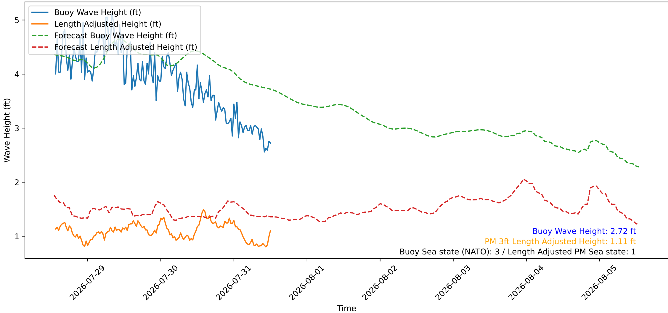
Wave Heights over Time for Red Beach at 2026-07-31 13:00:45
