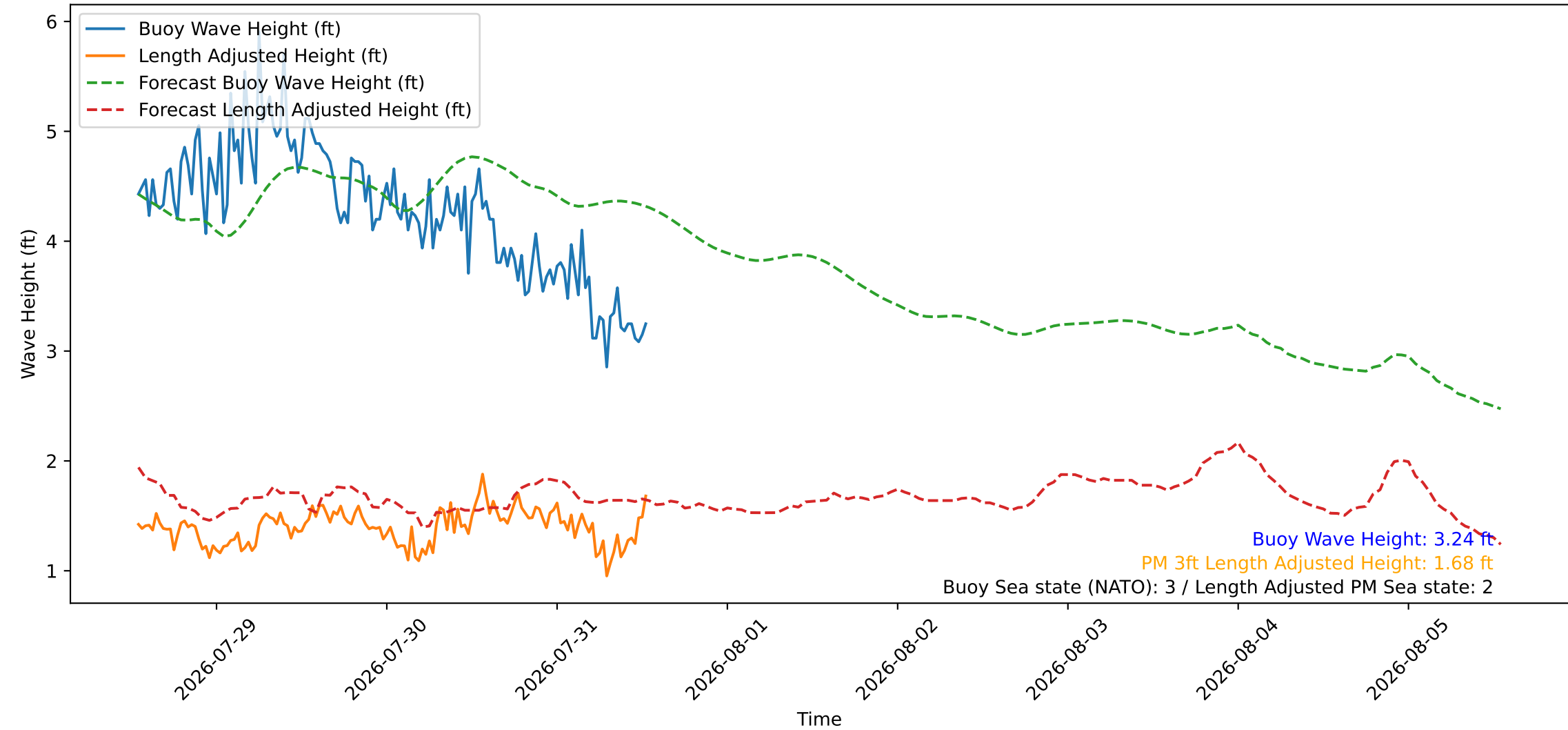
Wave Heights over Time for Oceanside Harbor at 2026-07-31 13:00:26
