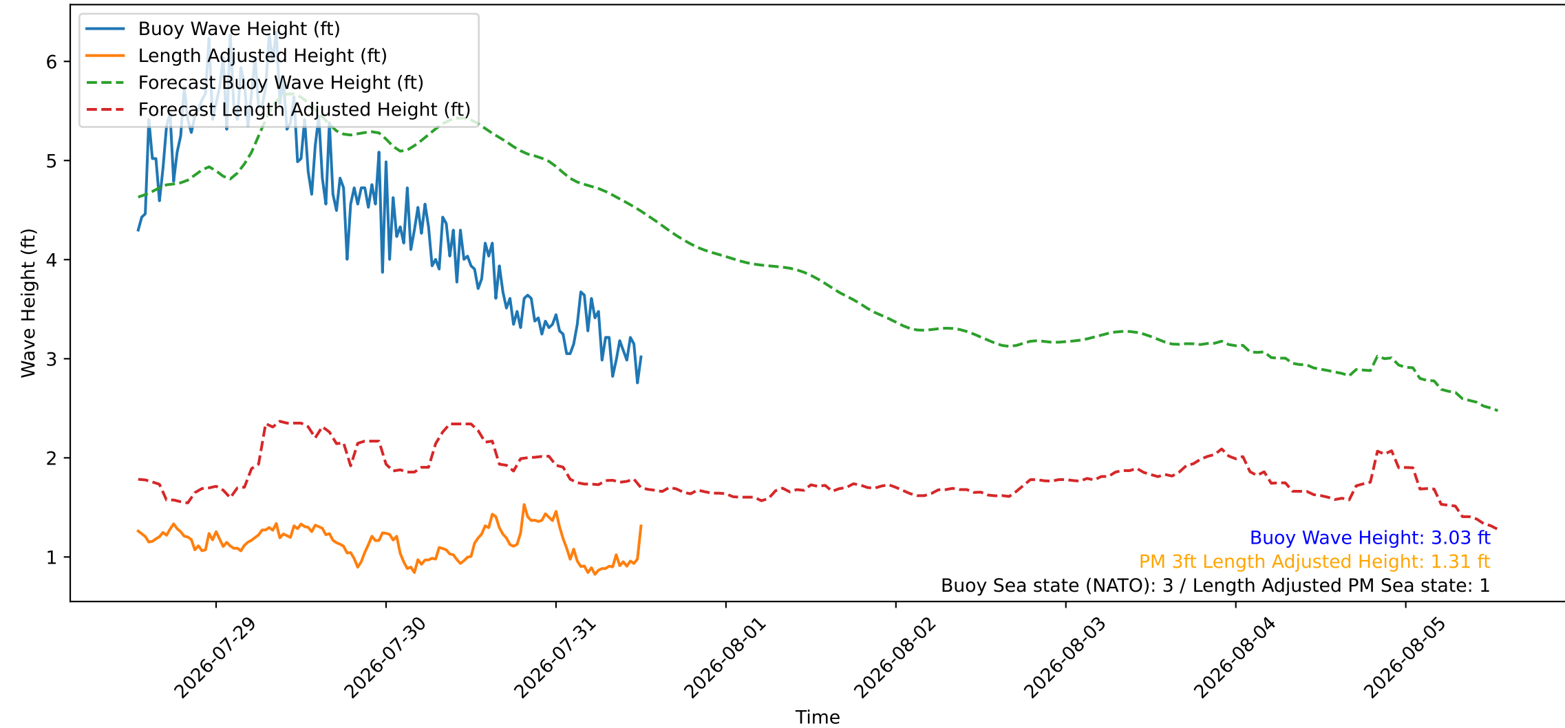
Wave Heights over Time for Green Beach at 2026-07-31 13:01:08
