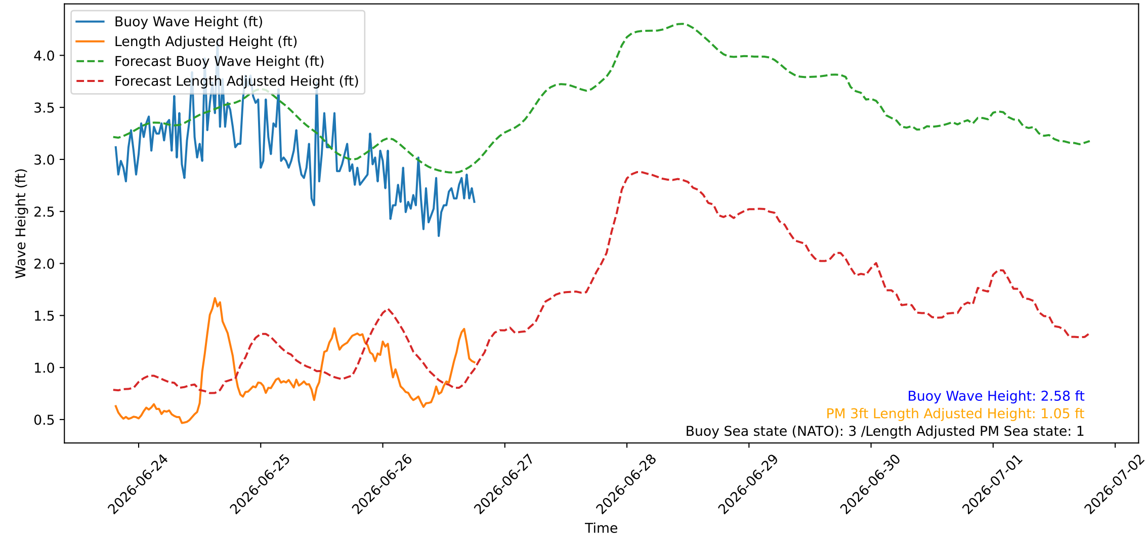
Wave Heights over Time for Red Beach at 2026-06-26 19:20:47
