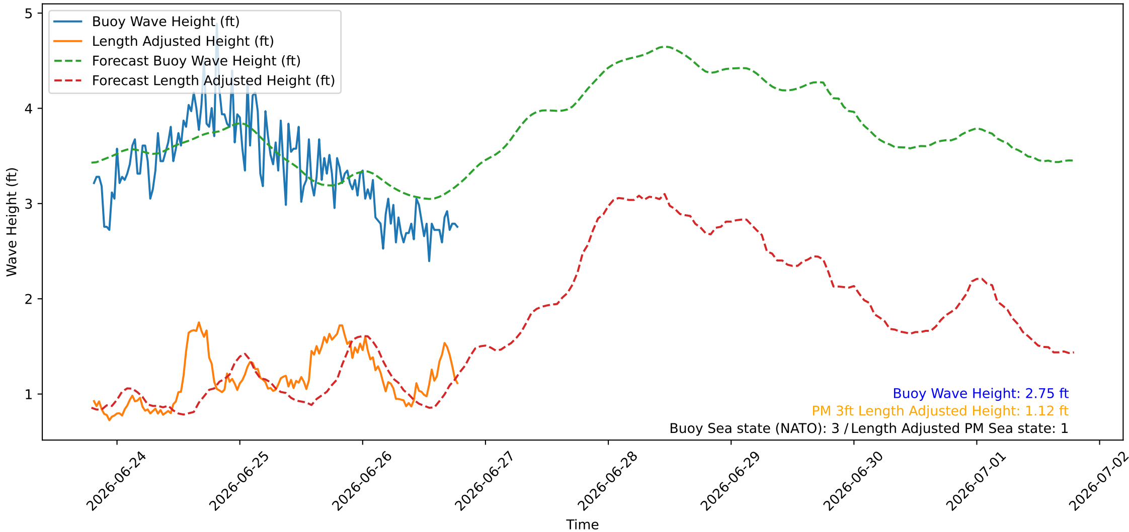
Wave Heights over Time for Oceanside Harbor at 2026-06-26 19:20:27
