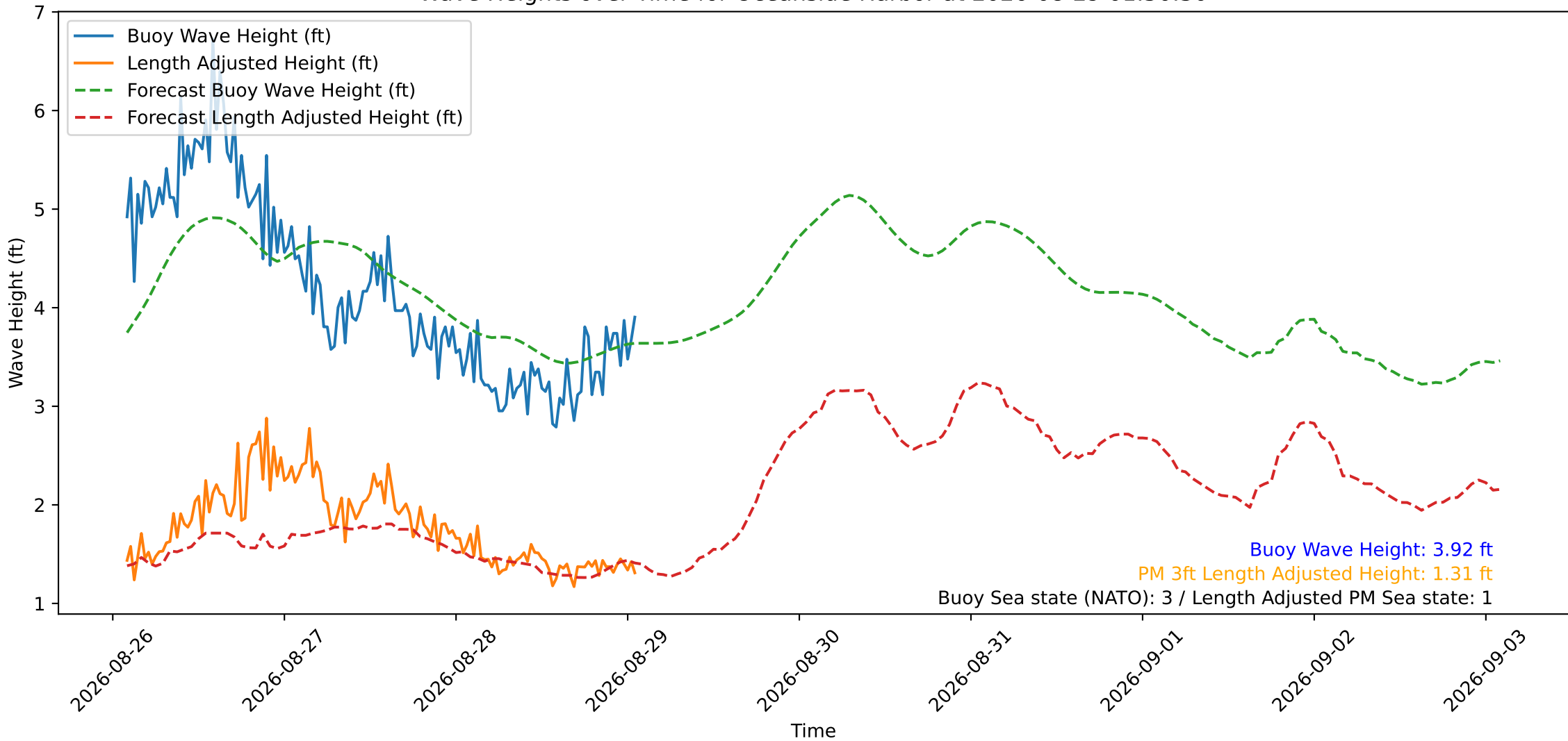
Wave Heights over Time for Oceanside Harbor at 2026-08-29 01:50:30
