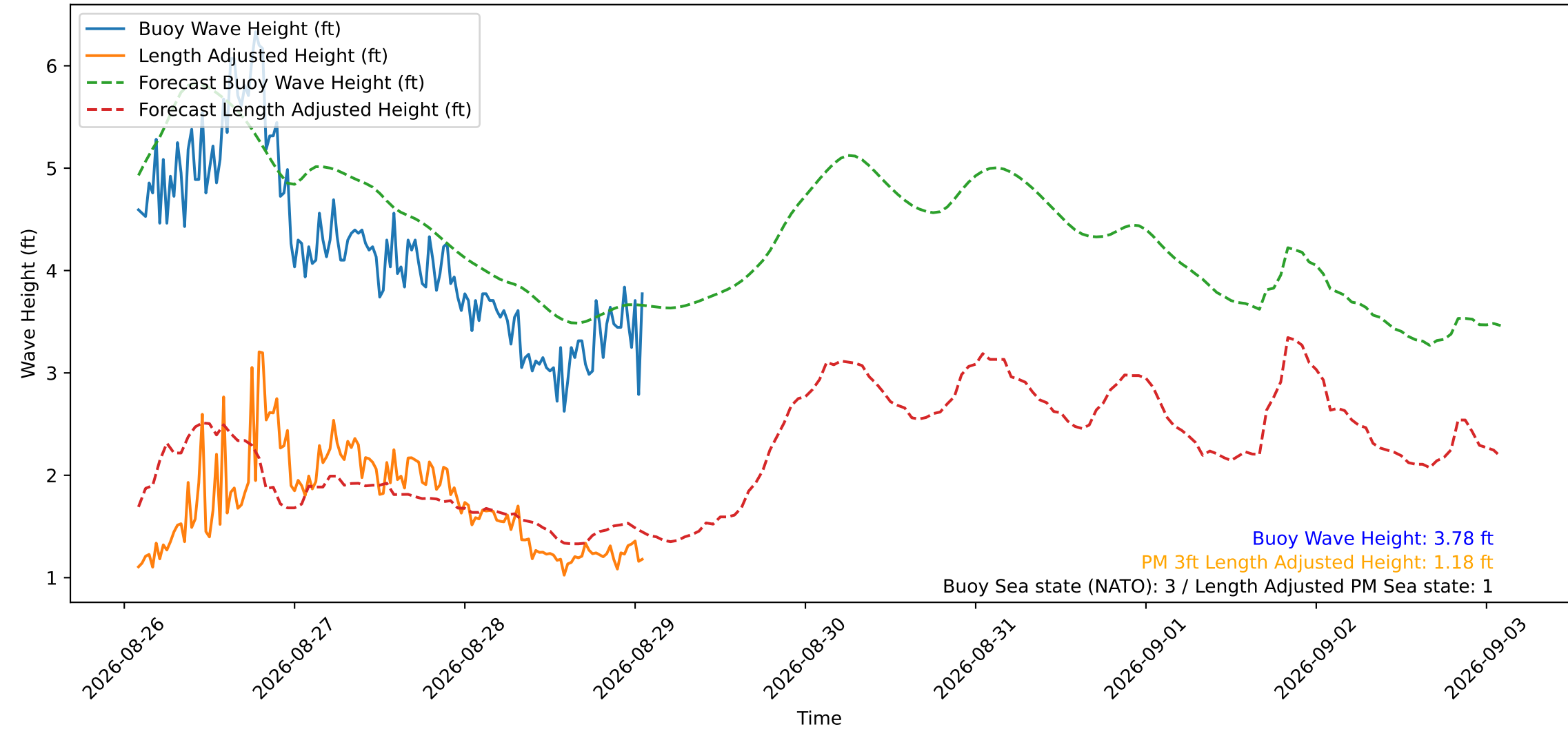
Wave Heights over Time for Green Beach at 2026-08-29 01:51:14
