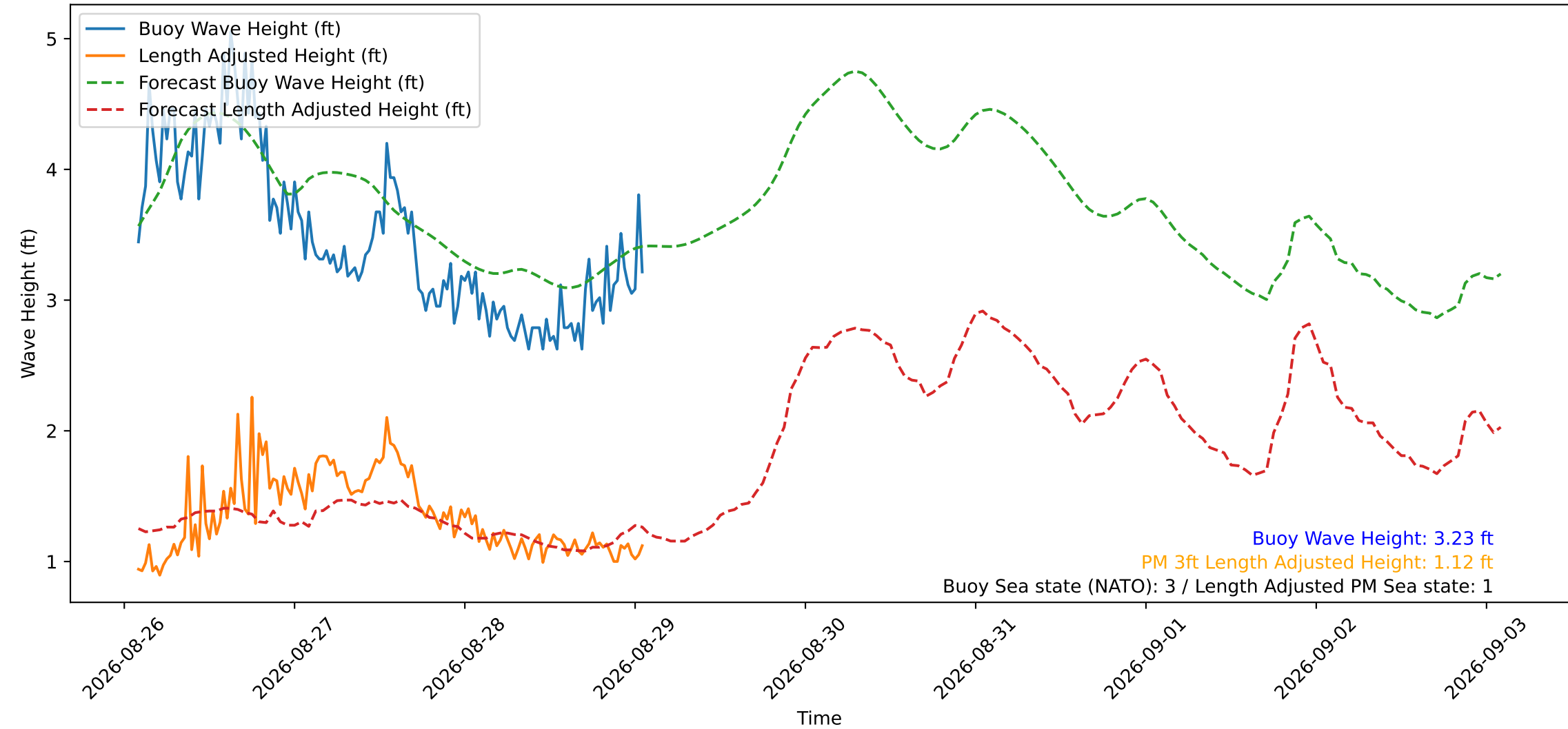
Wave Heights over Time for Red Beach at 2026-08-29 01:50:51
