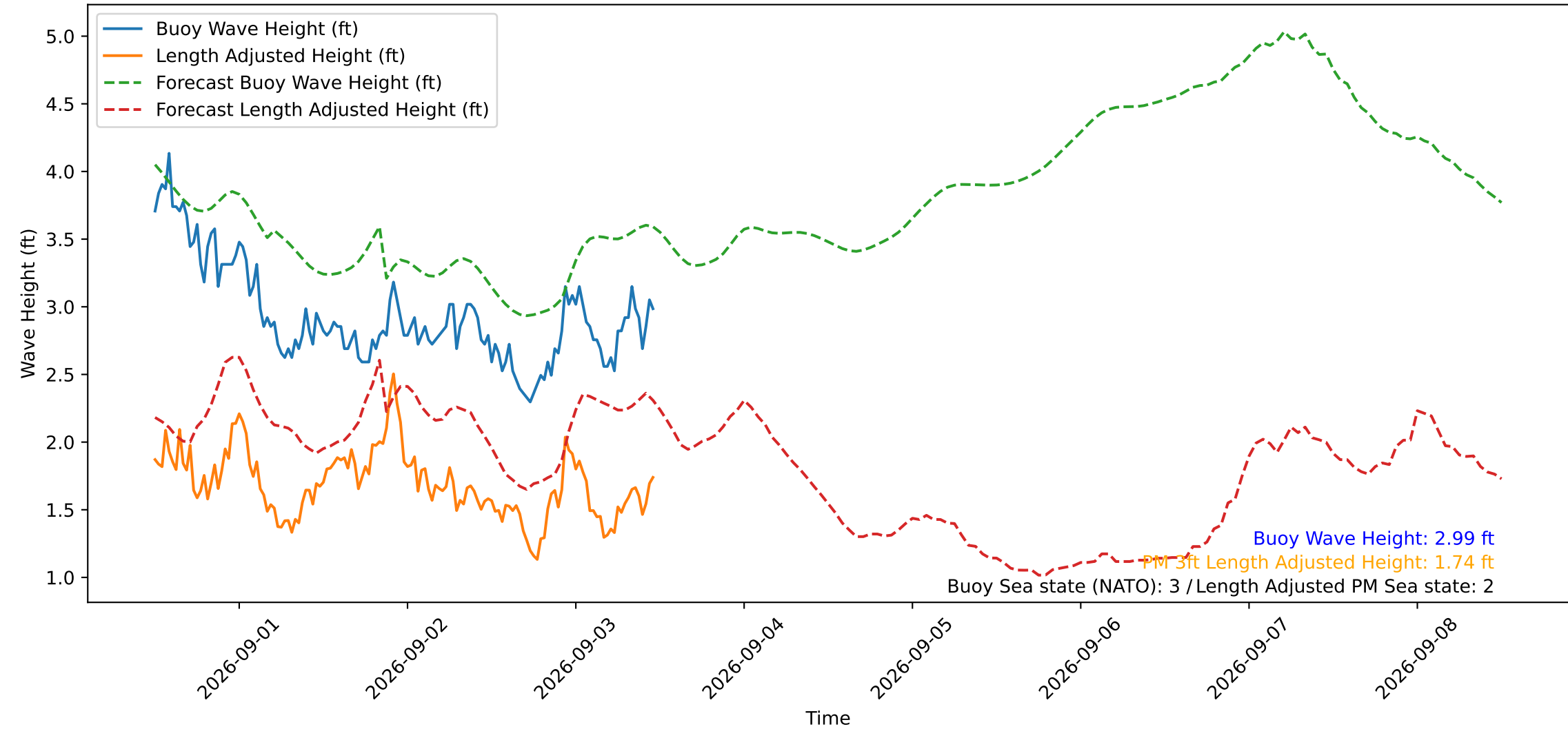
Wave Heights over Time for Red Beach at 2026-09-03 11:40:50
