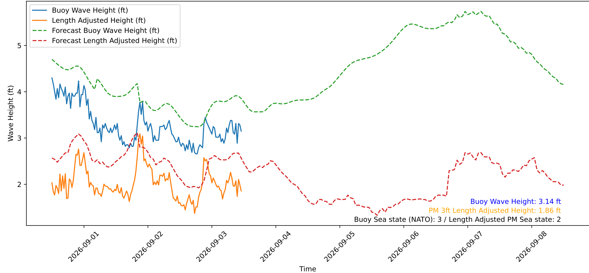
Wave Heights over Time for Green Beach at 2026-09-03 11:41:12
