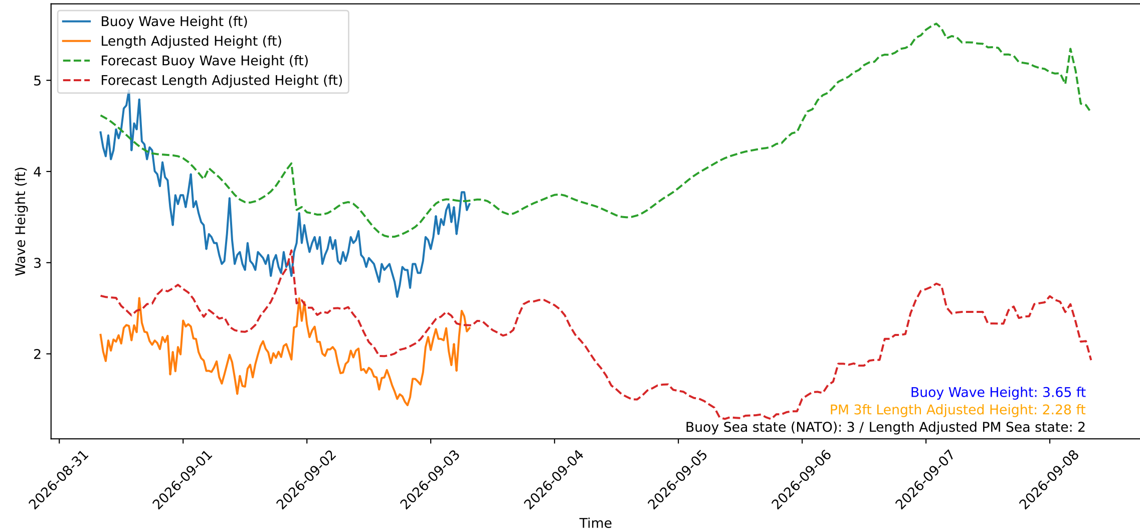
Wave Heights over Time for Oceanside Harbor at 2026-09-03 08:10:30
