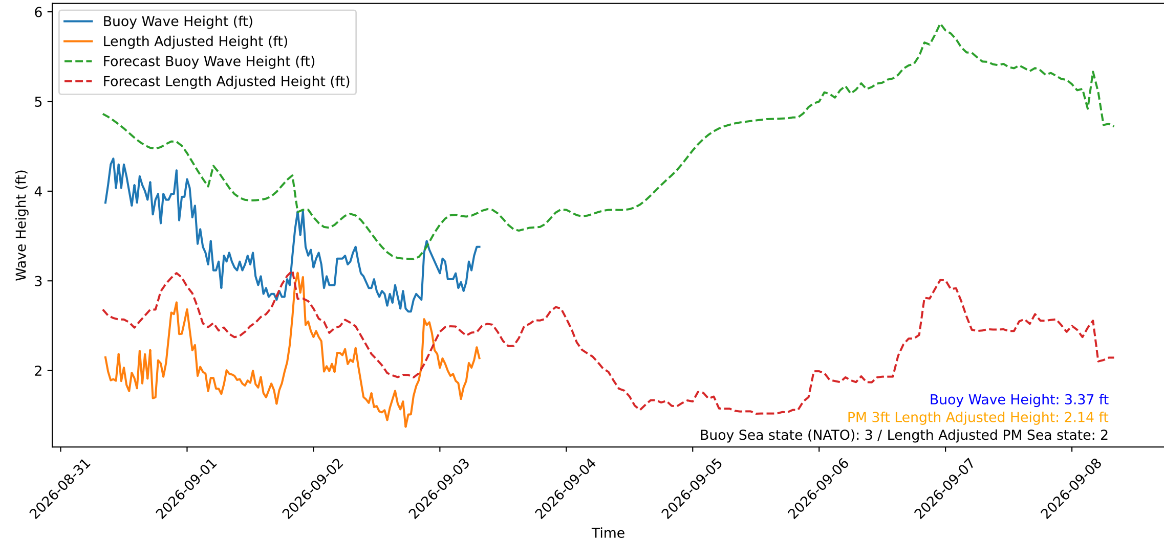
Wave Heights over Time for Green Beach at 2026-09-03 08:11:13
