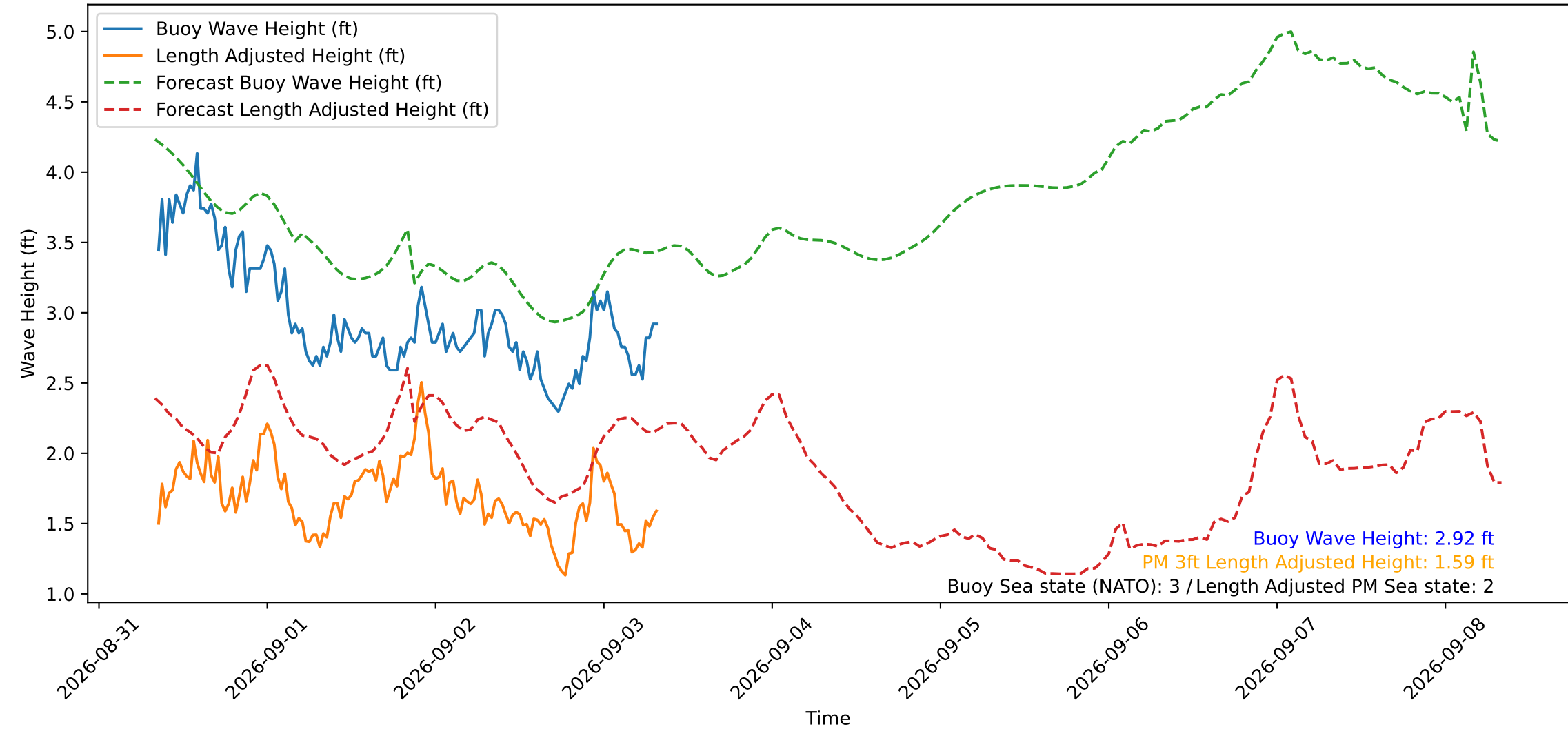
Wave Heights over Time for Red Beach at 2026-09-03 08:10:50
