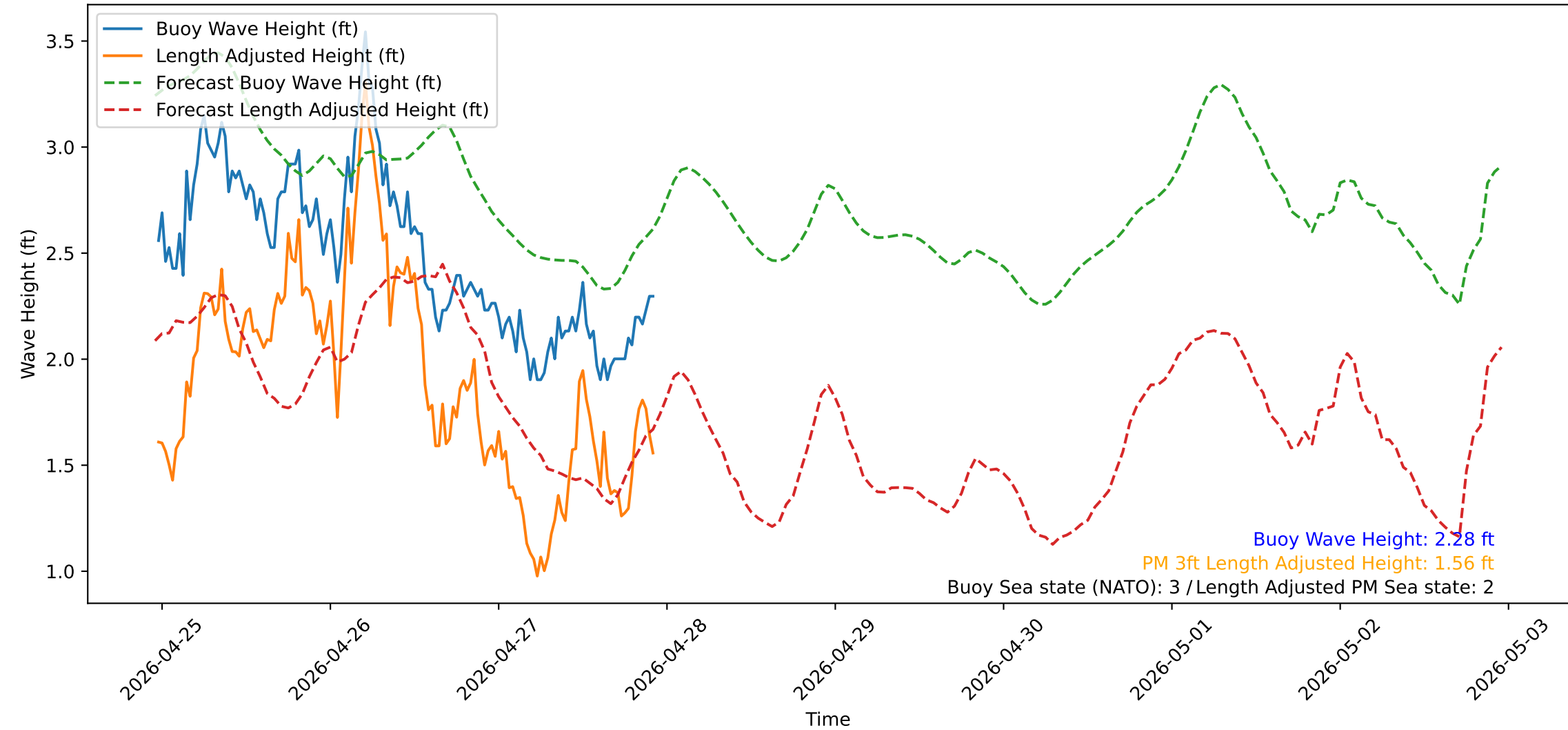
Wave Heights over Time for Red Beach at 2026-04-27 23:00:51
