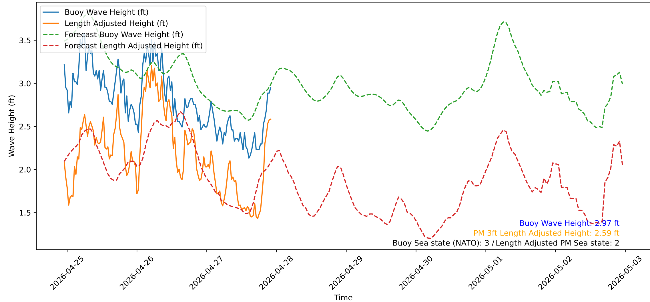
Wave Heights over Time for Green Beach at 2026-04-27 23:01:12
