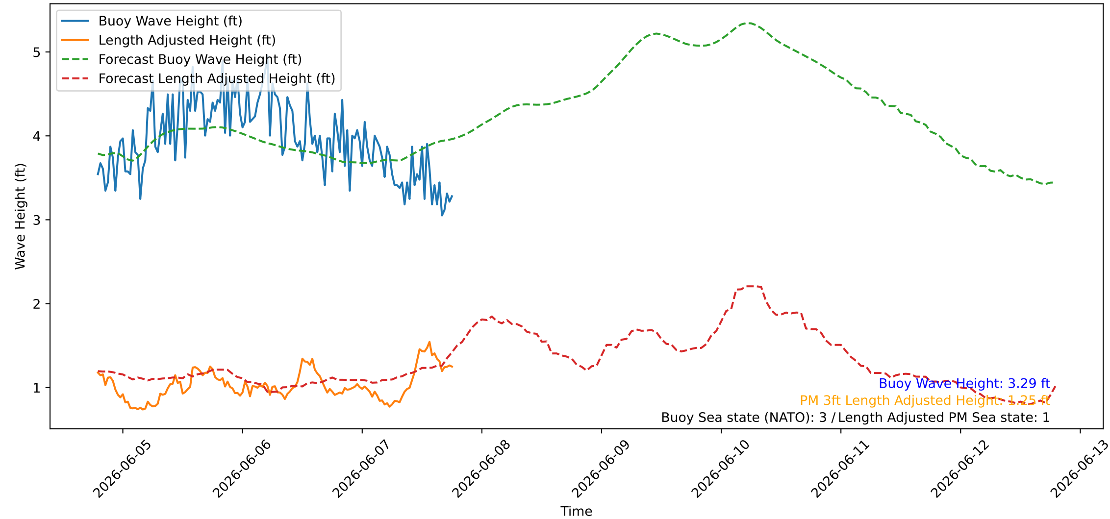
Wave Heights over Time for Red Beach at 2026-06-07 18:50:46
