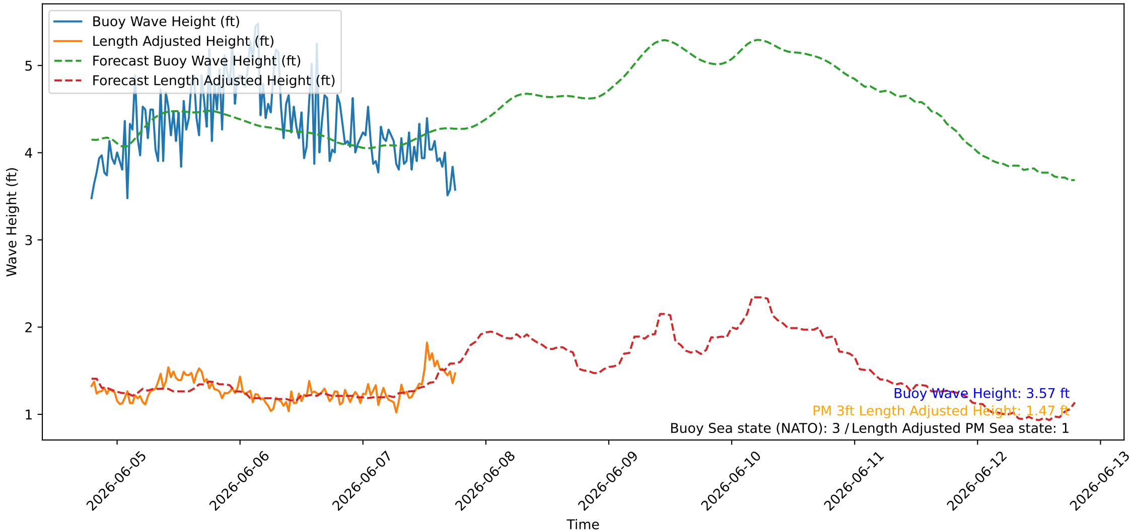
Wave Heights over Time for Oceanside Harbor at 2026-06-07 18:50:25
