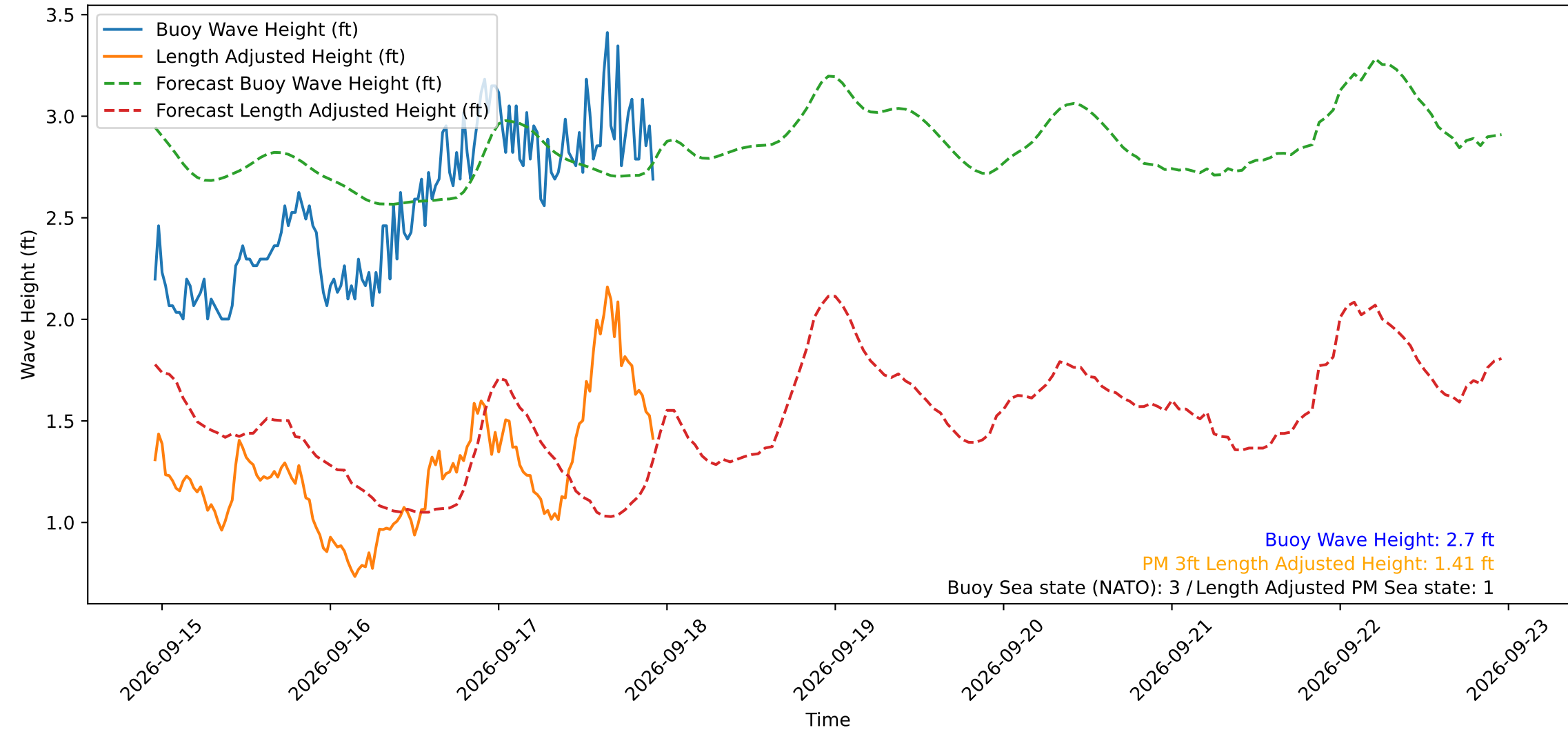
Wave Heights over Time for Red Beach at 2026-09-17 22:50:50
