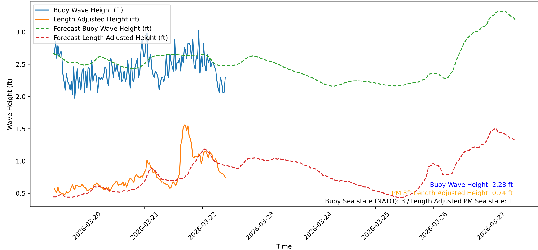
Wave Heights over Time for Oceanside Harbor at 2026-03-22 10:20:32
