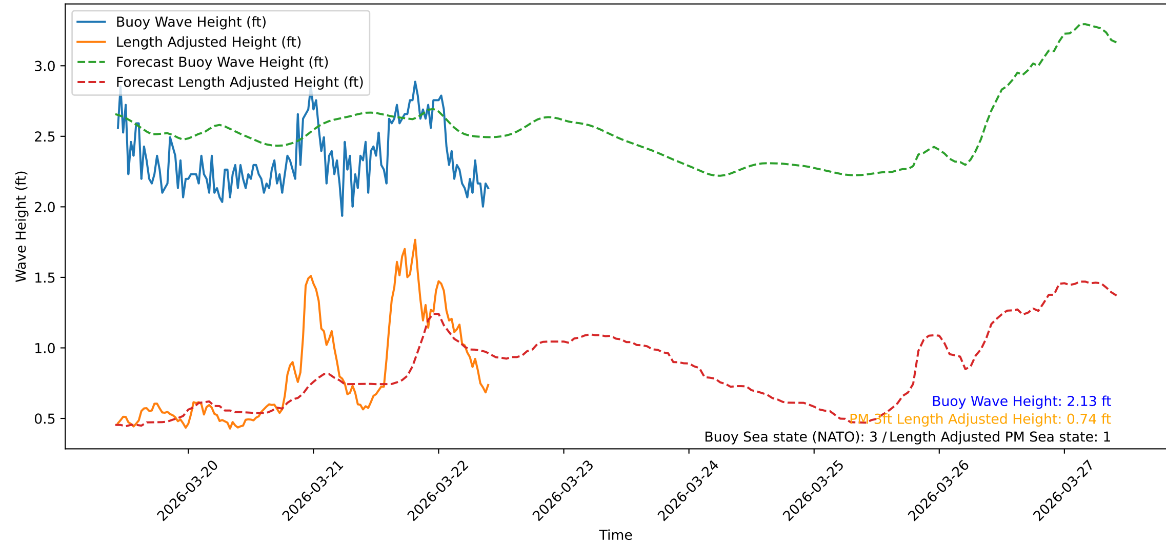
Wave Heights over Time for Green Beach at 2026-03-22 10:21:10
