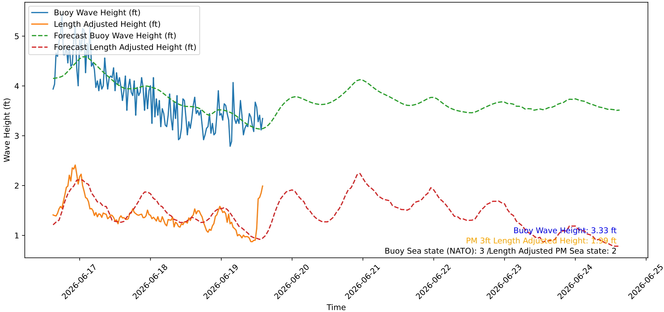
Wave Heights over Time for Oceanside Harbor at 2026-06-19 14:50:26
