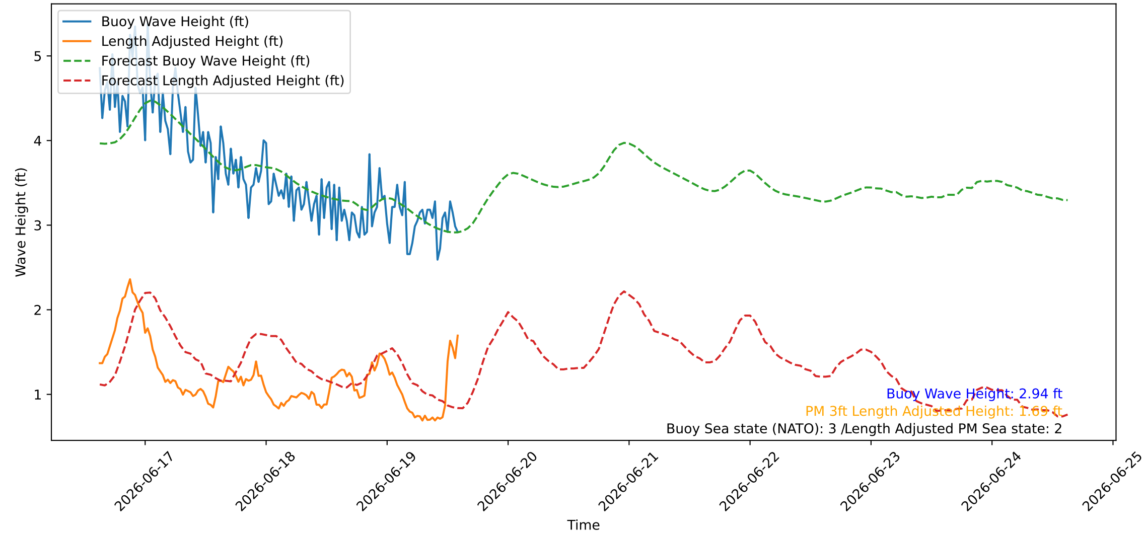
Wave Heights over Time for Red Beach at 2026-06-19 14:50:46
