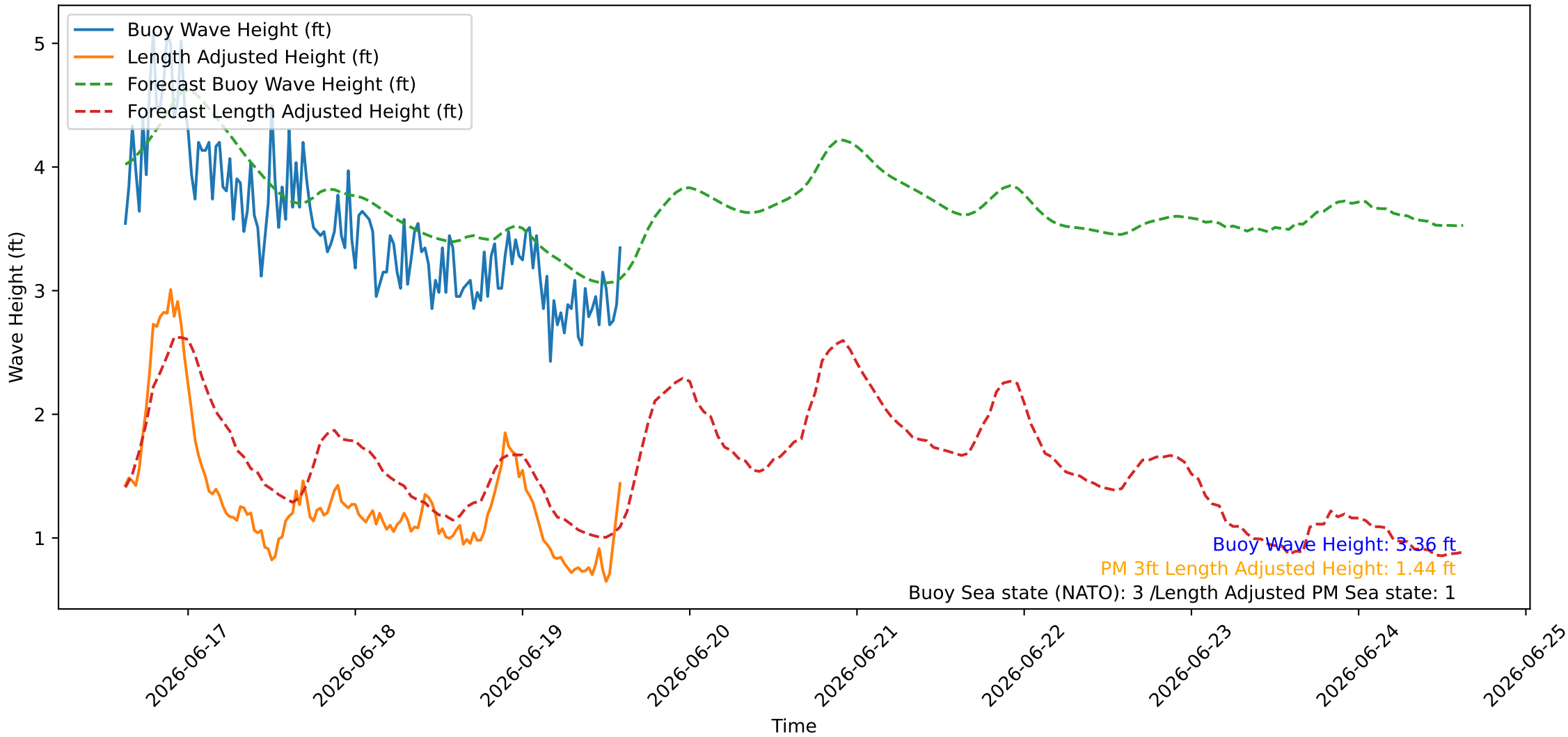
Wave Heights over Time for Green Beach at 2026-06-19 14:51:08
