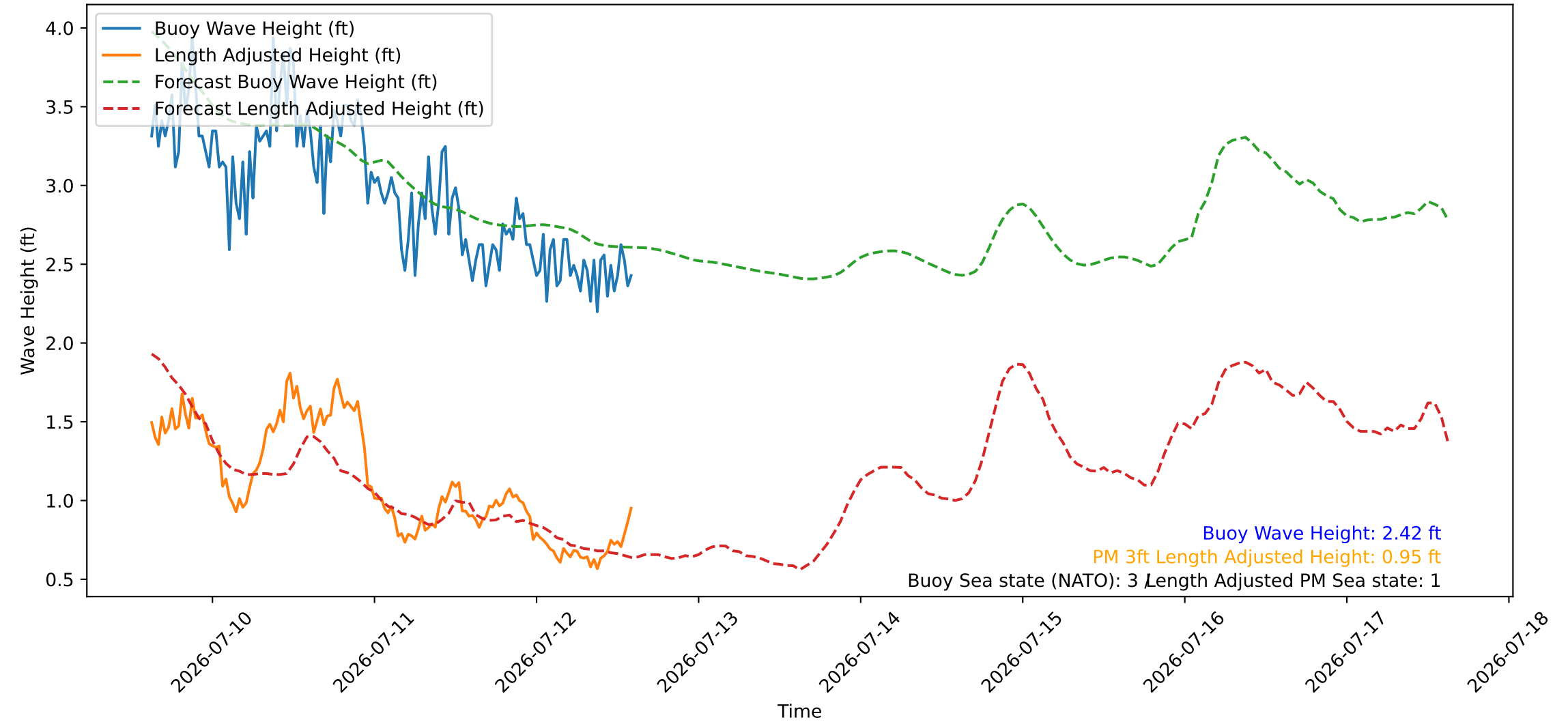
Wave Heights over Time for Red Beach at 2026-07-12 14:50:47
