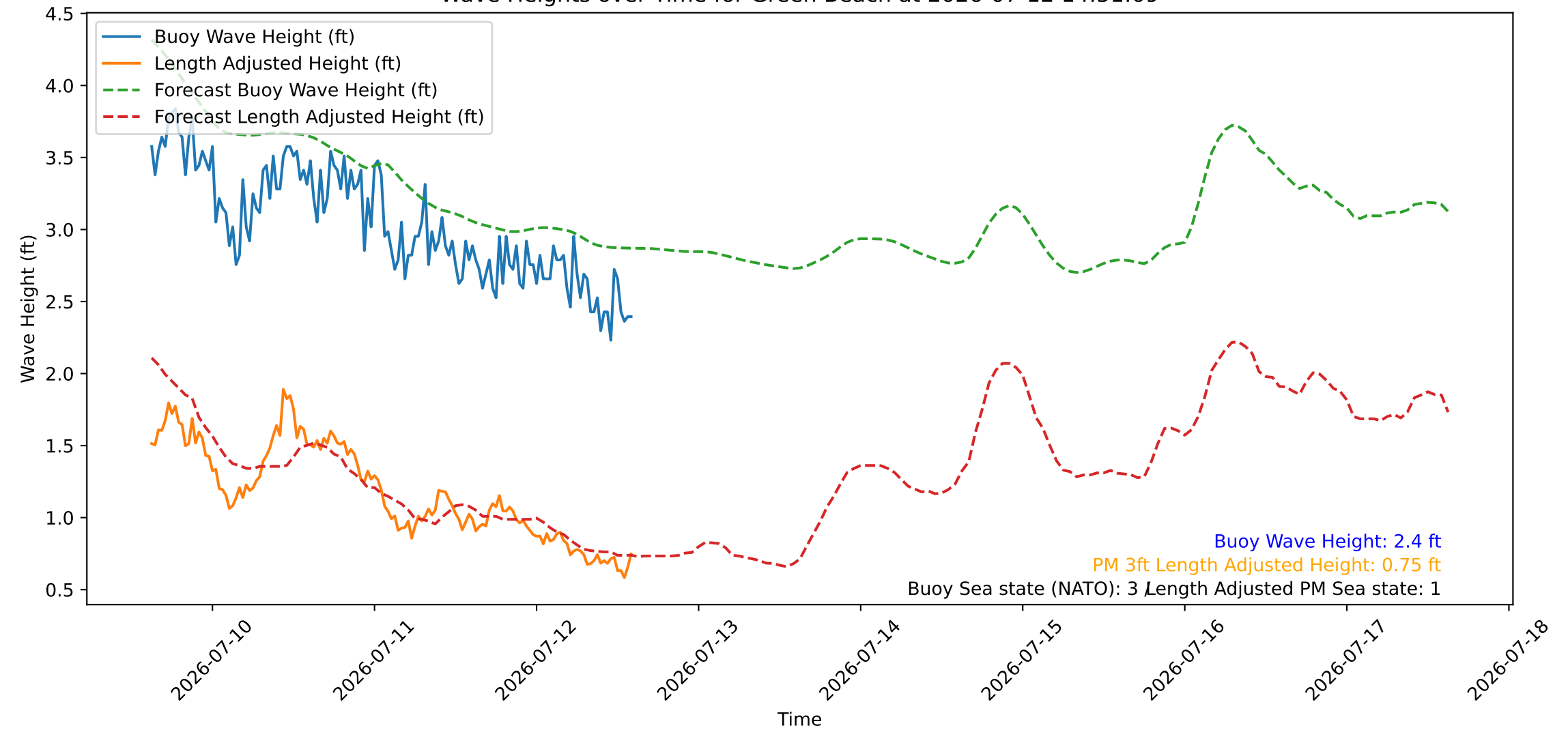
Wave Heights over Time for Green Beach at 2026-07-12 14:51:09
