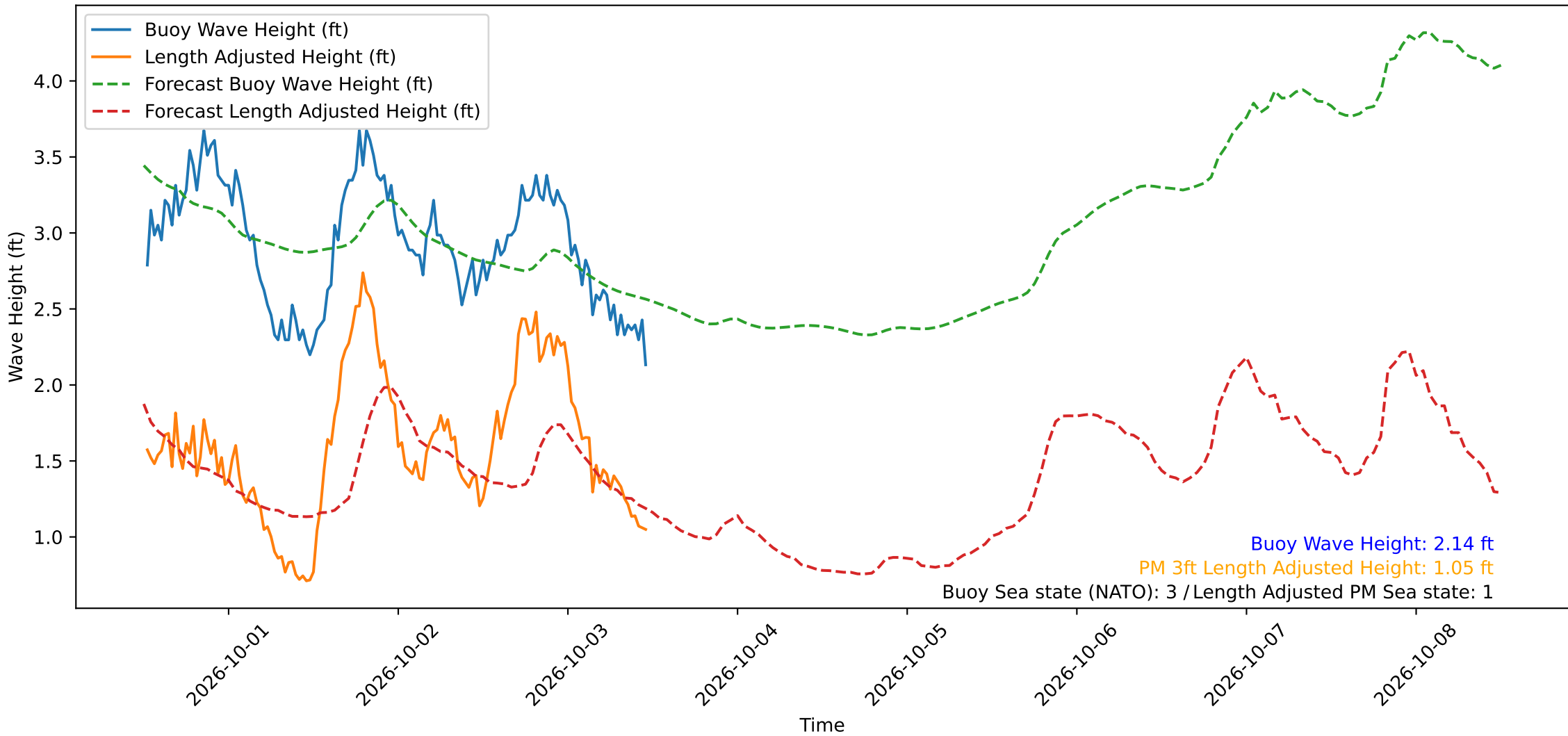
Wave Heights over Time for Green Beach at 2026-10-03 12:01:10
