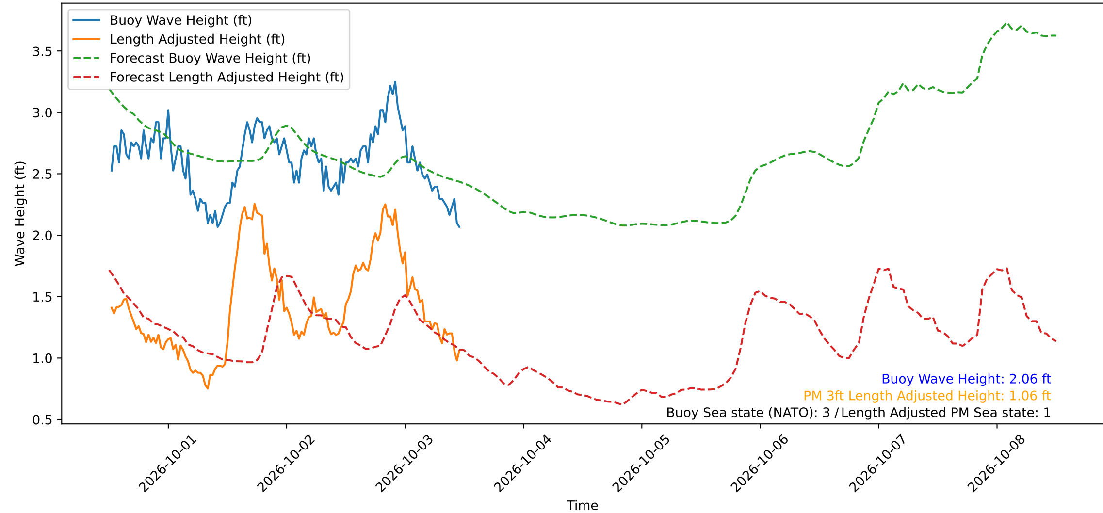
Wave Heights over Time for Red Beach at 2026-10-03 12:00:48
