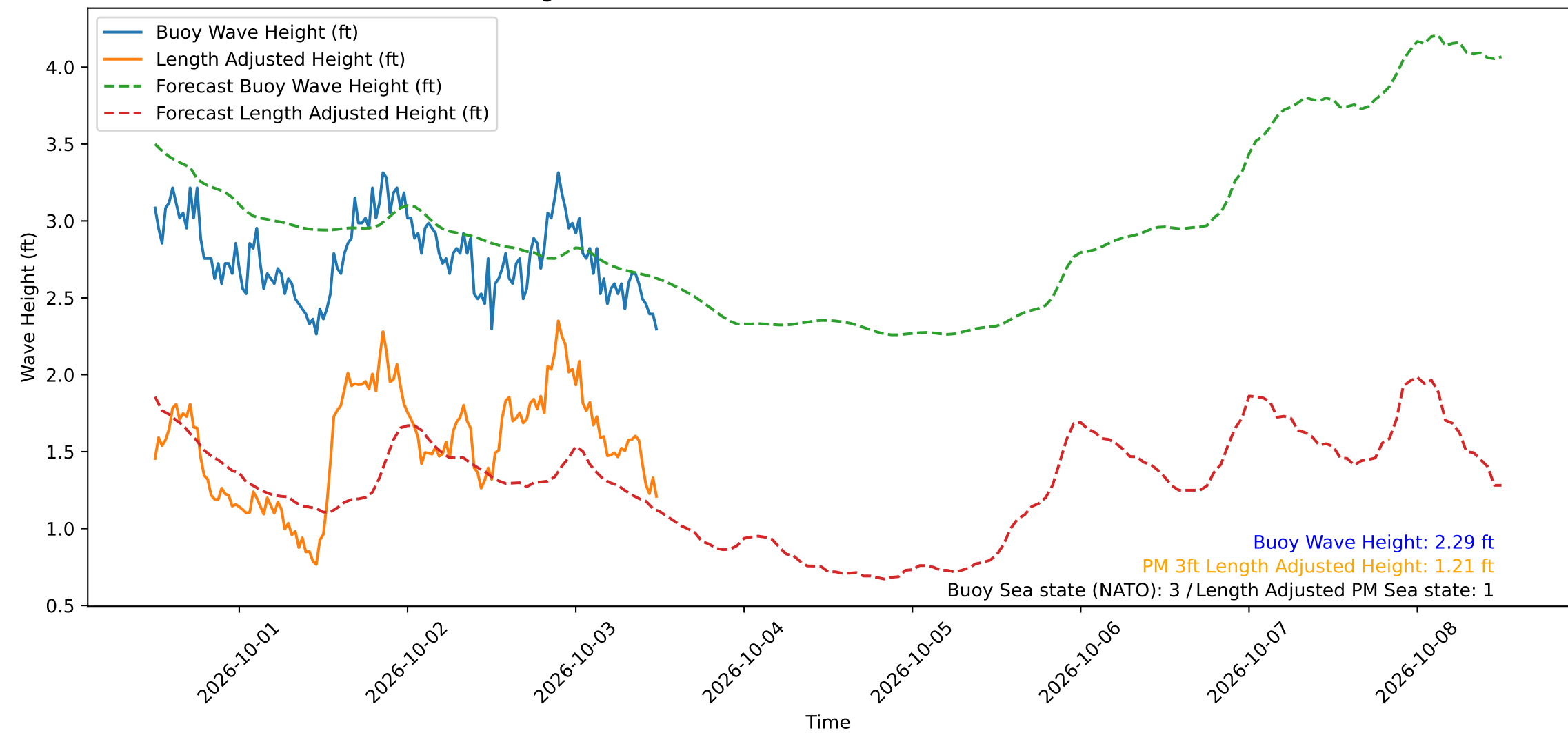
Wave Heights over Time for Oceanside Harbor at 2026-10-03 12:00:29
