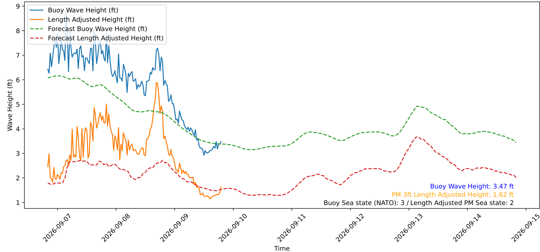
Wave Heights over Time for Green Beach at 2026-09-09 19:51:13
