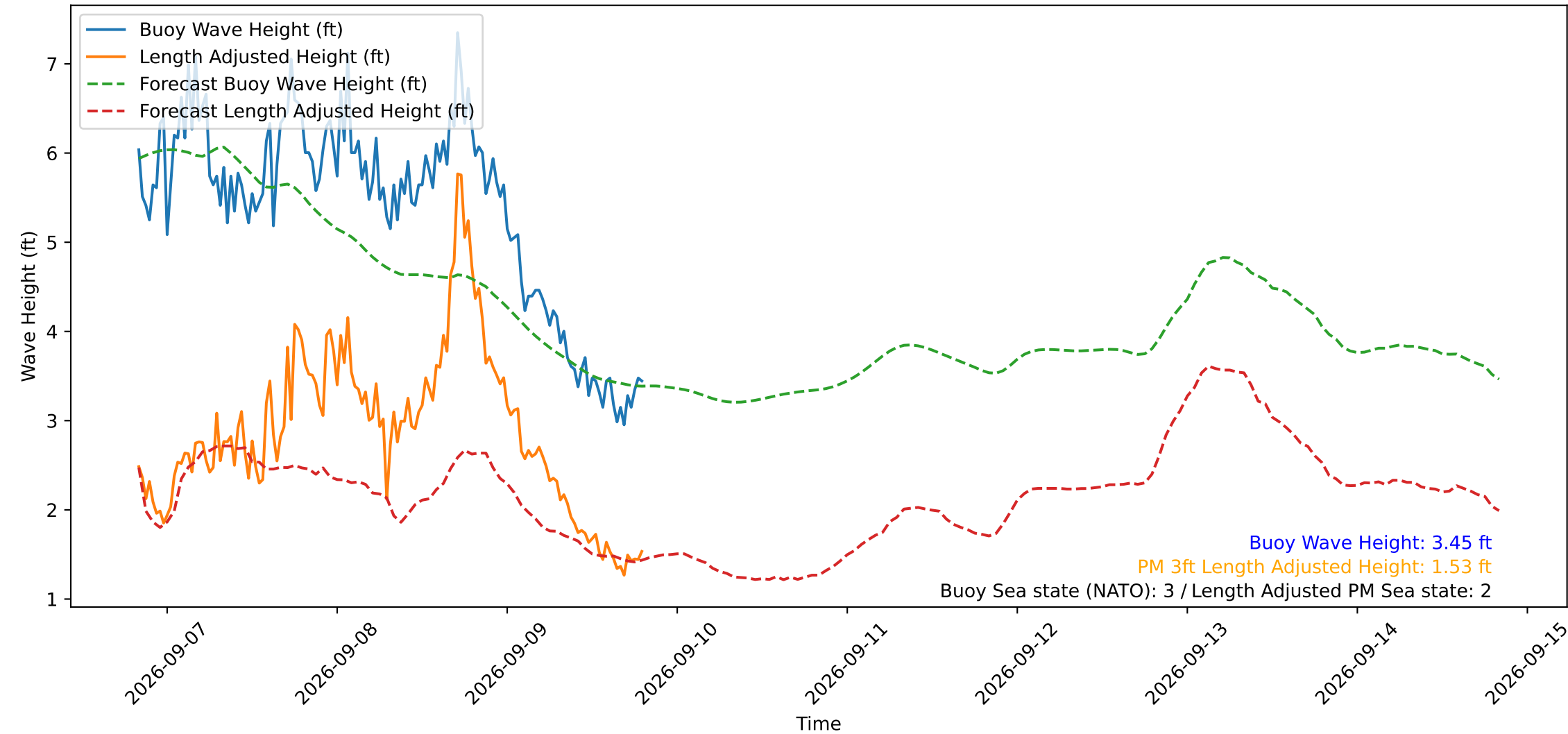
Wave Heights over Time for Oceanside Harbor at 2026-09-09 19:50:29
